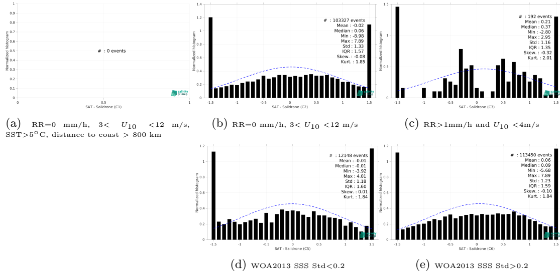
Figure 15: Normalized histogram of \Delta SSS (SMAP SSS L2 v5.3 (RSS) - Saldrone) for 5 different subdatasets corresponding to: RR=0 mm/h, 3 < U_{10} < 12 m/s, SST > 5°C, distance to coast > 800 km (a), RR=0 mm/h, 3 < U_{10} < 12 m/s (b), RR > 1mm/h and U_{10} < 4 m/s (c), WOA2013 SSS Std < 0.2 (d), WOA2013 SSS Std > 0.2 (e).
