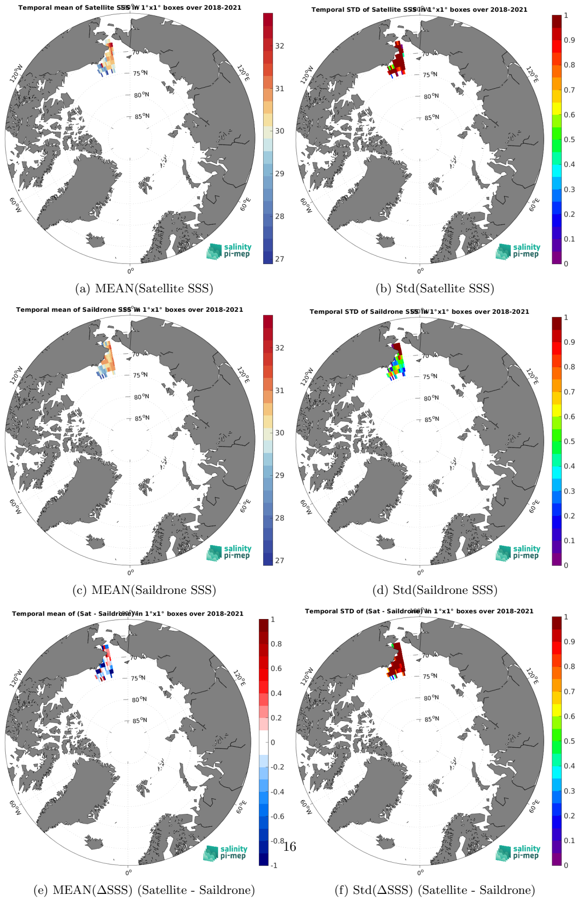
Figure 7: Temporal mean (left) and Std (right) of SSS from SMAP SSS L2 v5.3 (RSS) (top), Saildrone (middle), and of \Delta SSS (Satellite - Saildrone). Only match-up pairs are used to generate these maps.
