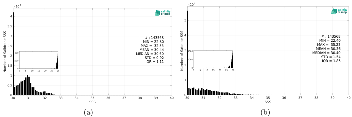
Figure 3: Histograms of SSS from Saildrone (a) and SMAP SSS L2 v5.3 (RSS) (b) considering all match-up pairs per bins of 0.1 over the Arctic Ocean Pi-MEP region and for the full satellite product period.
