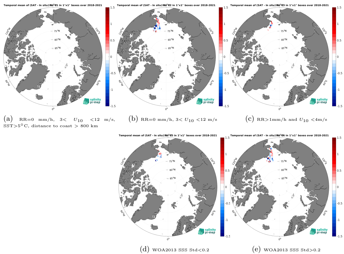
Figure 14: Temporal mean gridded over spatial boxes of size 1^\circ \times 1^\circ of \Delta SSS (SMAP SSS L2 v5.3 (RSS) - Saldrone) for 5 different subdatasets corresponding to:RR=0 mm/h, 3 < U_{10} < 12 m/s, SST>5°C, distance to coast > 800 km (a), RR=0 mm/h, 3 < U_{10} < 12 m/s (b), RR>1mm/h and U_{10} < 4 m/s (c), WOA2013 SSS Std<0.2 (d), WOA2013 SSS Std>0.2 (e).
