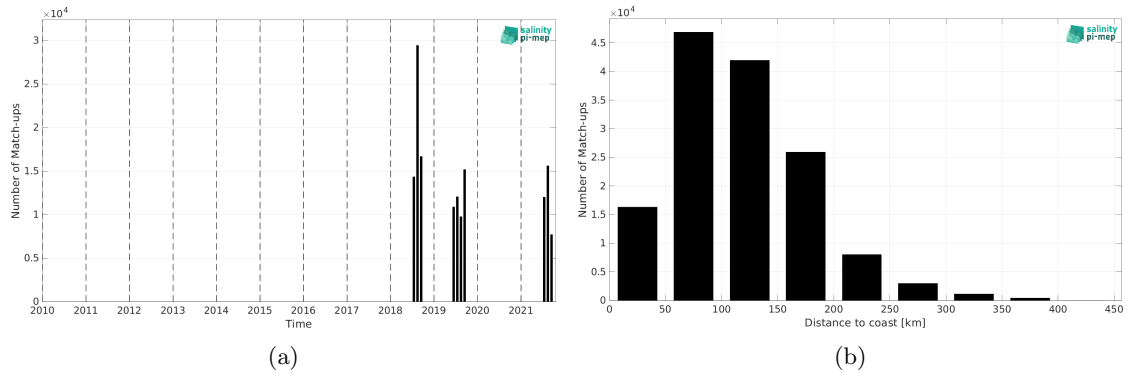
Figure 2: Number of match-ups between Saildrone and SMAP SSS L2 v5.3 (RSS) SSS as a function of time (a) and as function of the distance to coast (b) over the Arctic Ocean Pi-MEP region and for the full satellite product period.
