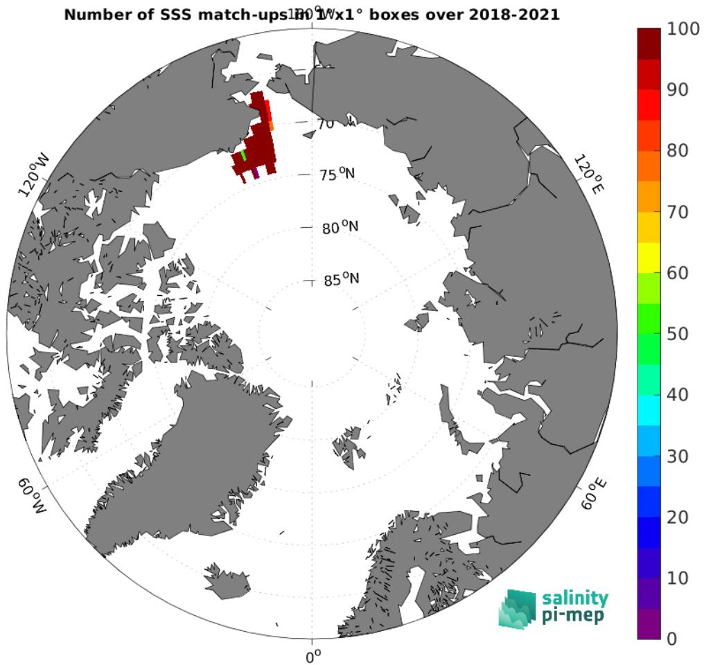
Figure 5: Number of SSS match-ups between Sailldrone SSS and the SMAP SSS L2 v5.3 (RSS) SSS product for the Arctic Ocean Pi-MEP region over 1^\circ \times 1^\circ boxes and for the full satellite product period.
