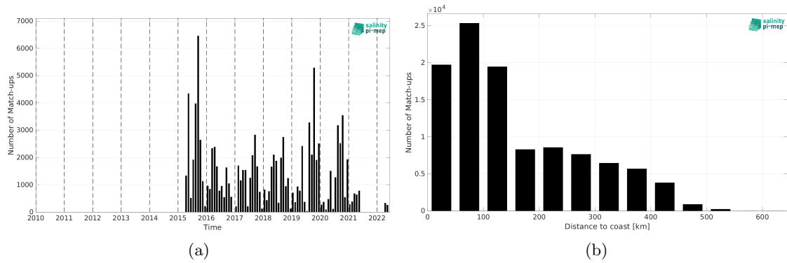
Figure 2: Number of match-ups between ICES and SMAP SSS L2 v5.3 (RSS) SSS as a function of time (a) and as function of the distance to coast (b) over the Arctic Ocean Pi-MEP region and for the full satellite product period.
