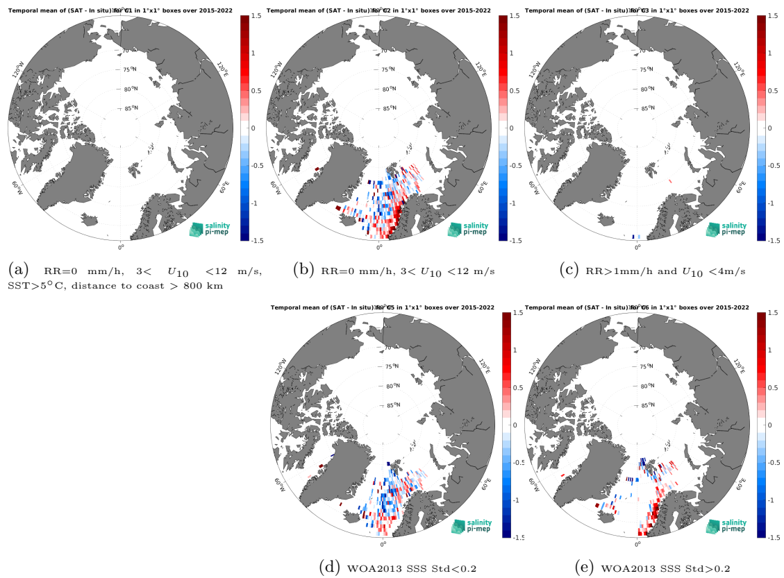
Figure 14: Temporal mean gridded over spatial boxes of size 1^\circ \times 1^\circ of \Delta SSS (SMAP SSS L2 v5.3 (RSS) - ICES) for 5 different subdatasets corresponding to:RR=0 mm/h, 3 < U_{10} < 12 m/s, SST>5°C, distance to coast > 800 km (a), RR=0 mm/h, 3 < U_{10} < 12 m/s (b), RR>1mm/h and U_{10} < 4 m/s (c), WOA2013 SSS Std<0.2 (d), WOA2013 SSS Std>0.2 (e).
