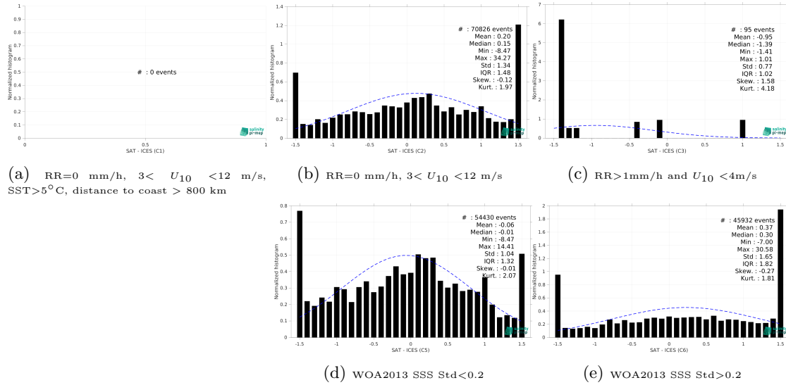
Figure 15: Normalized histogram of \Delta SSS (SMAP SSS L2 v5.3 (RSS) - ICES) for 5 different subdatasets corresponding to: RR=0 mm/h, 3 < U_{10} < 12 m/s, SST > 5°C, distance to coast > 800 km (a), RR=0 mm/h, 3 < U_{10} < 12 m/s (b), RR > 1mm/h and U_{10} < 4 m/s (c), WOA2013 SSS Std < 0.2 (d), WOA2013 SSS Std > 0.2 (e).
