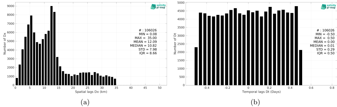
Figure 6: Histograms of the spatial (a) and temporal (b) lags between the location/time of the ICES measurement and the date of the corresponding SMAP SSS L2 v5.3 (RSS) SSS pixel.
