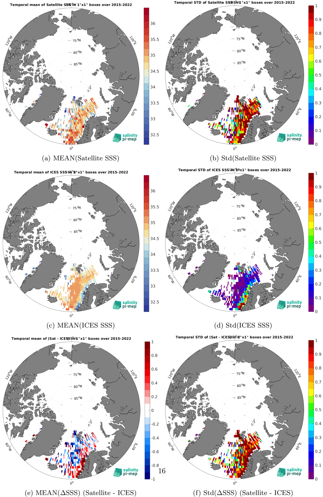
Figure 7: Temporal mean (left) and Std (right) of SSS from SMAP SSS L2 v5.3 (RSS) (top), ICES (middle), and of \Delta SSS (Satellite - ICES). Only match-up pairs are used to generate these maps.
