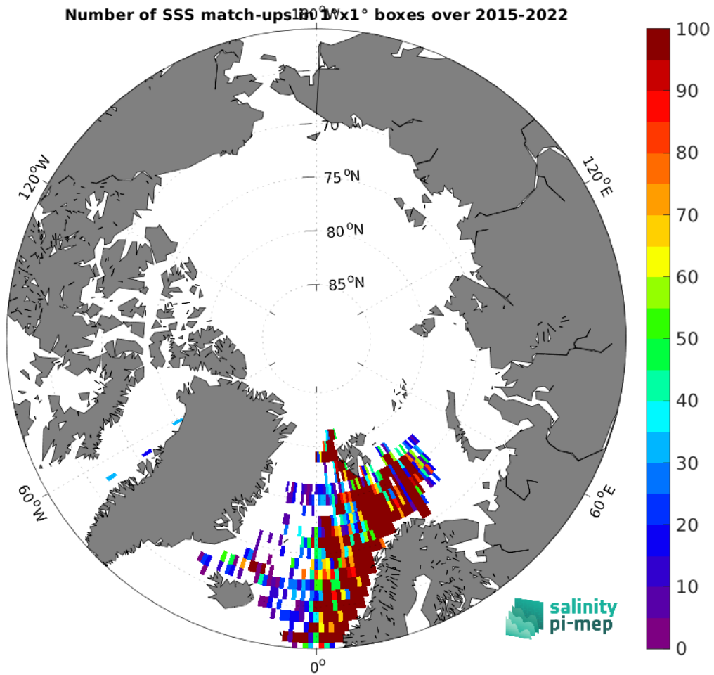
Figure 5: Number of SSS match-ups between ICES SSS and the SMAP SSS L2 v5.3 (RSS) SSS product for the Arctic Ocean Pi-MEP region over 1^\circ \times 1^\circ boxes and for the full satellite product period.
