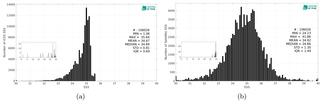
Figure 3: Histograms of SSS from ICES (a) and SMAP SSS L2 v5.3 (RSS) (b) considering all match-up pairs per bins of 0.1 over the Arctic Ocean Pi-MEP region and for the full satellite product period.
