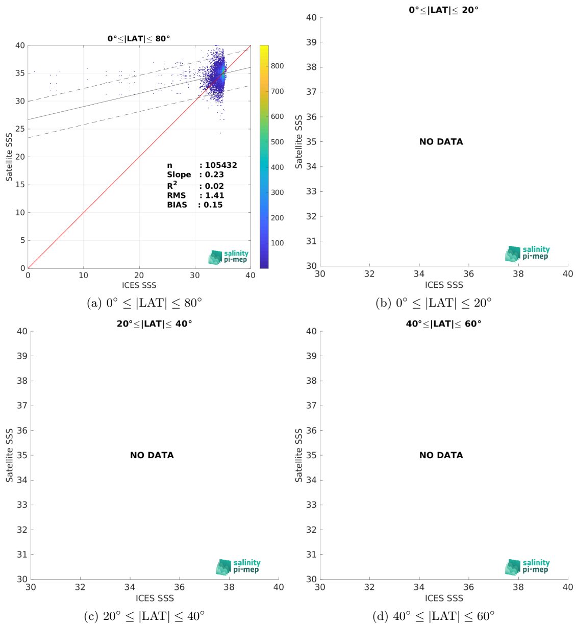
Figure 10: Contour maps of the concentration of SMAP SSS L2 v5.3 (RSS) SSS (y-axis) versus ICES SSS (x-axis) at match-up pairs for different latitude bands. For each plot, the red line shows x=y . The black thin and dashed lines indicate a linear fit through the data cloud and the \pm 95\% confidence levels, respectively. The number match-up pairs n , the slope and R^2 coefficient of the linear fit, the root mean square (RMS) and the mean bias between satellite and in situ data are indicated for each latitude band in each plots.
