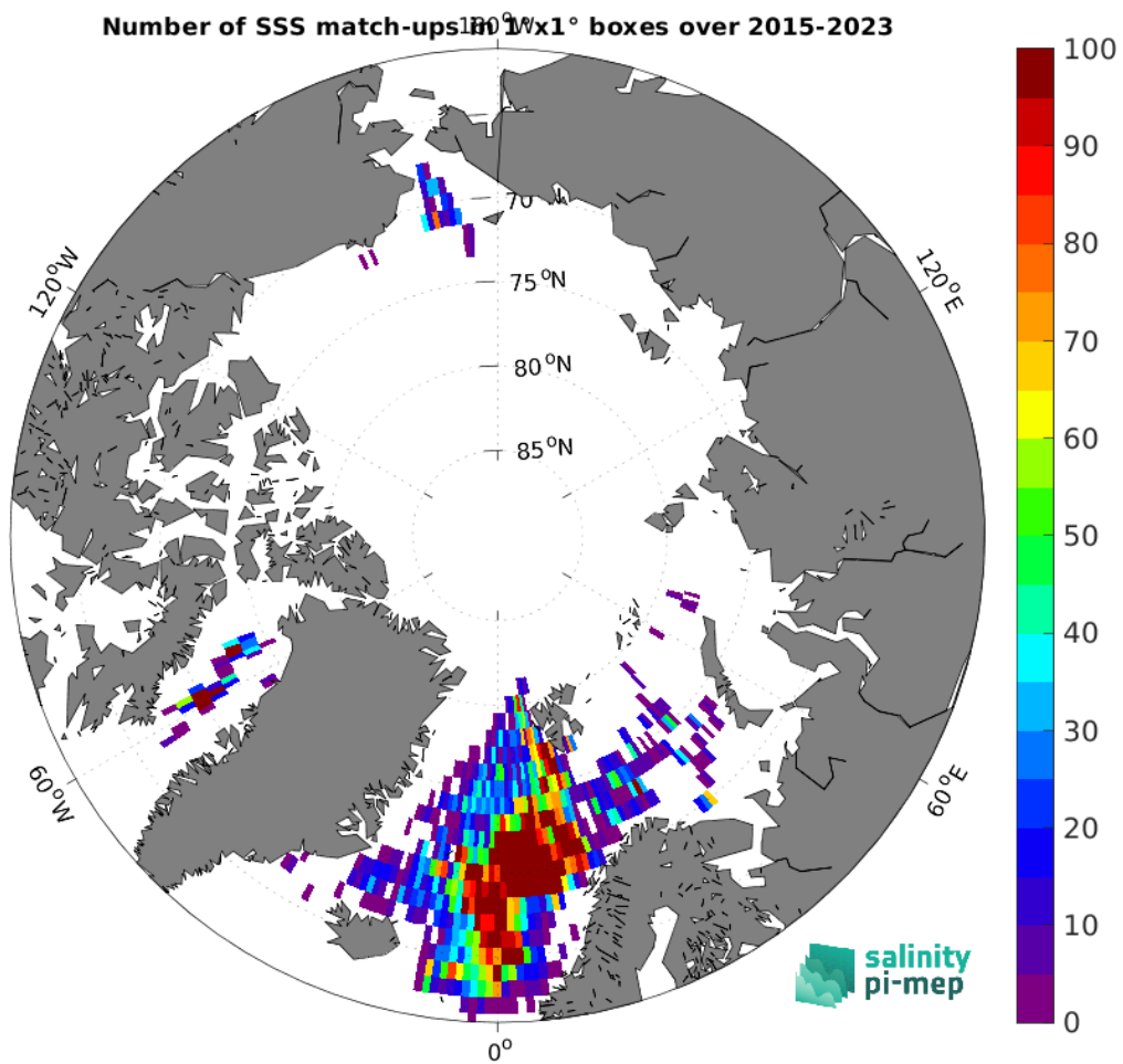
Figure 5: Number of SSS match-ups between Argo SSS and the SMAP SSS L2 v5.3 (RSS) SSS product for the Arctic Ocean Pi-MEP region over 1^\circ \times 1^\circ boxes and for the full satellite product period.
