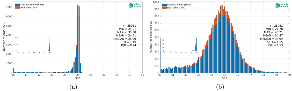
Figure 3: Histograms of SSS from Argo (a) and SMAP SSS L2 v5.3 (RSS) (b) considering all match-up pairs per bins of 0.1 over the Arctic Ocean Pi-MEP region and for the full satellite product period.
