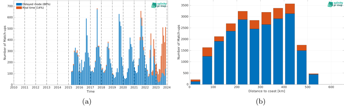
Figure 2: Number of match-ups between Argo and SMAP SSS L2 v5.3 (RSS) SSS as a function of time (a) and as function of the distance to coast (b) over the Arctic Ocean Pi-MEP region and for the full satellite product period.
