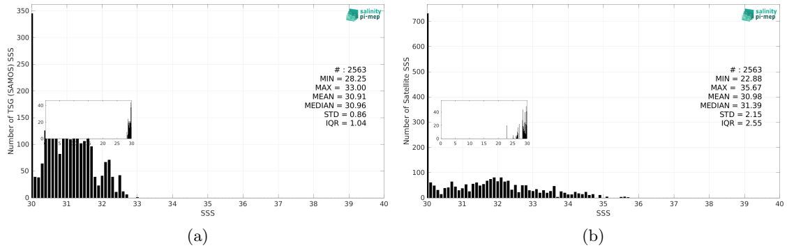
Figure 3: Histograms of SSS from TSG (SAMOS) (a) and SMAP SSS L2 v5.3 - 40 km (RSS) (b) considering all match-up pairs per bins of 0.1 over the Arctic Ocean Pi-MEP region and for the full satellite product period.
