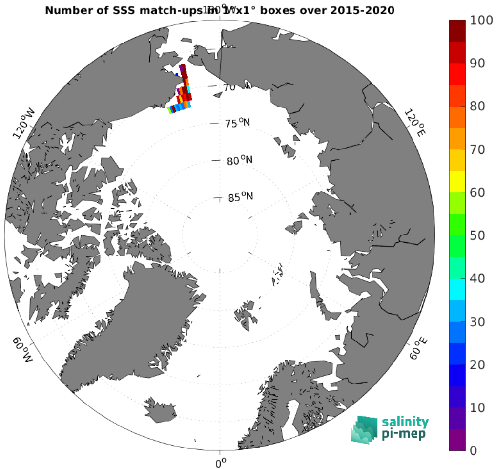
Figure 5: Number of SSS match-ups between TSG (SAMOS) SSS and the SMAP SSS L2 v5.3 - 40 km (RSS) SSS product for the Arctic Ocean Pi-MEP region over 1^\circ \times 1^\circ boxes and for the full satellite product period.
