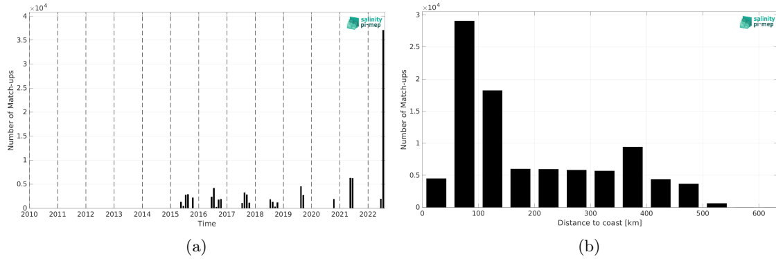
Figure 2: Number of match-ups between TSG (Polarstern) and SMAP SSS L2 v5.3 - 40 km (RSS) SSS as a function of time (a) and as function of the distance to coast (b) over the Arctic Ocean Pi-MEP region and for the full satellite product period.
