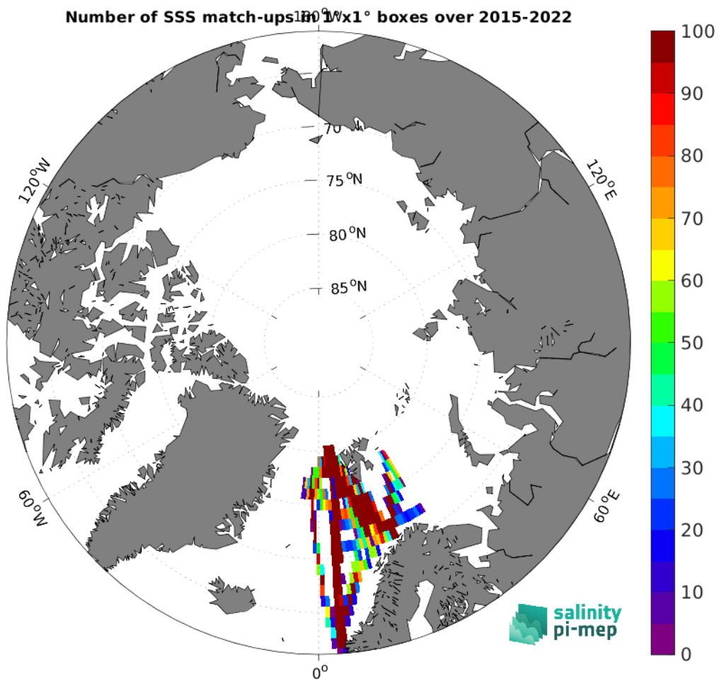
Figure 5: Number of SSS match-ups between TSG (Polarstern) SSS and the SMAP SSS L2 v5.3 - 40 km (RSS) SSS product for the Arctic Ocean Pi-MEP region over 1^\circ \times 1^\circ boxes and for the full satellite product period.
