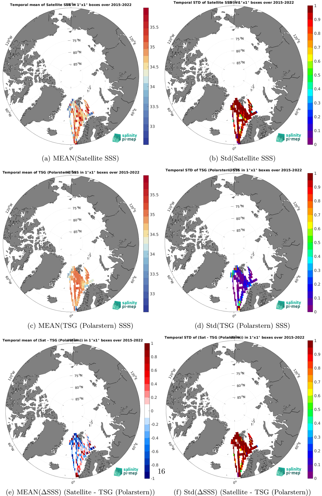
Figure 7: Temporal mean (left) and Std (right) of SSS from SMAP SSS L2 v5.3 - 40 km (RSS) (top), TSG (Polarstern) (middle), and of \Delta SSS (Satellite - TSG (Polarstern)). Only match-up pairs are used to generate these maps.
