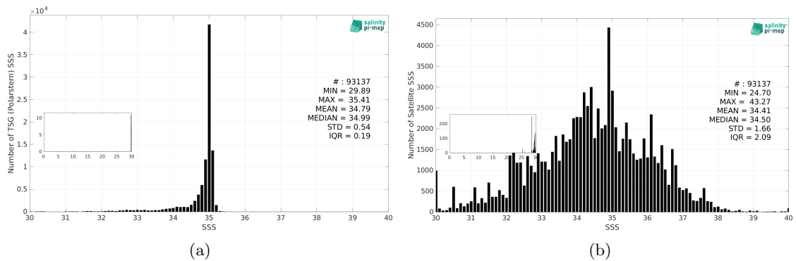
Figure 3: Histograms of SSS from TSG (Polarstern) (a) and SMAP SSS L2 v5.3 - 40 km (RSS) (b) considering all match-up pairs per bins of 0.1 over the Arctic Ocean Pi-MEP region and for the full satellite product period.
