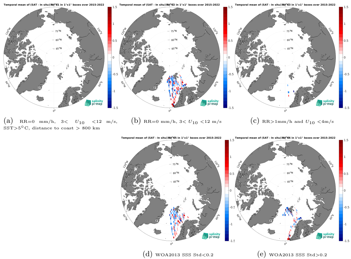
Figure 14: Temporal mean gridded over spatial boxes of size 1^\circ \times 1^\circ of \Delta SSS (SMAP SSS L2 v5.3 - 40 km (RSS) - TSG (Polarstern)) for 5 different subdatasets corresponding to:RR=0 mm/h, 3 < U_{10} < 12 m/s, SST>5°C, distance to coast > 800 km (a), RR=0 mm/h, 3 < U_{10} < 12 m/s (b), RR>1mm/h and U_{10} < 4 m/s (c), WOA2013 SSS Std<0.2 (d), WOA2013 SSS Std>0.2 (e).
