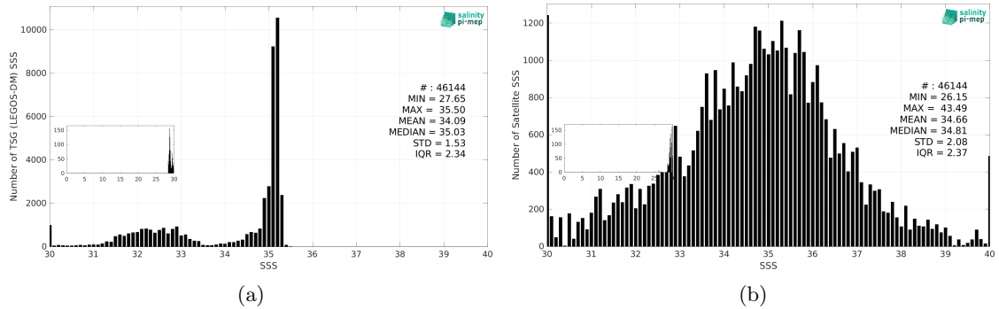
Figure 3: Histograms of SSS from TSG (LEGOS-DM) (a) and SMAP SSS L2 v5.3 - 40 km (RSS) (b) considering all match-up pairs per bins of 0.1 over the Arctic Ocean Pi-MEP region and for the full satellite product period.
