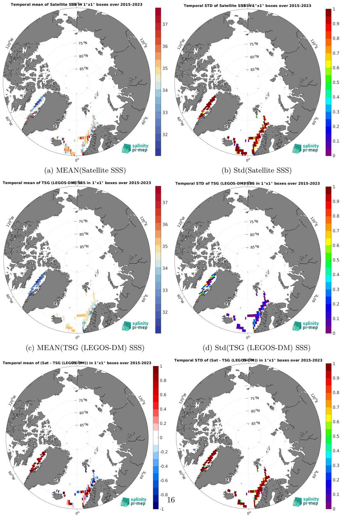
Figure 7: Temporal mean (left) and Std (right) of SSS from SMAP SSS L2 v5.3 - 40 km (RSS) (top), TSG (LEGOS-DM) (middle), and of \Delta SSS (Satellite - TSG (LEGOS-DM)). Only match-up pairs are used to generate these maps.
