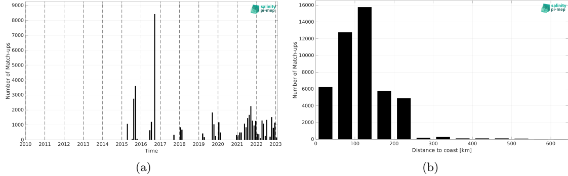
Figure 2: Number of match-ups between TSG (LEGOS-DM) and SMAP SSS L2 v5.3 - 40 km (RSS) SSS as a function of time (a) and as function of the distance to coast (b) over the Arctic Ocean Pi-MEP region and for the full satellite product period.
