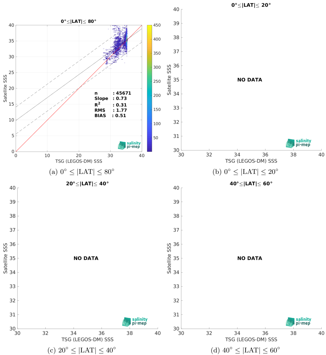
Figure 10: Contour maps of the concentration of SMAP SSS L2 v5.3 - 40 km (RSS) SSS (y-axis) versus TSG (LEGOS-DM) SSS (x-axis) at match-up pairs for different latitude bands. For each plot, the red line shows x=y . The black thin and dashed lines indicate a linear fit through the data cloud and the \pm 95\% confidence levels, respectively. The number match-up pairs n , the slope and R^2 coefficient of the linear fit, the root mean square (RMS) and the mean bias between satellite and in situ data are indicated for each latitude band in each plots.
