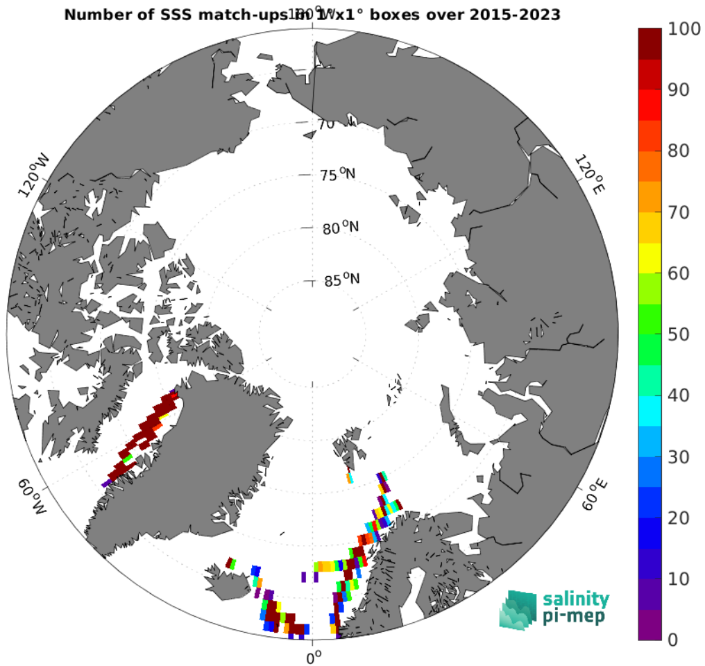
Figure 5: Number of SSS match-ups between TSG (LEGOS-DM) SSS and the SMAP SSS L2 v5.3 - 40 km (RSS) SSS product for the Arctic Ocean Pi-MEP region over 1^\circ \times 1^\circ boxes and for the full satellite product period.
