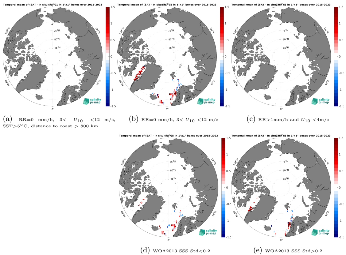
Figure 14: Temporal mean gridded over spatial boxes of size 1^\circ \times 1^\circ of \Delta SSS (SMAP SSS L2 v5.3 - 40 km (RSS) - TSG (LEGOS-DM)) for 5 different subdatasets corresponding to: RR=0 mm/h, 3 < U_{10} < 12 m/s, SST > 5°C, distance to coast > 800 km (a), RR=0 mm/h, 3 < U_{10} < 12 m/s (b), RR > 1mm/h and U_{10} < 4 m/s (c), WOA2013 SSS Std < 0.2 (d), WOA2013 SSS Std > 0.2 (e).
