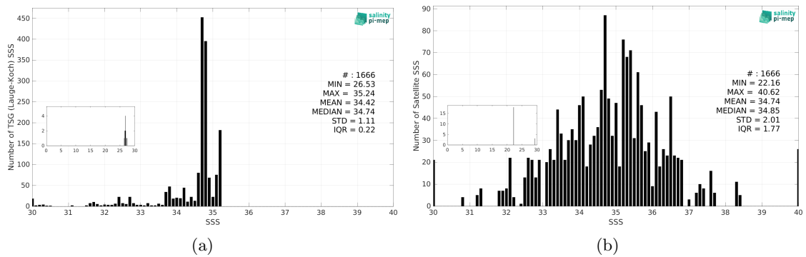
Figure 3: Histograms of SSS from TSG (Lauge-Koch) (a) and SMAP SSS L2 v5.3 - 40 km (RSS) (b) considering all match-up pairs per bins of 0.1 over the Arctic Ocean Pi-MEP region and for the full satellite product period.
