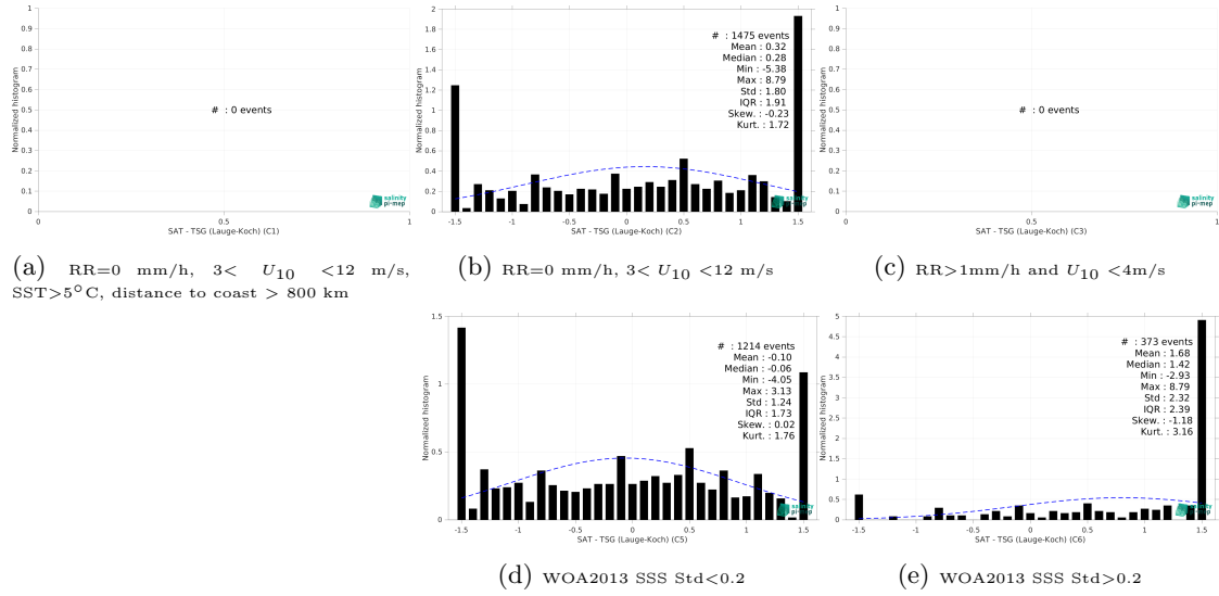
Figure 15: Normalized histogram of \Delta SSS (SMAP SSS L2 v5.3 - 40 km (RSS) - TSG (Lauge-Koch)) for 5 different subdatasets corresponding to: RR=0 mm/h, 3 < U_{10} < 12 m/s, SST > 5°C, distance to coast > 800 km (a), RR=0 mm/h, 3 < U_{10} < 12 m/s (b), RR > 1mm/h and U_{10} < 4 m/s (c), WOA2013 SSS Std < 0.2 (d), WOA2013 SSS Std > 0.2 (e).
