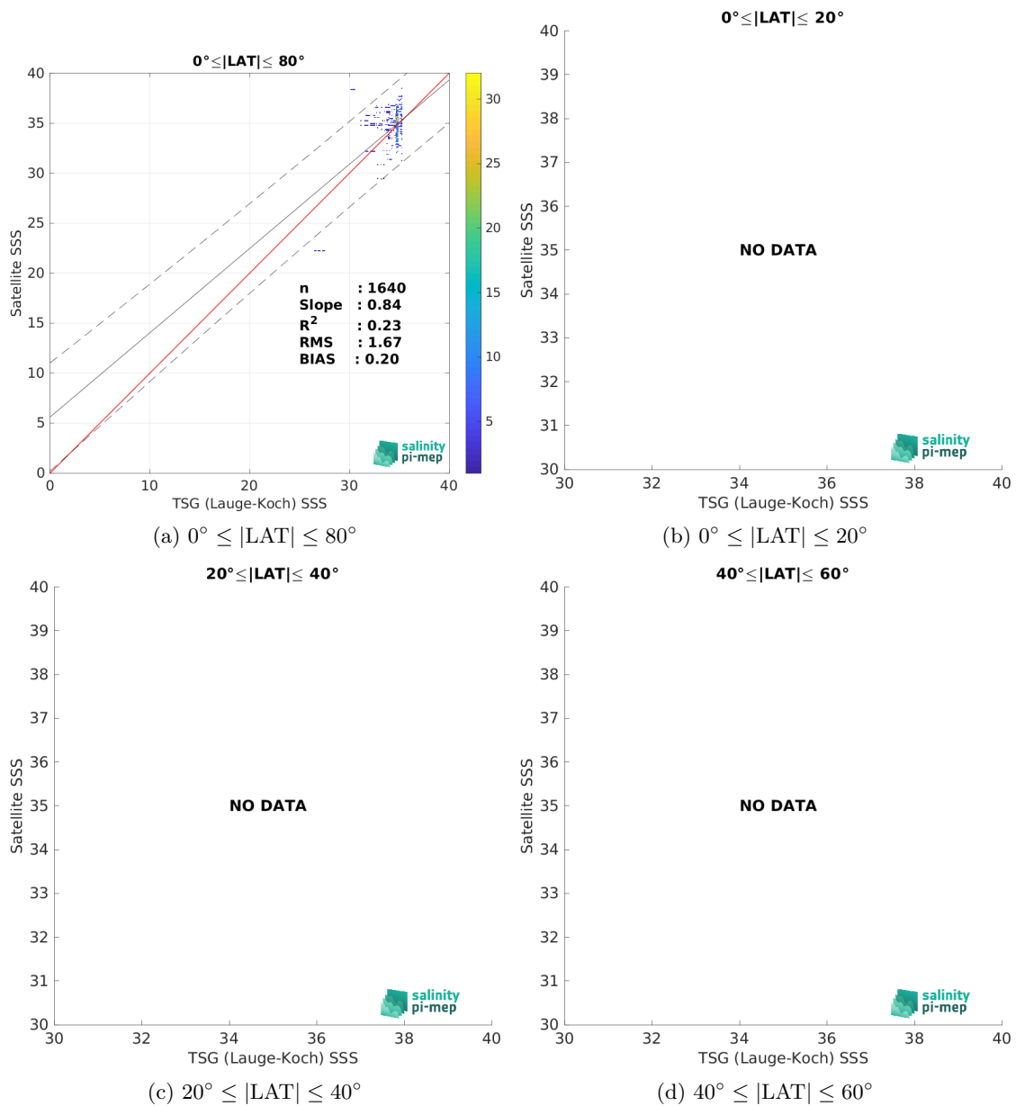
Figure 10: Contour maps of the concentration of SMAP SSS L2 v5.3 - 40 km (RSS) SSS (y-axis) versus TSG (Lauge-Koch) SSS (x-axis) at match-up pairs for different latitude bands. For each plot, the red line shows x=y . The black thin and dashed lines indicate a linear fit through the data cloud and the \pm 95\% confidence levels, respectively. The number match-up pairs n , the slope and R^2 coefficient of the linear fit, the root mean square (RMS) and the mean bias between satellite and in situ data are indicated for each latitude band in each plots.
