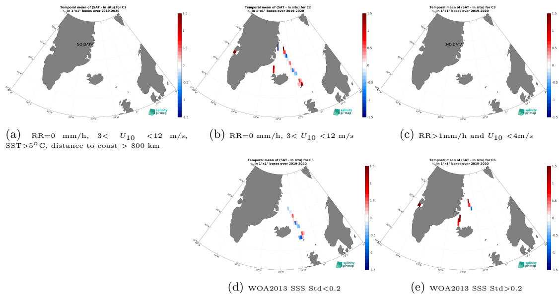
Figure 14: Temporal mean gridded over spatial boxes of size 1^\circ \times 1^\circ of \Delta SSS (SMAP SSS L2 v5.3 - 40 km (RSS) - TSG (Lauge-Koch)) for 5 different subdatasets corresponding to:RR=0 mm/h, 3 < U_{10} < 12 m/s, SST > 5^\circ\text{C} , distance to coast > 800 km (a), RR=0 mm/h, 3 < U_{10} < 12 m/s (b), RR > 1 mm/h and U_{10} < 4 m/s (c), WOA2013 SSS Std < 0.2 (d), WOA2013 SSS Std > 0.2 (e).
