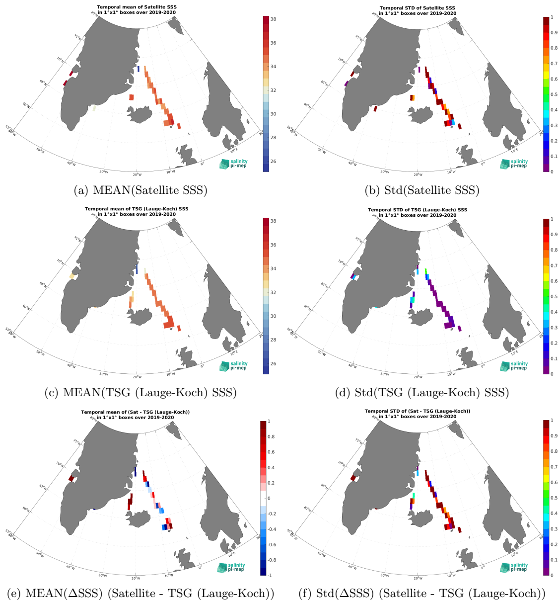
Figure 7: Temporal mean (left) and Std (right) of SSS from SMAP SSS L2 v5.3 - 40 km (RSS) (top), TSG (Lauge-Koch) (middle), and of \Delta SSS (Satellite - TSG (Lauge-Koch)). Only match-up pairs are used to generate these maps.
