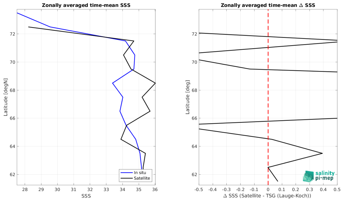
Figure 9: Left panel: Zonal mean SSS from SMAP SSS L2 v5.3 - 40 km (RSS) satellite product (black) and from TSG (Lauge-Koch) (blue). Right panel: Zonal mean of \Delta SSS (Satellite - TSG (Lauge-Koch)) for all the collected Pi-MEP match-up pairs estimated over the full satellite product period.
