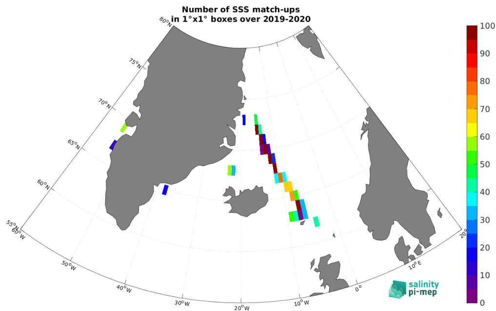
Figure 5: Number of SSS match-ups between TSG (Lauge-Koch) SSS and the SMAP SSS L2 v5.3 - 40 km (RSS) SSS product for the Arctic Ocean Pi-MEP region over 1^\circ \times 1^\circ boxes and for the full satellite product period.
