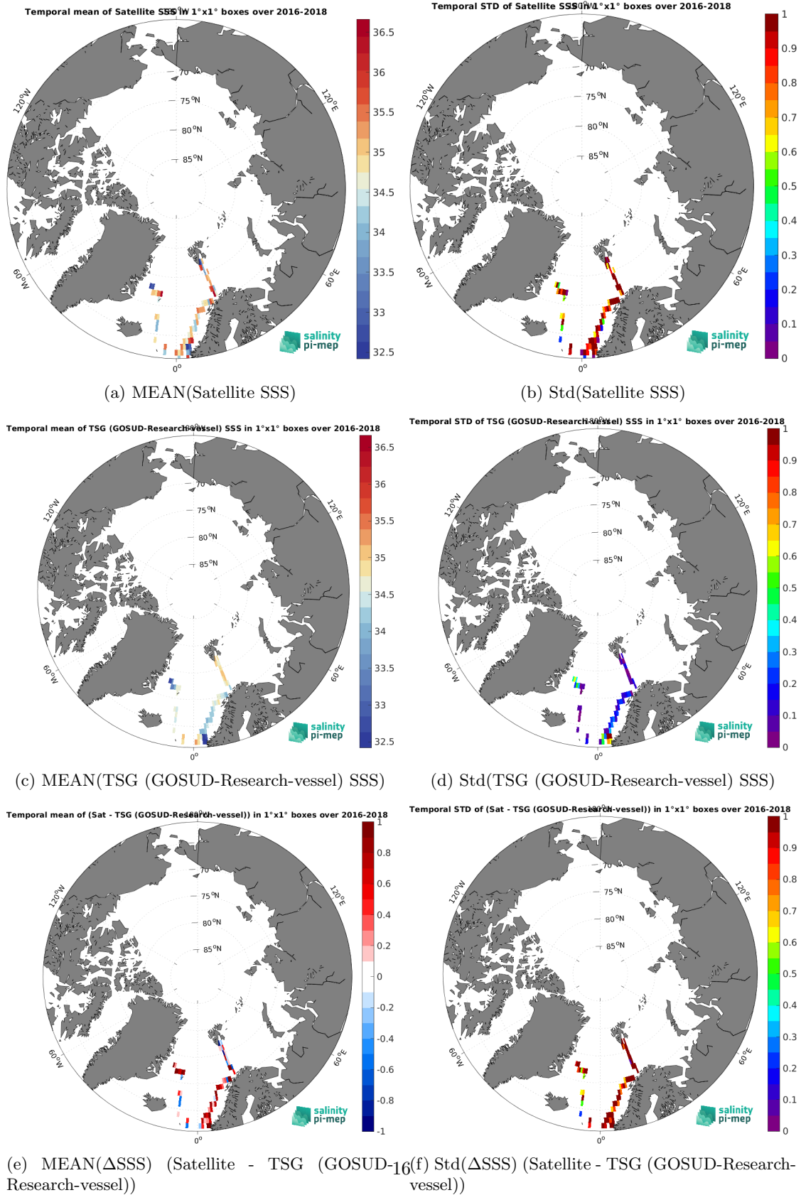
Figure 7: Temporal mean (left) and Std (right) of SSS from SMAP SSS L2 v5.3 - 40 km (RSS) (top), TSG (GOSUD-Research-vessel) (middle), and of \Delta SSS (Satellite - TSG (GOSUD-Research-vessel)). Only match-up pairs are used to generate these maps.
