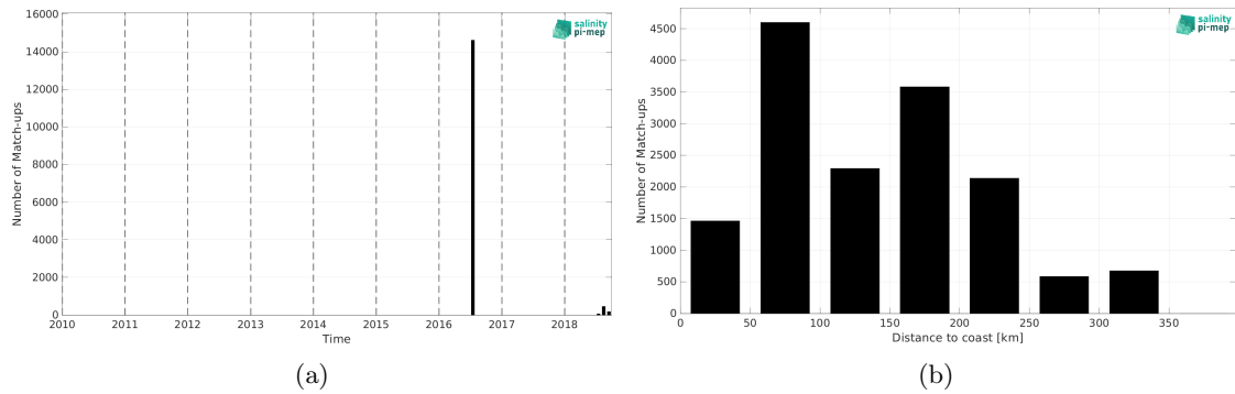
Figure 2: Number of match-ups between TSG (GOSUD-Research-vessel) and SMAP SSS L2 v5.3 - 40 km (RSS) SSS as a function of time (a) and as function of the distance to coast (b) over the Arctic Ocean Pi-MEP region and for the full satellite product period.
