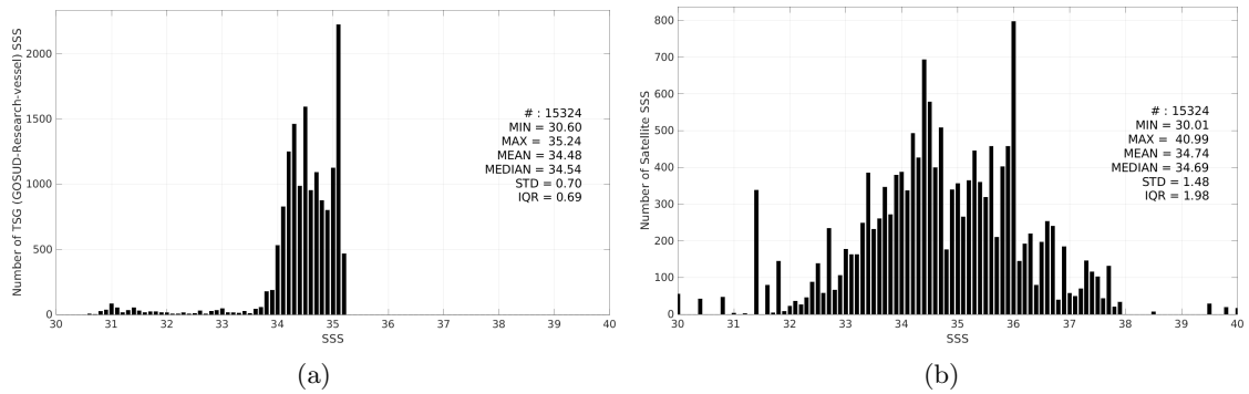
Figure 3: Histograms of SSS from TSG (GOSUD-Research-vessel) (a) and SMAP SSS L2 v5.3 - 40 km (RSS) (b) considering all match-up pairs per bins of 0.1 over the Arctic Ocean Pi-MEP region and for the full satellite product period.
