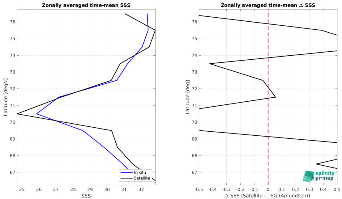
Figure 9: Left panel: Zonal mean SSS from SMAP SSS L2 v5.3 - 40 km (RSS) satellite product (black) and from TSG (Amundsen) (blue). Right panel: Zonal mean of \Delta SSS (Satellite - TSG (Amundsen)) for all the collected Pi-MEP match-up pairs estimated over the full satellite product period.
