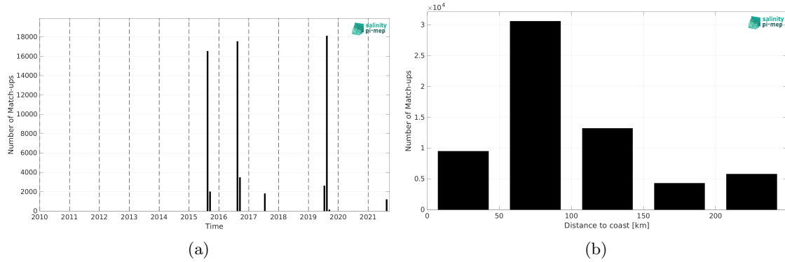
Figure 2: Number of match-ups between TSG (Amundsen) and SMAP SSS L2 v5.3 - 40 km (RSS) SSS as a function of time (a) and as function of the distance to coast (b) over the Arctic Ocean Pi-MEP region and for the full satellite product period.
