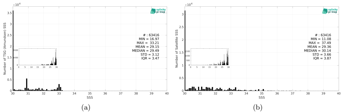
Figure 3: Histograms of SSS from TSG (Amundsen) (a) and SMAP SSS L2 v5.3 - 40 km (RSS) (b) considering all match-up pairs per bins of 0.1 over the Arctic Ocean Pi-MEP region and for the full satellite product period.
