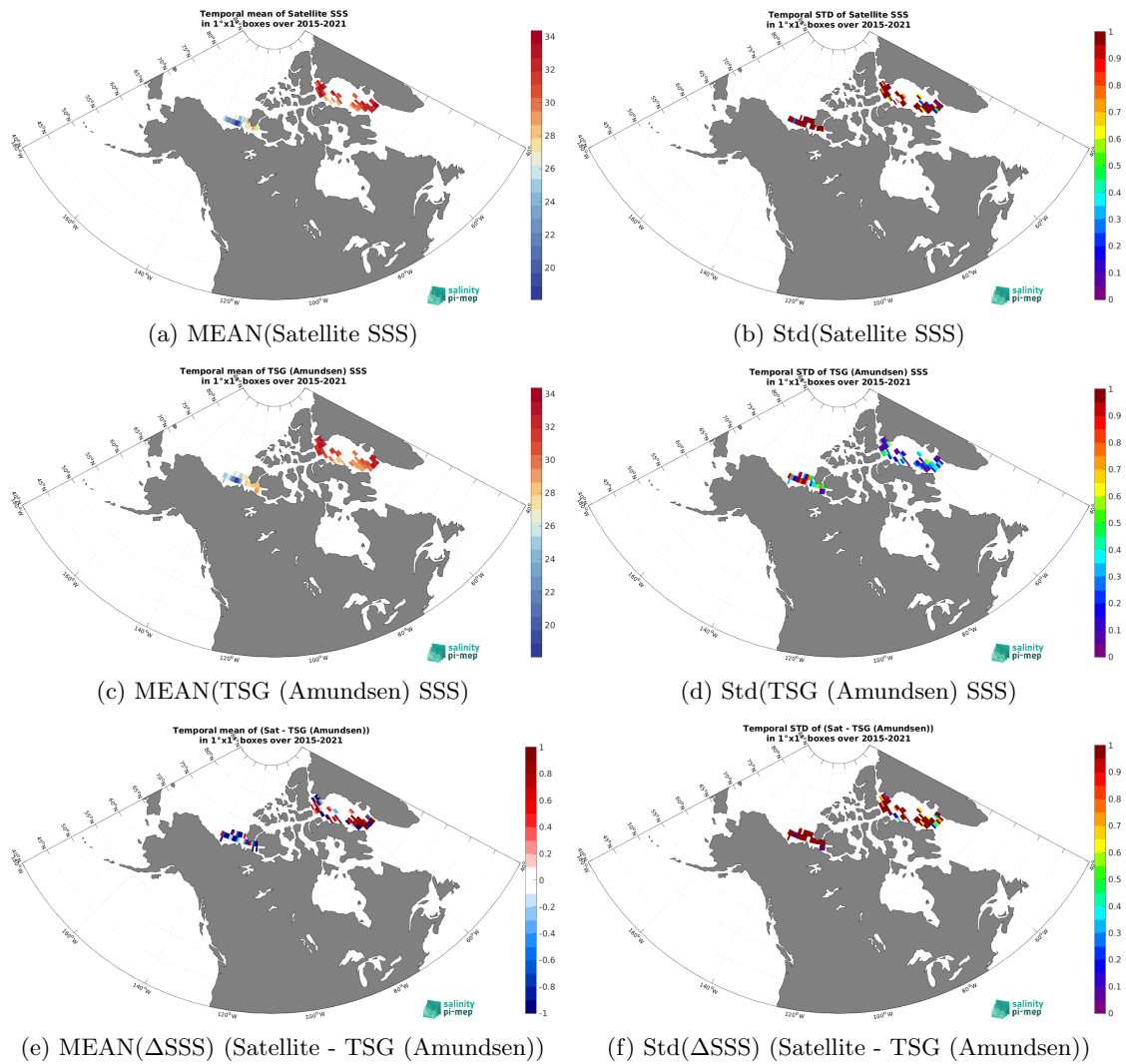
Figure 7: Temporal mean (left) and Std (right) of SSS from SMAP SSS L2 v5.3 - 40 km (RSS) (top), TSG (Amundsen) (middle), and of \Delta SSS (Satellite - TSG (Amundsen)). Only match-up pairs are used to generate these maps.
