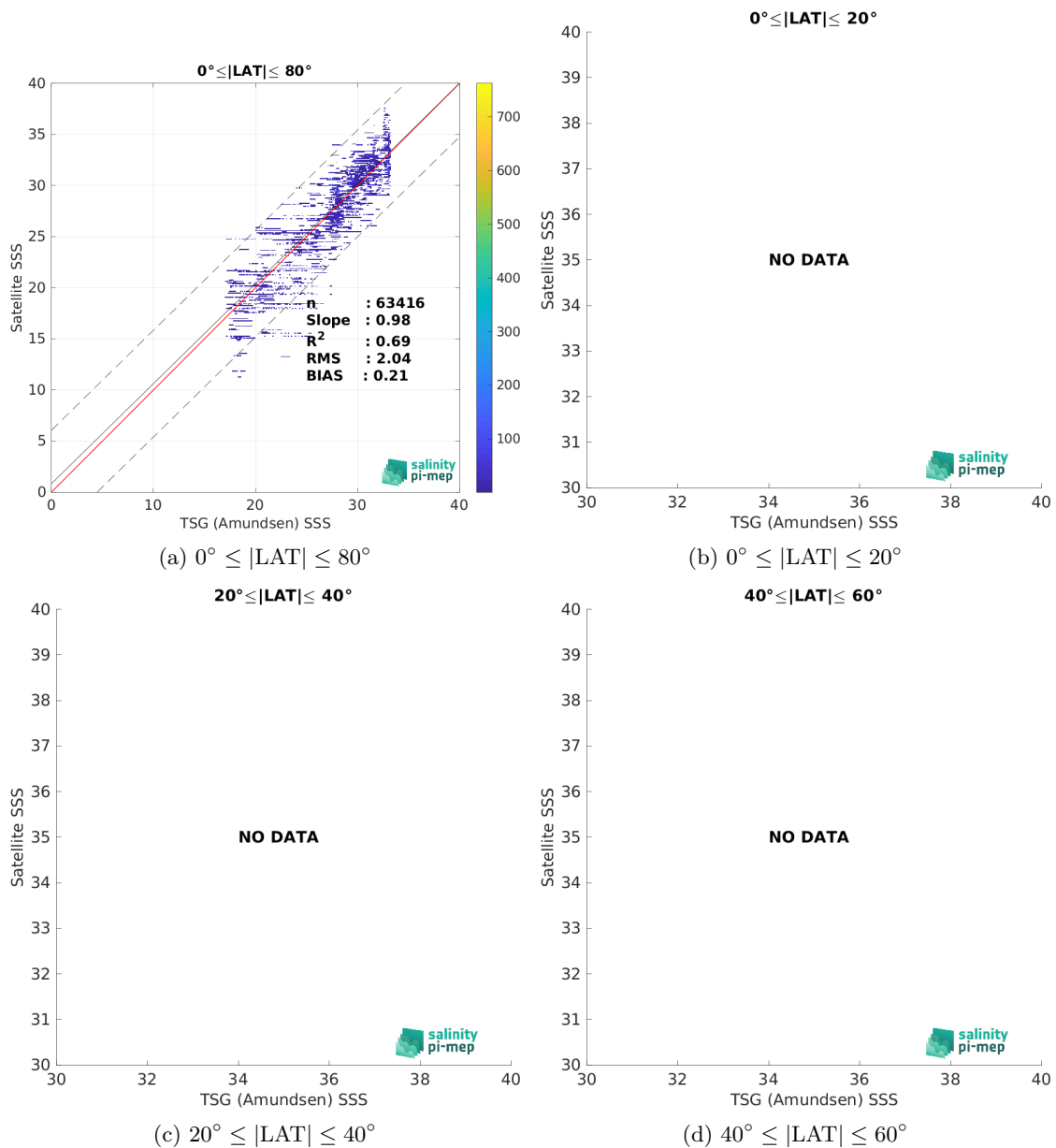
Figure 10: Contour maps of the concentration of SMAP SSS L2 v5.3 - 40 km (RSS) SSS (y-axis) versus TSG (Amundsen) SSS (x-axis) at match-up pairs for different latitude bands. For each plot, the red line shows x=y . The black thin and dashed lines indicate a linear fit through the data cloud and the \pm 95\% confidence levels, respectively. The number match-up pairs n , the slope and R^2 coefficient of the linear fit, the root mean square (RMS) and the mean bias between satellite and in situ data are indicated for each latitude band in each plots.
