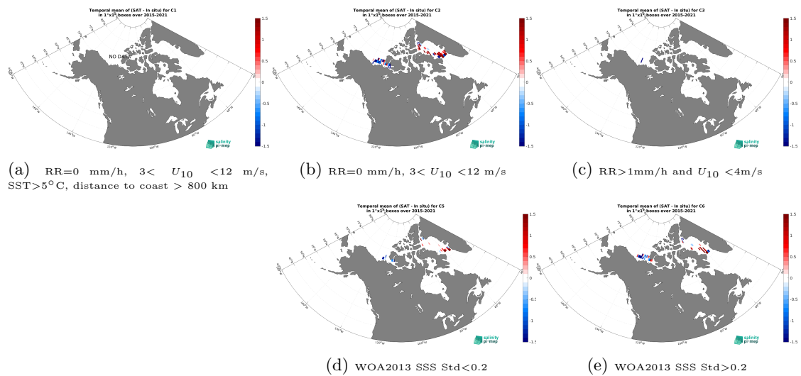
Figure 14: Temporal mean gridded over spatial boxes of size 1^\circ \times 1^\circ of \Delta SSS (SMAP SSS L2 v5.3 - 40 km (RSS) - TSG (Amundsen)) for 5 different subdatasets corresponding to:RR=0 mm/h, 3 < U_{10} < 12 m/s, SST > 5°C, distance to coast > 800 km (a), RR=0 mm/h, 3 < U_{10} < 12 m/s (b), RR > 1mm/h and U_{10} < 4 m/s (c), WOA2013 SSS Std < 0.2 (d), WOA2013 SSS Std > 0.2 (e).
