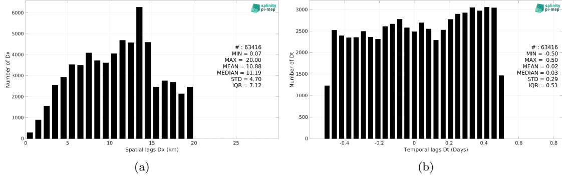
Figure 6: Histograms of the spatial (a) and temporal (b) lags between the location/time of the TSG (Amundsen) measurement and the date of the corresponding SMAP SSS L2 v5.3 - 40 km (RSS) SSS pixel.
