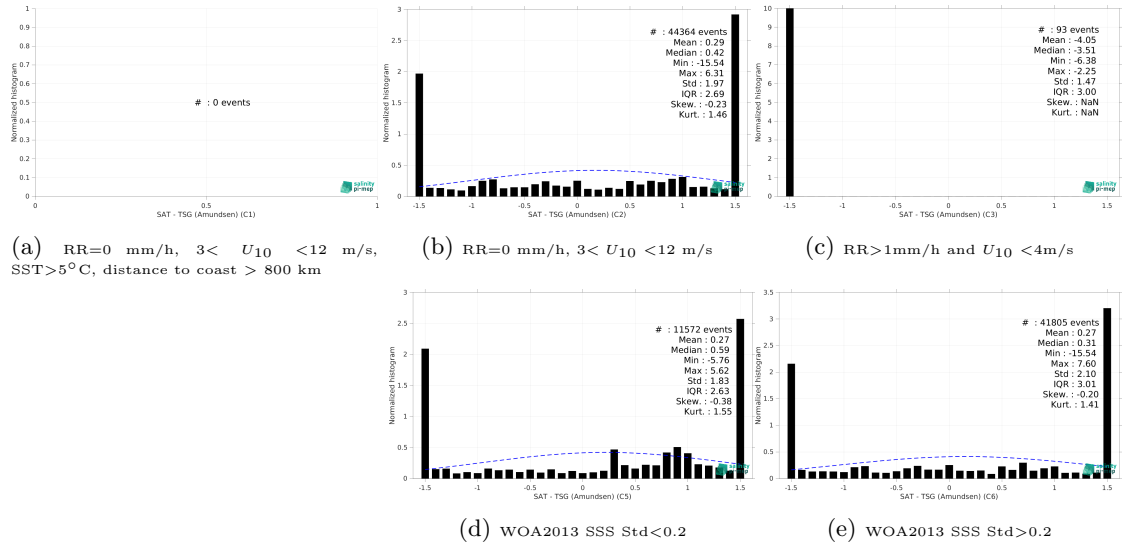
Figure 15: Normalized histogram of \Delta SSS (SMAP SSS L2 v5.3 - 40 km (RSS) - TSG (Amundsen)) for 5 different subdatasets corresponding to: RR=0 mm/h, 3 < U_{10} < 12 m/s, SST > 5°C, distance to coast > 800 km (a), RR=0 mm/h, 3 < U_{10} < 12 m/s (b), RR > 1mm/h and U_{10} < 4 m/s (c), WOA2013 SSS Std < 0.2 (d), WOA2013 SSS Std > 0.2 (e).
