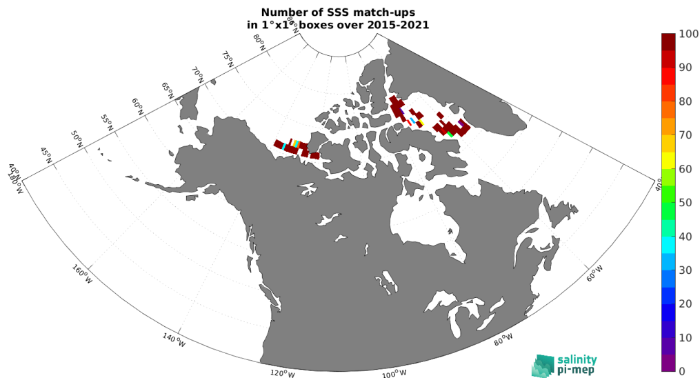
Figure 5: Number of SSS match-ups between TSG (Amundsen) SSS and the SMAP SSS L2 v5.3 - 40 km (RSS) SSS product for the Arctic Ocean Pi-MEP region over 1^\circ \times 1^\circ boxes and for the full satellite product period.
