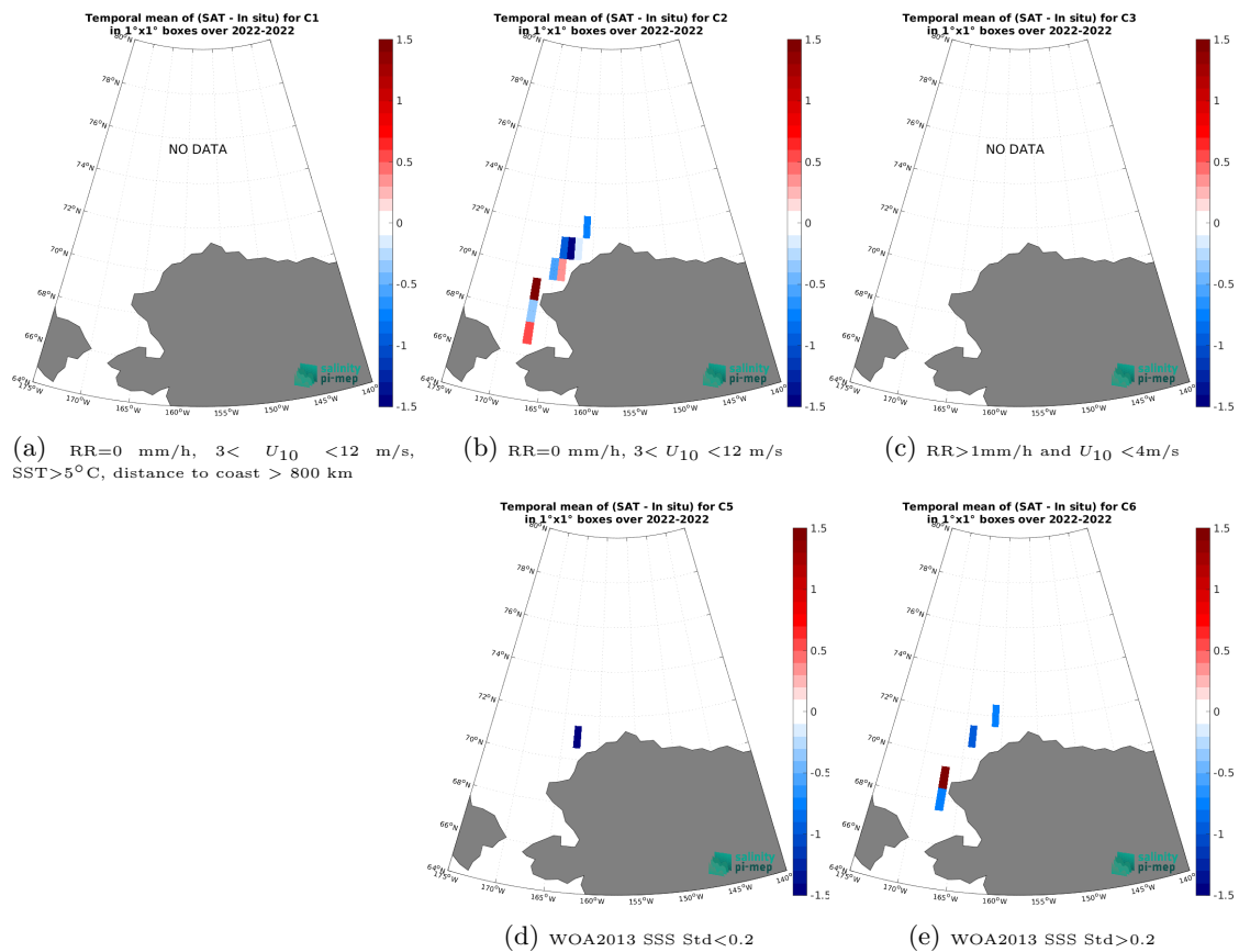
Figure 14: Temporal mean gridded over spatial boxes of size 1^\circ \times 1^\circ of \Delta\text{SSS} (SMAP SSS L2 v5.3 - 40 km (RSS) - SASSIE) for 5 different subdatasets corresponding to:RR=0 mm/h, 3 < U_{10} < 12 m/s, SST>5°C, distance to coast > 800 km (a), RR=0 mm/h, 3 < U_{10} < 12 m/s (b), RR>1mm/h and U_{10} < 4 m/s (c), WOA2013 SSS Std<0.2 (d), WOA2013 SSS Std>0.2 (e).
