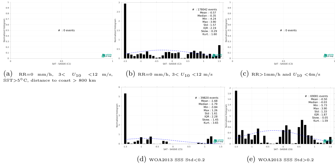
Figure 15: Normalized histogram of \Delta SSS (SMAP SSS L2 v5.3 - 40 km (RSS) - SASSIE) for 5 different subdatasets corresponding to: RR=0 mm/h, 3 < U_{10} < 12 m/s, SST > 5°C, distance to coast > 800 km (a), RR=0 mm/h, 3 < U_{10} < 12 m/s (b), RR > 1mm/h and U_{10} < 4 m/s (c), WOA2013 SSS Std < 0.2 (d), WOA2013 SSS Std > 0.2 (e).
