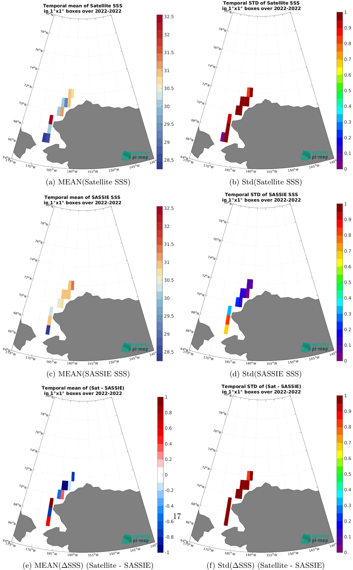
Figure 7: Temporal mean (left) and Std (right) of SSS from SMAP SSS L2 v5.3 - 40 km (RSS) (top), SASSIE (middle), and of \Delta SSS (Satellite - SASSIE). Only match-up pairs are used to generate these maps.
