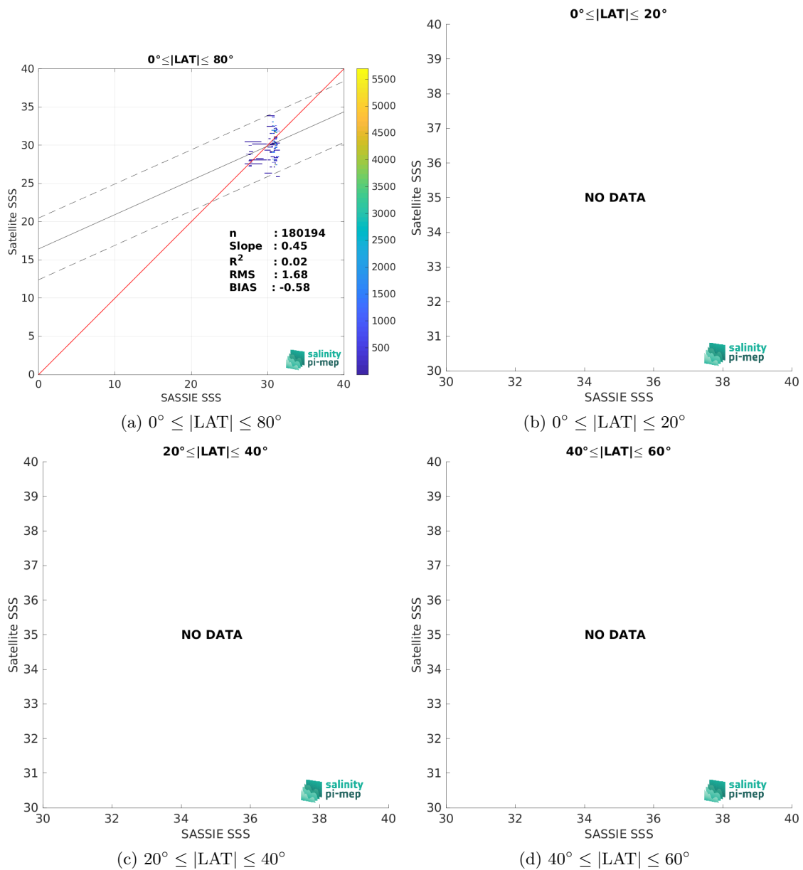
Figure 10: Contour maps of the concentration of SMAP SSS L2 v5.3 - 40 km (RSS) SSS (y-axis) versus SASSIE SSS (x-axis) at match-up pairs for different latitude bands. For each plot, the red line shows x=y . The black thin and dashed lines indicate a linear fit through the data cloud and the \pm 95\% confidence levels, respectively. The number match-up pairs n , the slope and R^2 coefficient of the linear fit, the root mean square (RMS) and the mean bias between satellite and in situ data are indicated for each latitude band in each plots.
