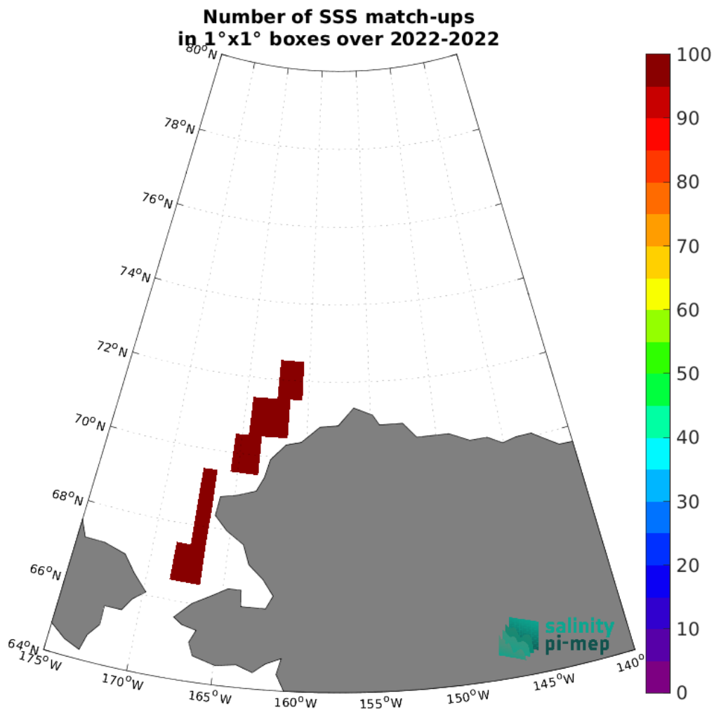
Figure 5: Number of SSS match-ups between SASSIE SSS and the SMAP SSS L2 v5.3 - 40 km (RSS) SSS product for the Arctic Ocean Pi-MEP region over 1°x1° boxes and for the full satellite product period.
