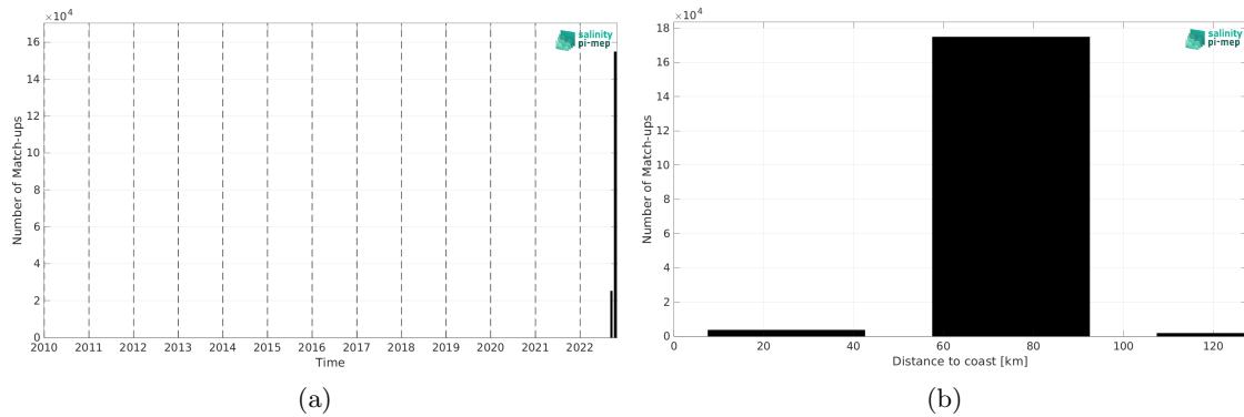
Figure 2: Number of match-ups between SASSIE and SMAP SSS L2 v5.3 - 40 km (RSS) SSS as a function of time (a) and as function of the distance to coast (b) over the Arctic Ocean Pi-MEP region and for the full satellite product period.
