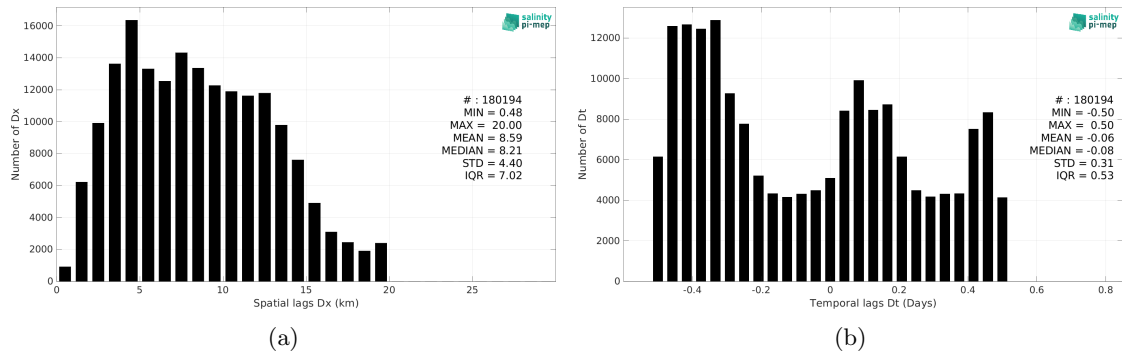
Figure 6: Histograms of the spatial (a) and temporal (b) lags between the location/time of the SASSIE measurement and the date of the corresponding SMAP SSS L2 v5.3 - 40 km (RSS) SSS pixel.
