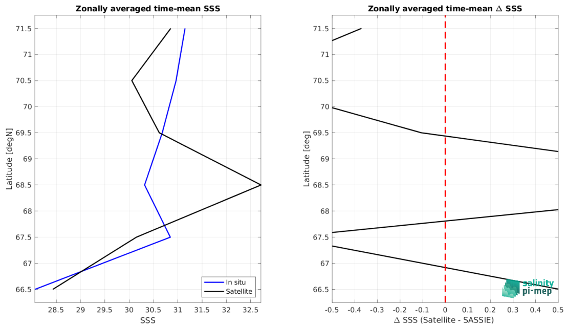
Figure 9: Left panel: Zonal mean SSS from SMAP SSS L2 v5.3 - 40 km (RSS) satellite product (black) and from SASSIE (blue). Right panel: Zonal mean of \Delta SSS (Satellite - SASSIE) for all the collected Pi-MEP match-up pairs estimated over the full satellite product period.
