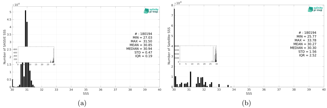
Figure 3: Histograms of SSS from SASSIE (a) and SMAP SSS L2 v5.3 - 40 km (RSS) (b) considering all match-up pairs per bins of 0.1 over the Arctic Ocean Pi-MEP region and for the full satellite product period.
