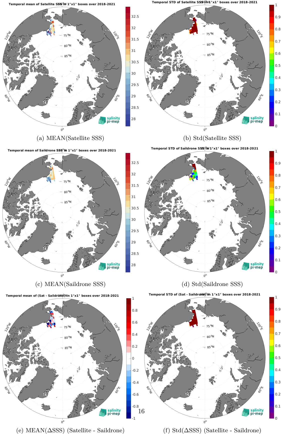
Figure 7: Temporal mean (left) and Std (right) of SSS from SMAP SSS L2 v5.3 - 40 km (RSS) (top), Saildrone (middle), and of \Delta SSS (Satellite - Saildrone). Only match-up pairs are used to generate these maps.
