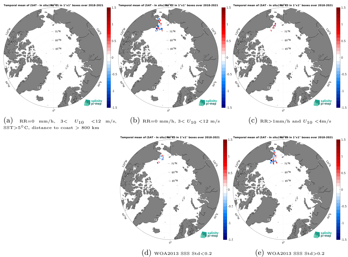
Figure 14: Temporal mean gridded over spatial boxes of size 1^\circ \times 1^\circ of \Delta\text{SSS} (SMAP SSS L2 v5.3 - 40 km (RSS) - Saildrone) for 5 different subdatasets corresponding to:RR=0 mm/h, 3 < U_{10} < 12 m/s, SST>5°C, distance to coast > 800 km (a), RR=0 mm/h, 3 < U_{10} < 12 m/s (b), RR>1mm/h and U_{10} < 4 m/s (c), WOA2013 SSS Std<0.2 (d), WOA2013 SSS Std>0.2 (e).
