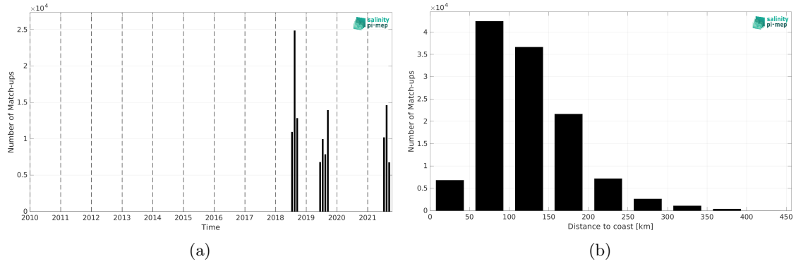
Figure 2: Number of match-ups between Sailldrone and SMAP SSS L2 v5.3 - 40 km (RSS) SSS as a function of time (a) and as function of the distance to coast (b) over the Arctic Ocean Pi-MEP region and for the full satellite product period.
