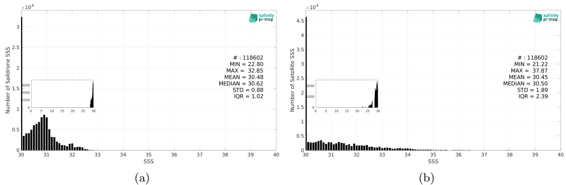
Figure 3: Histograms of SSS from Sailldrone (a) and SMAP SSS L2 v5.3 - 40 km (RSS) (b) considering all match-up pairs per bins of 0.1 over the Arctic Ocean Pi-MEP region and for the full satellite product period.
