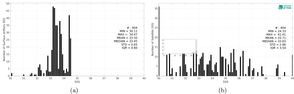
Figure 3: Histograms of SSS from Surface drifters (a) and SMAP SSS L2 v5.3 - 40 km (RSS) (b) considering all match-up pairs per bins of 0.1 over the Arctic Ocean Pi-MEP region and for the full satellite product period.
