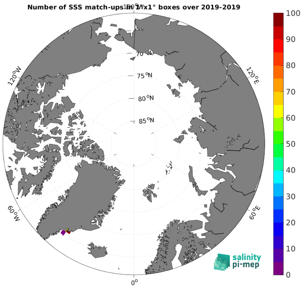
Figure 4: Number of SSS match-ups between Surface drifters SSS and the SMAP SSS L2 v5.3 - 40 km (RSS) SSS product for the Arctic Ocean Pi-MEP region over 1^\circ \times 1^\circ boxes and for the full satellite product period.
