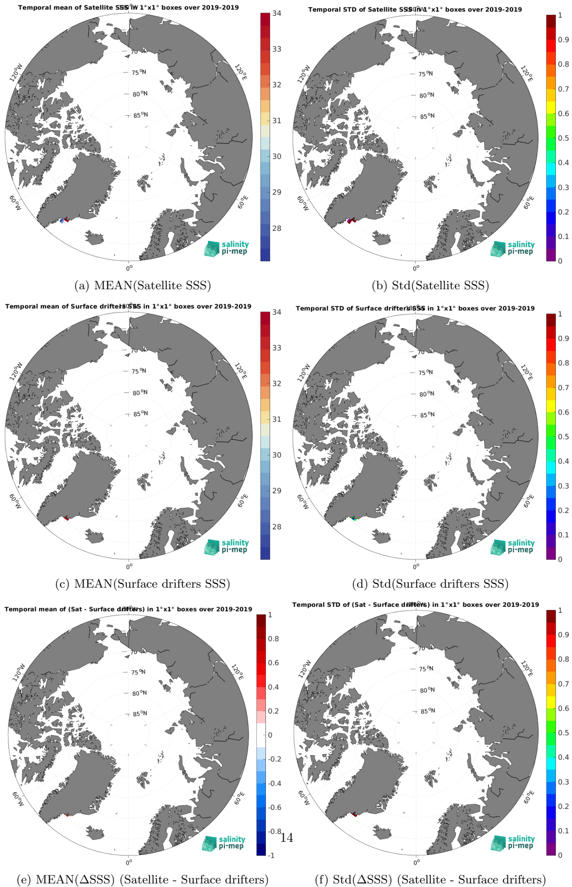
Figure 6: Temporal mean (left) and Std (right) of SSS from SMAP SSS L2 v5.3 - 40 km (RSS) (top), Surface drifters (middle), and of \Delta SSS (Satellite - Surface drifters). Only match-up pairs are used to generate these maps.
