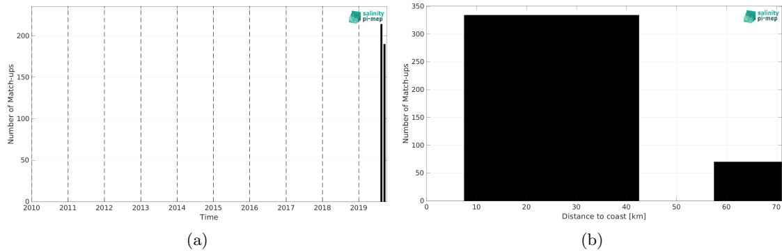
Figure 2: Number of match-ups between Surface drifters and SMAP SSS L2 v5.3 - 40 km (RSS) SSS as a function of time (a) and as function of the distance to coast (b) over the Arctic Ocean Pi-MEP region and for the full satellite product period.
