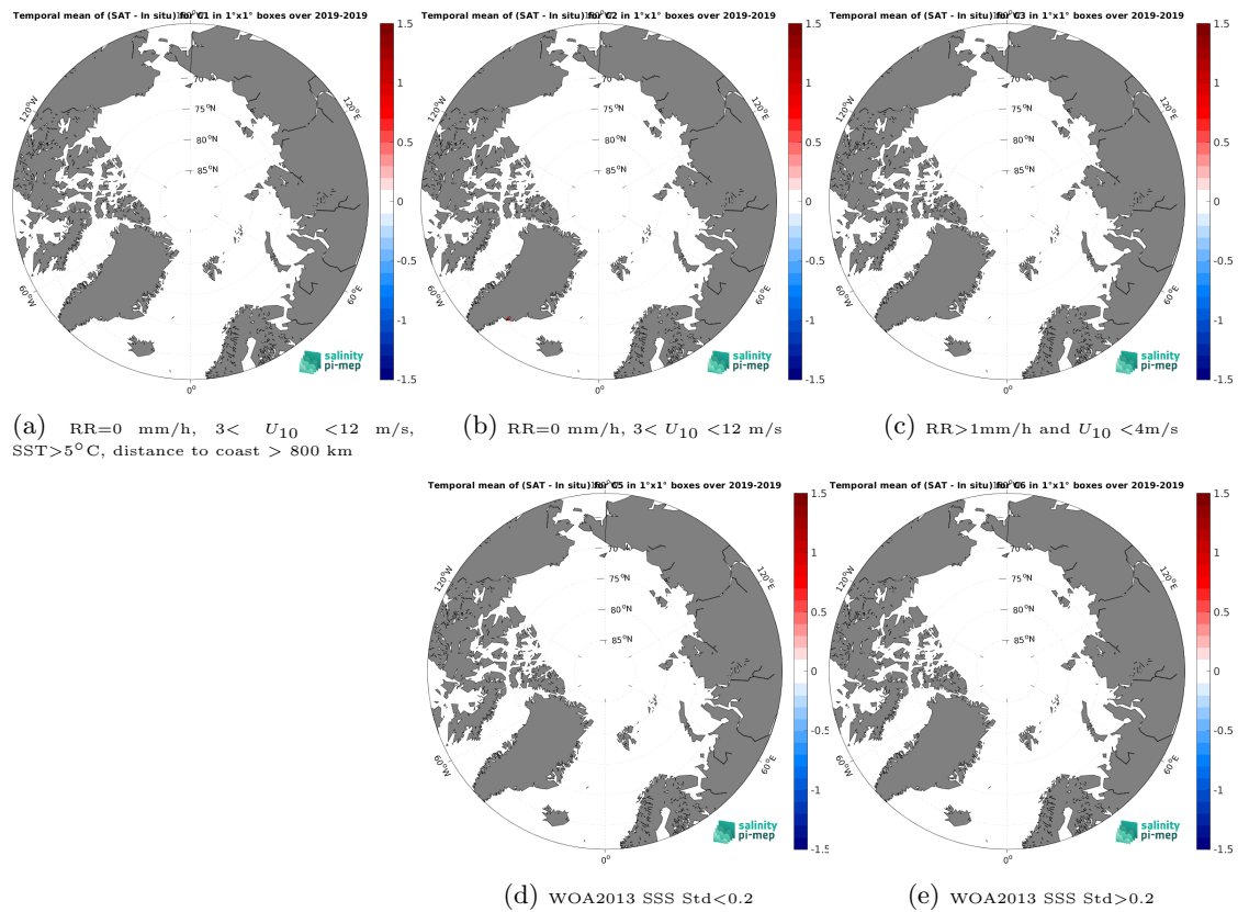
Figure 13: Temporal mean gridded over spatial boxes of size 1^\circ \times 1^\circ of \Delta SSS (SMAP SSS L2 v5.3 - 40 km (RSS) - Surface drifters) for 5 different subdatasets corresponding to:RR=0 mm/h, 3 < U_{10} < 12 m/s, SST > 5^\circ\text{C} , distance to coast > 800 km (a), RR=0 mm/h, 3 < U_{10} < 12 m/s (b), RR > 1 mm/h and U_{10} < 4 m/s (c), WOA2013 SSS Std < 0.2 (d), WOA2013 SSS Std > 0.2 (e).
