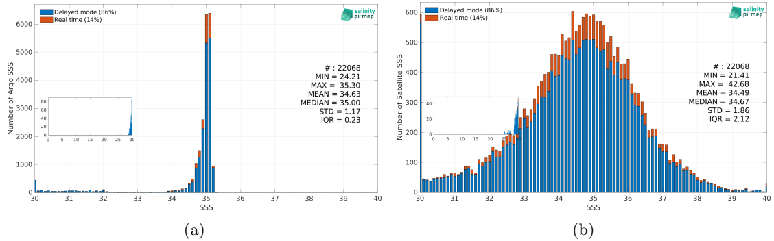
Figure 3: Histograms of SSS from Argo (a) and SMAP SSS L2 v5.3 - 40 km (RSS) (b) considering all match-up pairs per bins of 0.1 over the Arctic Ocean Pi-MEP region and for the full satellite product period.
