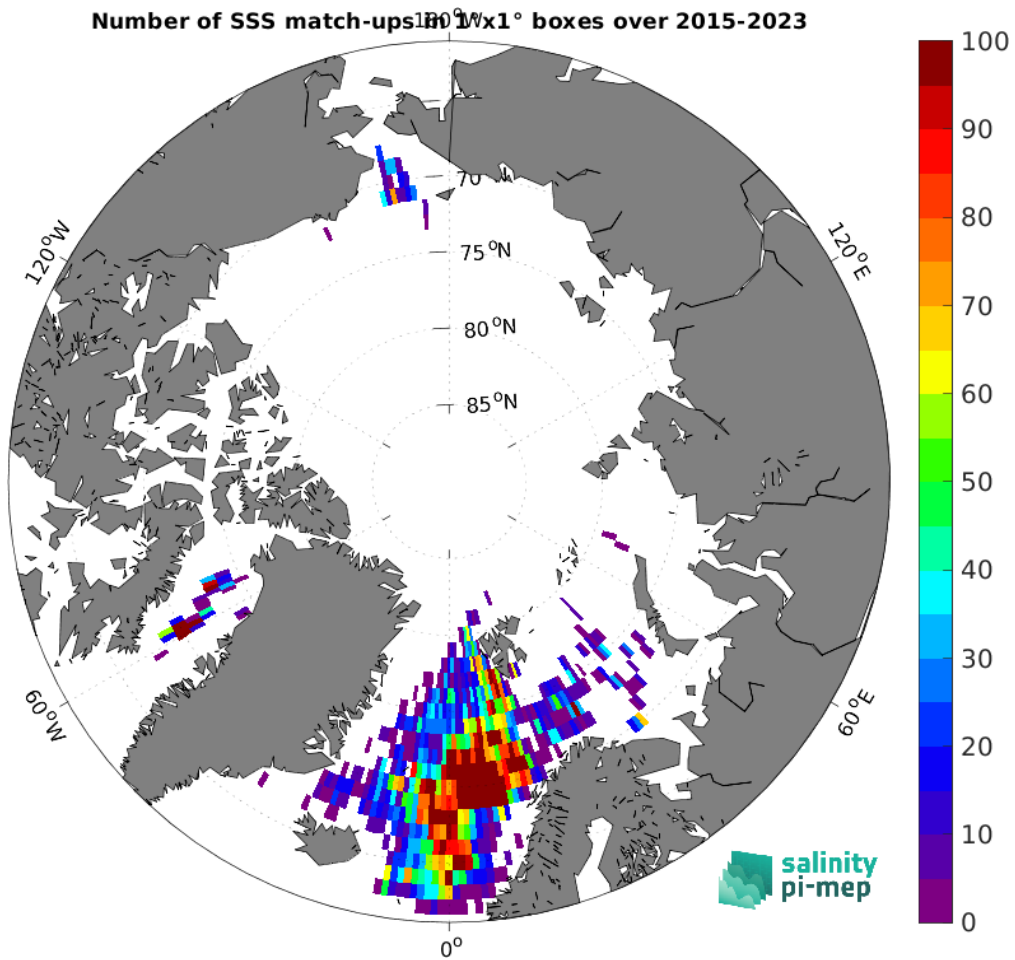
Figure 5: Number of SSS match-ups between Argo SSS and the SMAP SSS L2 v5.3 - 40 km (RSS) SSS product for the Arctic Ocean Pi-MEP region over 1^\circ \times 1^\circ boxes and for the full satellite product period.
