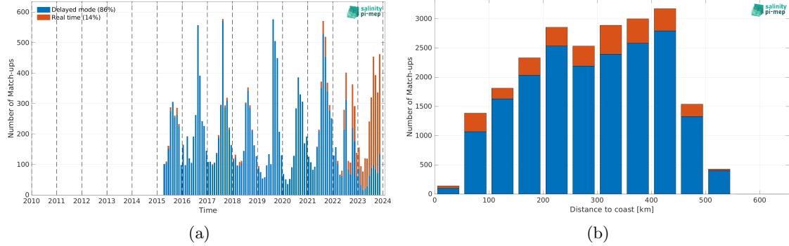
Figure 2: Number of match-ups between Argo and SMAP SSS L2 v5.3 - 40 km (RSS) SSS as a function of time (a) and as function of the distance to coast (b) over the Arctic Ocean Pi-MEP region and for the full satellite product period.
