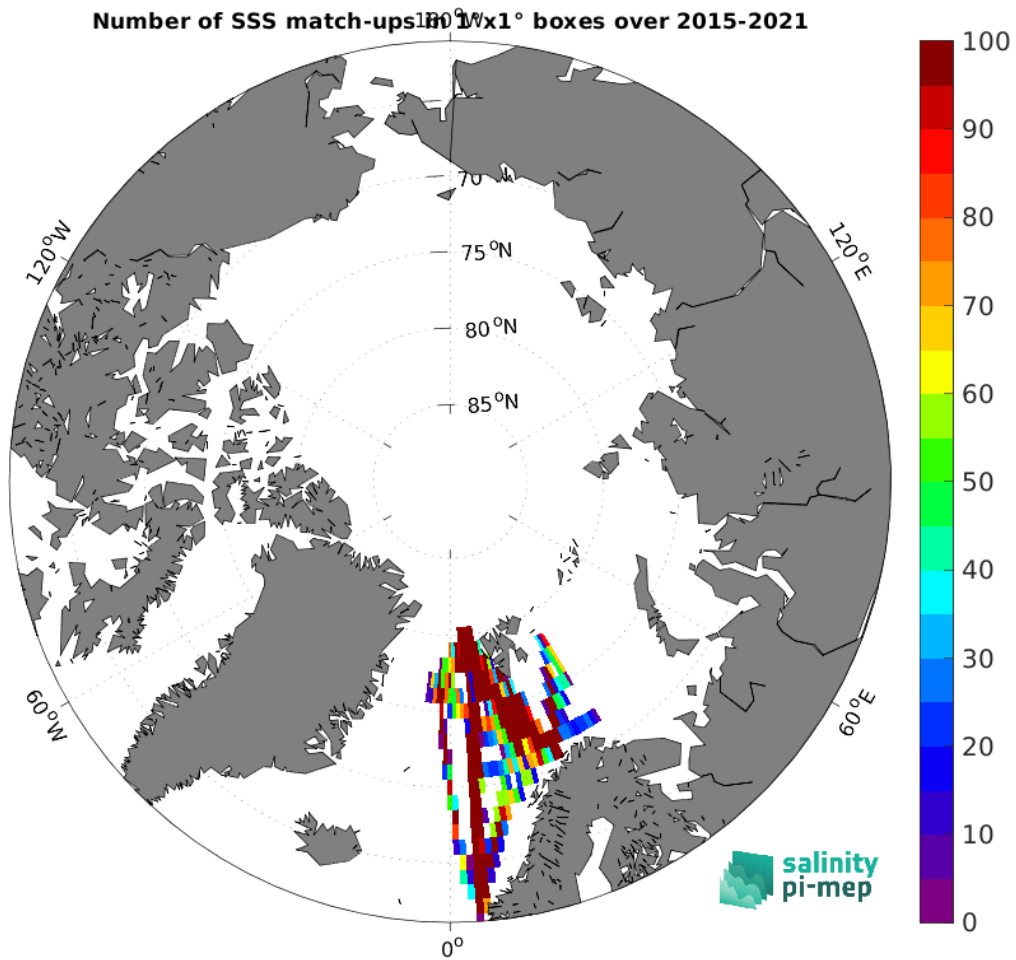
Figure 4: Number of SSS match-ups between TSG (Polarstern) SSS and the SMAP SSS L2 v5 - 40 km (RSS) SSS product for the Arctic Ocean Pi-MEP region over 1^\circ \times 1^\circ boxes and for the full satellite product period.
