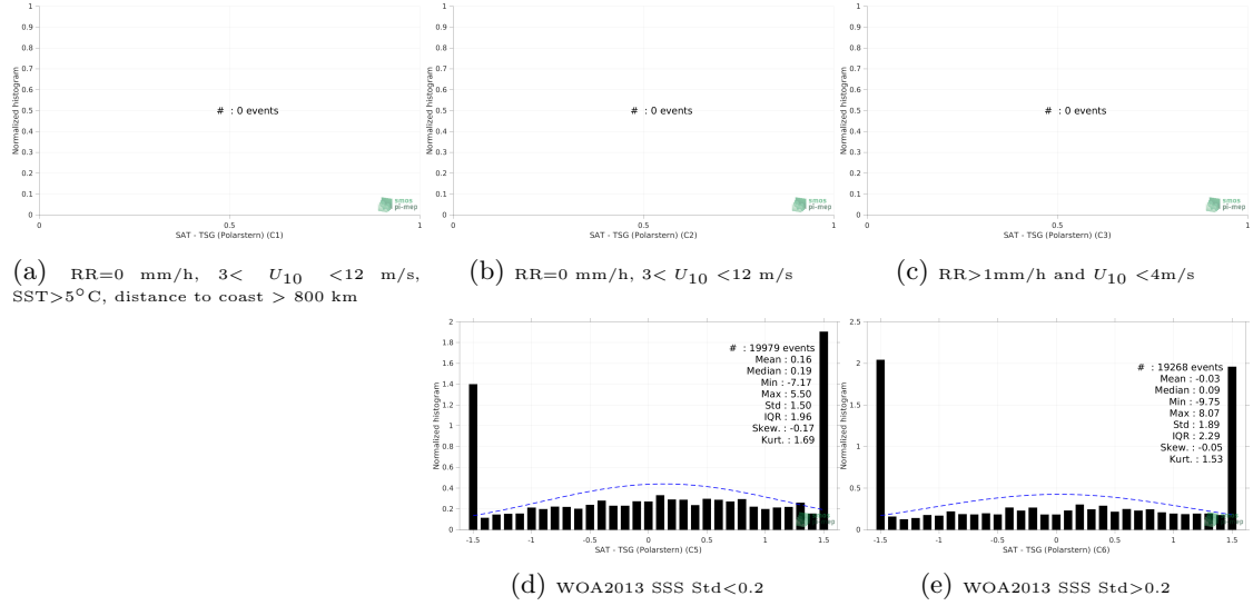
Figure 13: Normalized histogram of \Delta SSS (SMAP SSS L2 v5 - 40 km (RSS) - TSG (Polarstern)) for 5 different subdatasets corresponding to: RR=0 mm/h, 3 < U_{10} < 12 m/s, SST > 5°C, distance to coast > 800 km (a), RR=0 mm/h, 3 < U_{10} < 12 m/s (b), RR > 1mm/h and U_{10} < 4 m/s (c), WOA2013 SSS Std < 0.2 (d), WOA2013 SSS Std > 0.2 (e).
