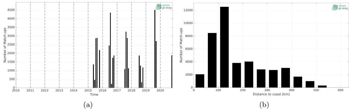
Figure 1: Number of match-ups between TSG (Polarstern) and SMAP SSS L2 v5 - 40 km (RSS) SSS as a function of time (a) and as function of the distance to coast (b) over the Arctic Ocean Pi-MEP region and for the full satellite product period.
