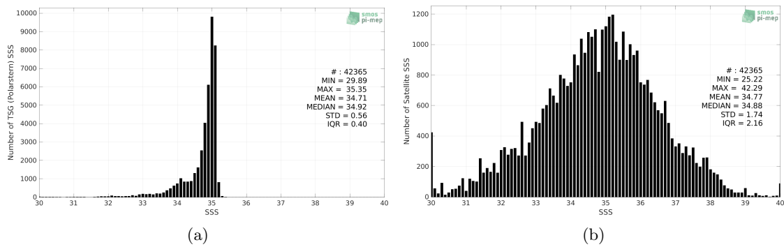
Figure 2: Histograms of SSS from TSG (Polarstern) (a) and SMAP SSS L2 v5 - 40 km (RSS) (b) considering all match-up pairs per bins of 0.1 over the Arctic Ocean Pi-MEP region and for the full satellite product period.
