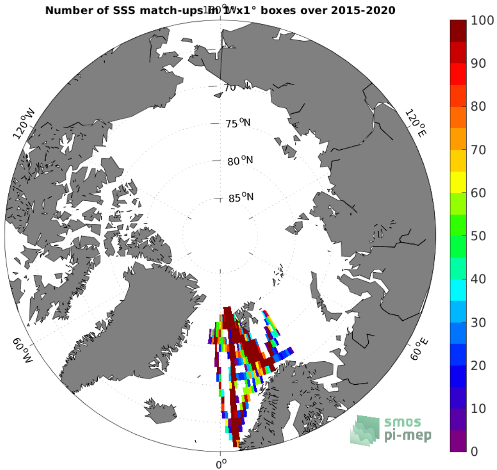
Figure 4: Number of SSS match-ups between TSG (Polarstern) SSS and the SMAP SSS L2 v5 - 40 km (RSS) SSS product for the Arctic Ocean Pi-MEP region over 1^{\circ} \times 1^{\circ} boxes and for the full satellite product period.
