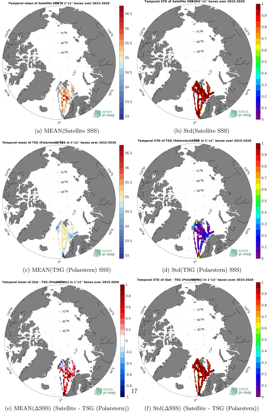
Figure 6: Temporal mean (left) and Std (right) of SSS from SMAP SSS L2 v5 - 40 km (RSS) (top), TSG (Polarstern) (middle), and of \Delta SSS (Satellite - TSG (Polarstern)). Only match-up pairs are used to generate these maps.
