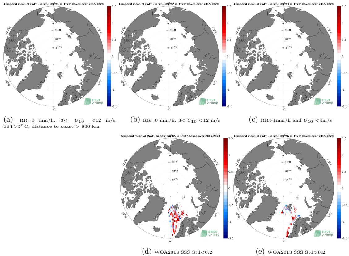
Figure 12: Temporal mean gridded over spatial boxes of size 1^{\circ}\times 1^{\circ} of \Delta\text{SSS} (SMAP SSS L2 v5 - 40 km (RSS) - TSG (Polarstern)) for 5 different subdatasets corresponding to:RR=0 mm/h, 3 < U_{10} < 12 m/s, \text{SST}>5^{\circ}\text{C} , distance to coast > 800 km (a), RR=0 mm/h, 3 < U_{10} < 12 m/s (b), RR >1 mm/h and U_{10} < 4 m/s (c), WOA2013 SSS Std <0.2 (d), WOA2013 SSS Std >0.2 (e).
