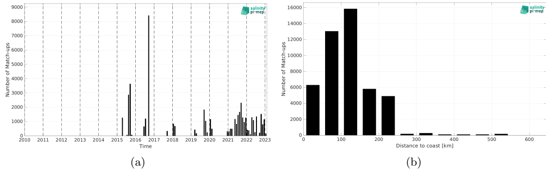
Figure 1: Number of match-ups between TSG (LEGOS-DM) and SMAP SSS L2 v5 - 40 km (RSS) SSS as a function of time (a) and as function of the distance to coast (b) over the Arctic Ocean Pi-MEP region and for the full satellite product period.
