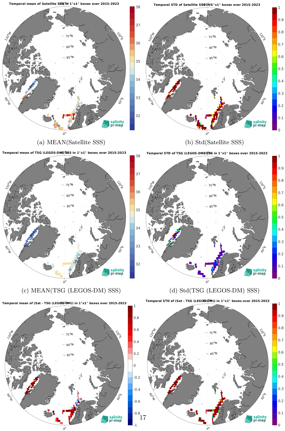
Figure 6: Temporal mean (left) and Std (right) of SSS from SMAP SSS L2 v5 - 40 km (RSS) (top), TSG (LEGOS-DM) (middle), and of \Delta SSS (Satellite - TSG (LEGOS-DM)). Only match-up pairs are used to generate these maps.
