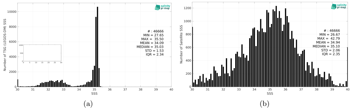
Figure 2: Histograms of SSS from TSG (LEGOS-DM) (a) and SMAP SSS L2 v5 - 40 km (RSS) (b) considering all match-up pairs per bins of 0.1 over the Arctic Ocean Pi-MEP region and for the full satellite product period.
