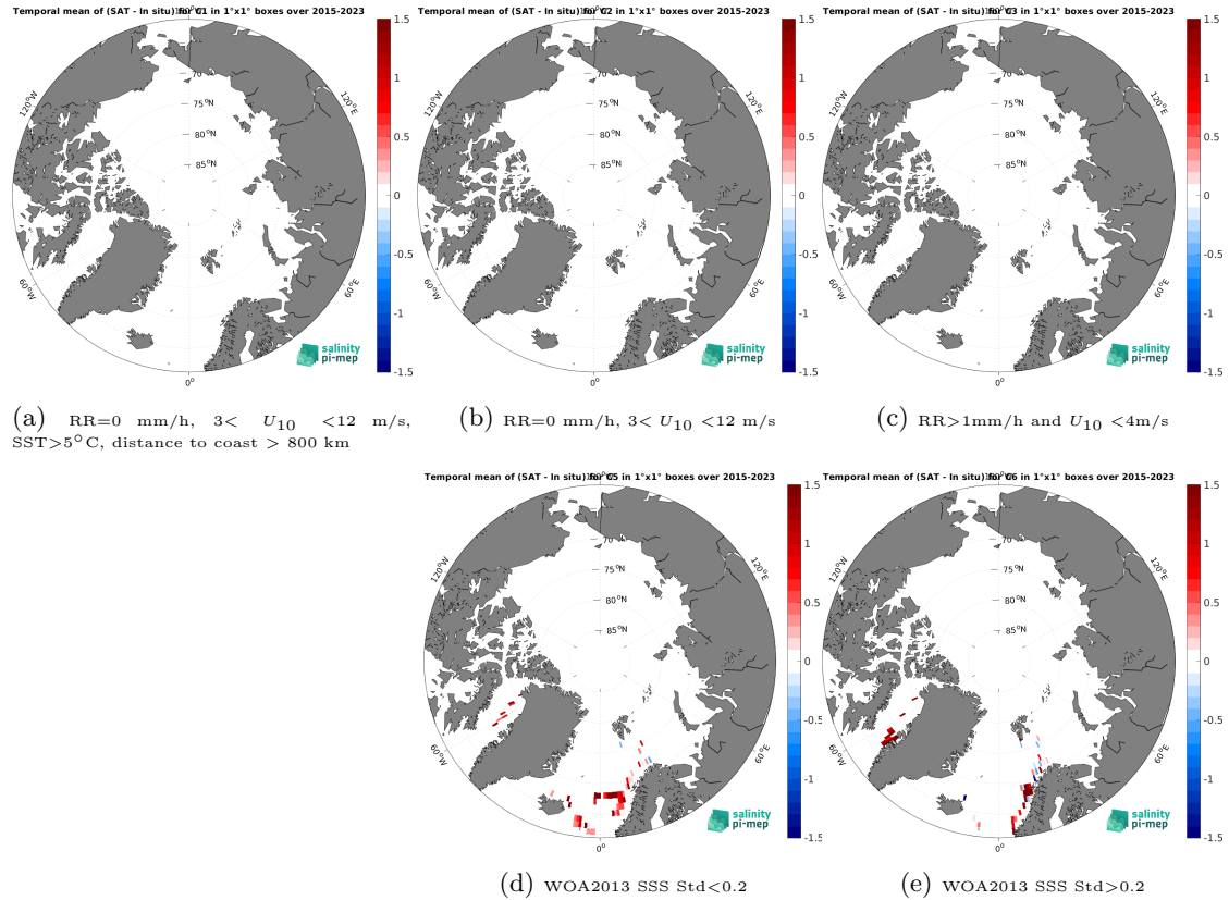
Figure 12: Temporal mean gridded over spatial boxes of size 1^{\circ}\times 1^{\circ} of \Delta\text{SSS} (SMAP SSS L2 v5 - 40 km (RSS) - TSG (LEGOS-DM)) for 5 different subdatasets corresponding to:RR=0 mm/h, 3 < U_{10} < 12 m/s, SST >5^{\circ}\text{C} , distance to coast > 800 km (a), RR=0 mm/h, 3 < U_{10} < 12 m/s (b), RR >1 mm/h and U_{10} < 4 m/s (c), WOA2013 SSS Std <0.2 (d), WOA2013 SSS Std >0.2 (e).
