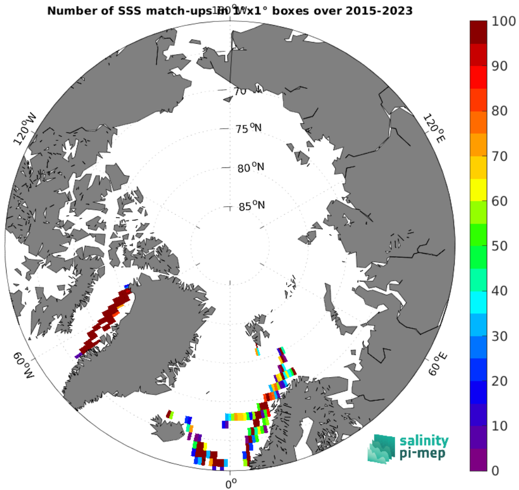
Figure 4: Number of SSS match-ups between TSG (LEGOS-DM) SSS and the SMAP SSS L2 v5 - 40 km (RSS) SSS product for the Arctic Ocean Pi-MEP region over 1^\circ \times 1^\circ boxes and for the full satellite product period.
