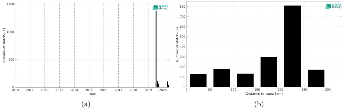
Figure 1: Number of match-ups between TSG (Lauge-Koch) and SMAP SSS L2 v5 - 40 km (RSS) SSS as a function of time (a) and as function of the distance to coast (b) over the Arctic Ocean Pi-MEP region and for the full satellite product period.
