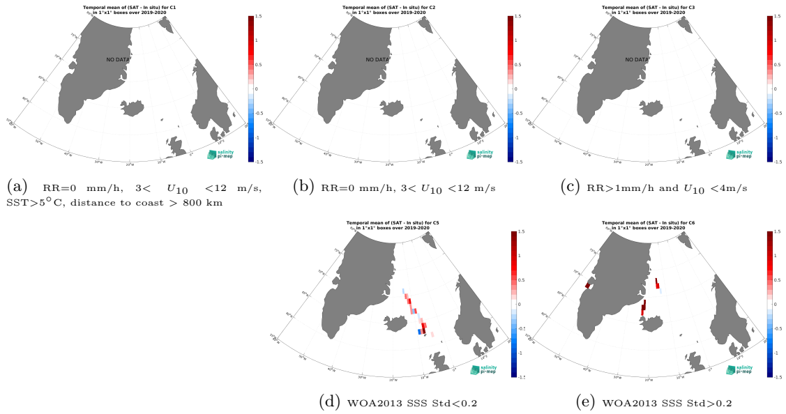
Figure 12: Temporal mean gridded over spatial boxes of size 1^{\circ}\times 1^{\circ} of \Delta\text{SSS} (SMAP SSS L2 v5 - 40 km (RSS) - TSG (Lauge-Koch)) for 5 different subdatasets corresponding to:RR=0 mm/h, 3 < U_{10} < 12 m/s, SST > 5^{\circ}\text{C} , distance to coast > 800 km (a), RR=0 mm/h, 3 < U_{10} < 12 m/s (b), RR > 1\text{mm/h} and U_{10} < 4\text{m/s} (c), WOA2013 SSS Std < 0.2 (d), WOA2013 SSS Std > 0.2 (e).
