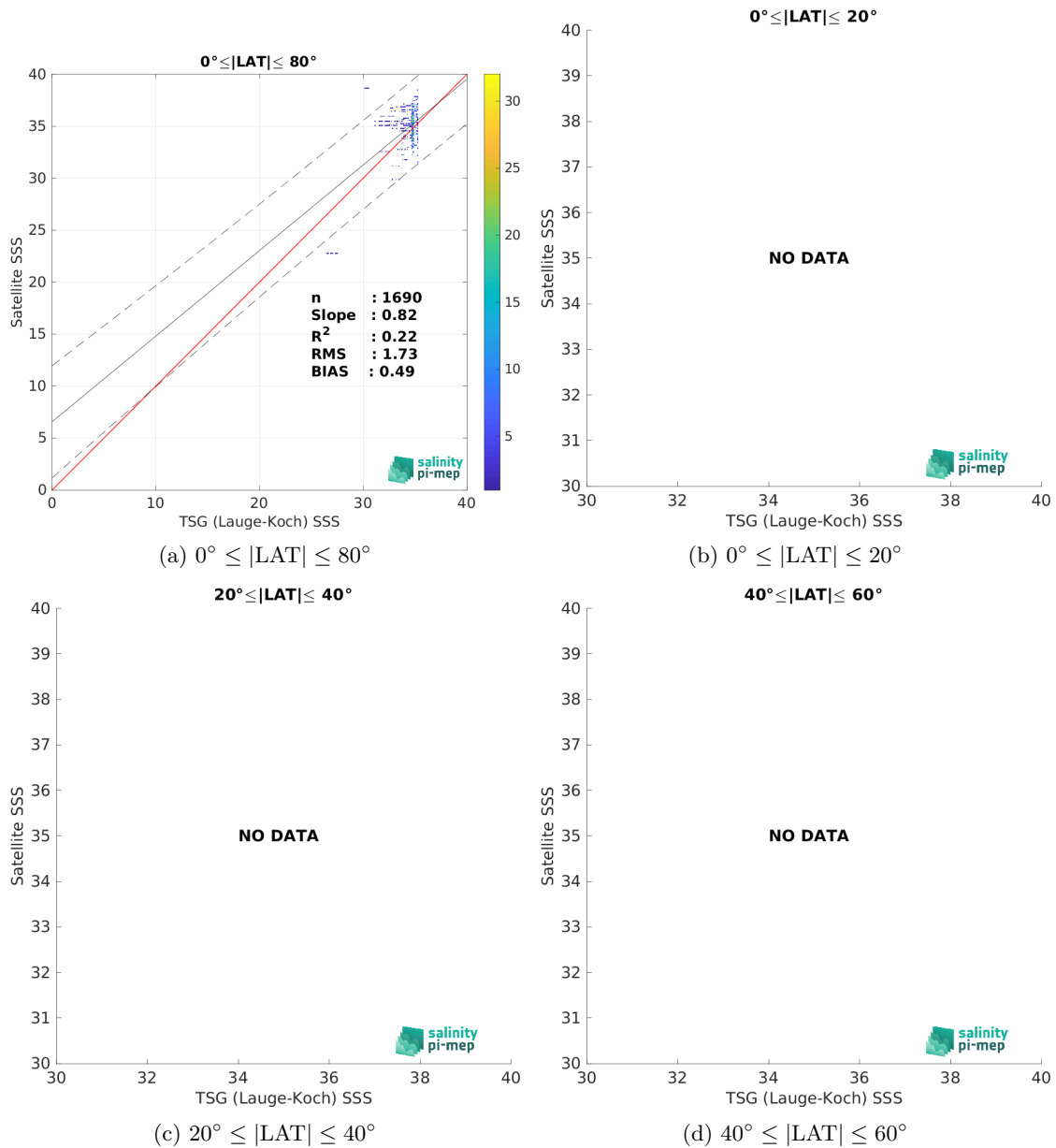
Figure 9: Contour maps of the concentration of SMAP SSS L2 v5 - 40 km (RSS) SSS (y-axis) versus TSG (Lauge-Koch) SSS (x-axis) at match-up pairs for different latitude bands. For each plot, the red line shows x=y . The black thin and dashed lines indicate a linear fit through the data cloud and the \pm 95\% confidence levels, respectively. The number match-up pairs n , the slope and R^2 coefficient of the linear fit, the root mean square (RMS) and the mean bias between satellite and in situ data are indicated for each latitude band in each plots.
