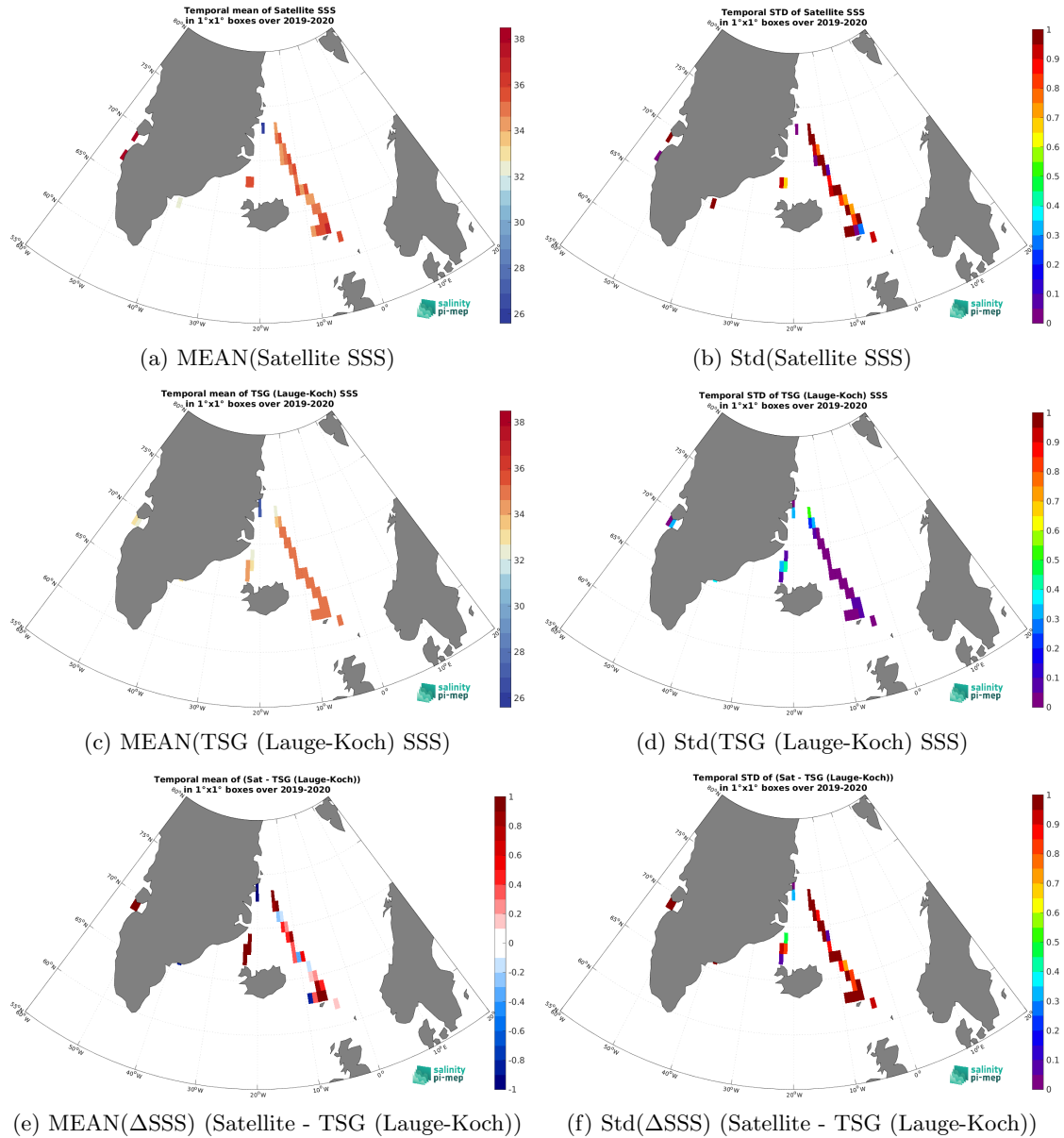
Figure 6: Temporal mean (left) and Std (right) of SSS from SMAP SSS L2 v5 - 40 km (RSS) (top), TSG (Lauge-Koch) (middle), and of \Delta SSS (Satellite - TSG (Lauge-Koch)). Only match-up pairs are used to generate these maps.
