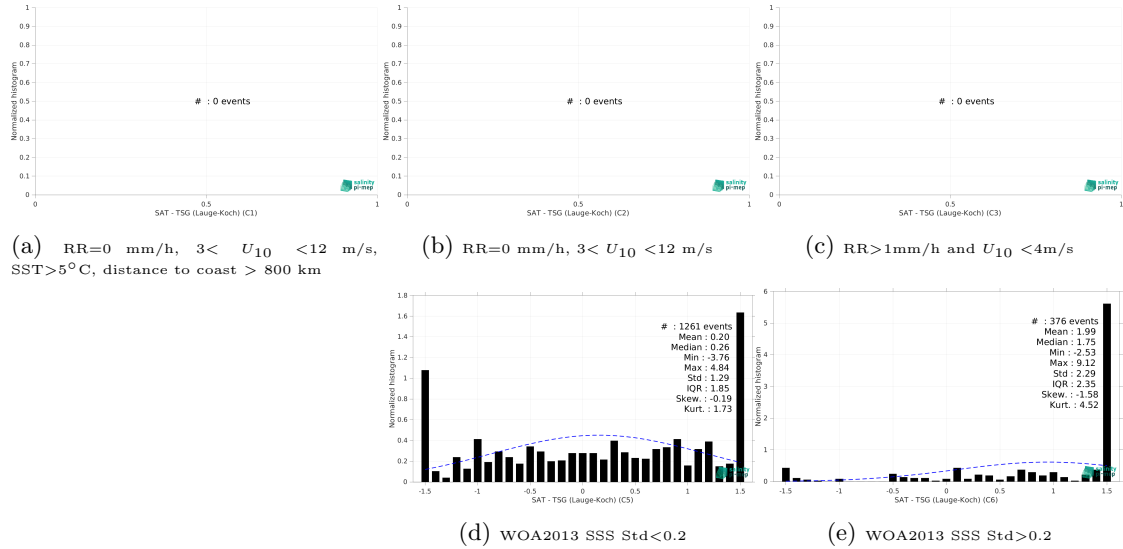
Figure 13: Normalized histogram of \Delta SSS (SMAP SSS L2 v5 - 40 km (RSS) - TSG (Lauge-Koch)) for 5 different subdatasets corresponding to: RR=0 mm/h, 3 < U_{10} < 12 m/s, SST > 5°C, distance to coast > 800 km (a), RR=0 mm/h, 3 < U_{10} < 12 m/s (b), RR > 1mm/h and U_{10} < 4 m/s (c), WOA2013 SSS Std < 0.2 (d), WOA2013 SSS Std > 0.2 (e).
