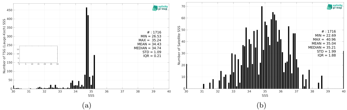
Figure 2: Histograms of SSS from TSG (Lauge-Koch) (a) and SMAP SSS L2 v5 - 40 km (RSS) (b) considering all match-up pairs per bins of 0.1 over the Arctic Ocean Pi-MEP region and for the full satellite product period.
