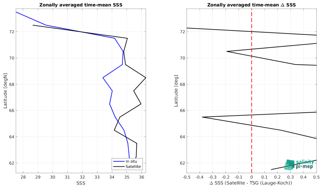
Figure 8: Left panel: Zonal mean SSS from SMAP SSS L2 v5 - 40 km (RSS) satellite product (black) and from TSG (Lauge-Koch) (blue). Right panel: Zonal mean of \Delta SSS (Satellite - TSG (Lauge-Koch)) for all the collected Pi-MEP match-up pairs estimated over the full satellite product period.
