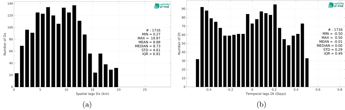
Figure 5: Histograms of the spatial (a) and temporal (b) lags between the location/time of the TSG (Lauge-Koch) measurement and the date of the corresponding SMAP SSS L2 v5 - 40 km (RSS) SSS pixel.
