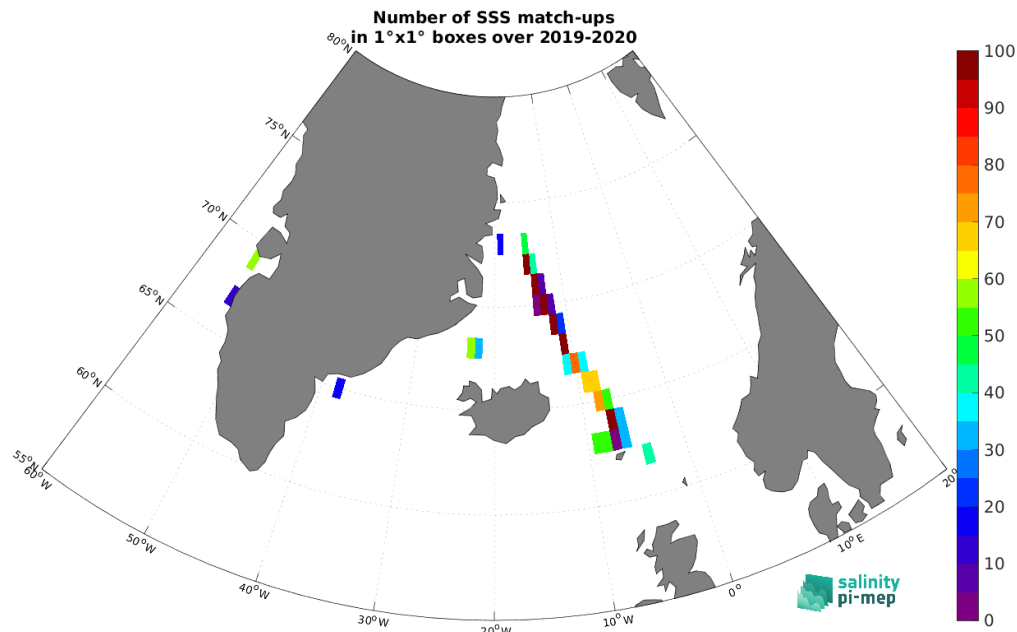
Figure 4: Number of SSS match-ups between TSG (Lauge-Koch) SSS and the SMAP SSS L2 v5 - 40 km (RSS) SSS product for the Arctic Ocean Pi-MEP region over 1^\circ \times 1^\circ boxes and for the full satellite product period.
