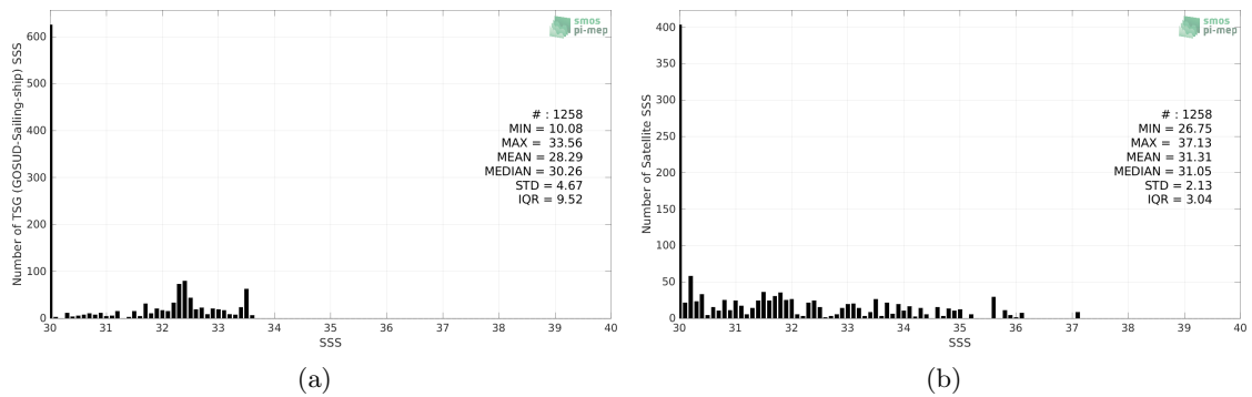
Figure 2: Histograms of SSS from TSG (GOSUD-Sailing-ship) (a) and SMAP SSS L2 v5 - 40 km (RSS) (b) considering all match-up pairs per bins of 0.1 over the Arctic Ocean Pi-MEP region and for the full satellite product period.
