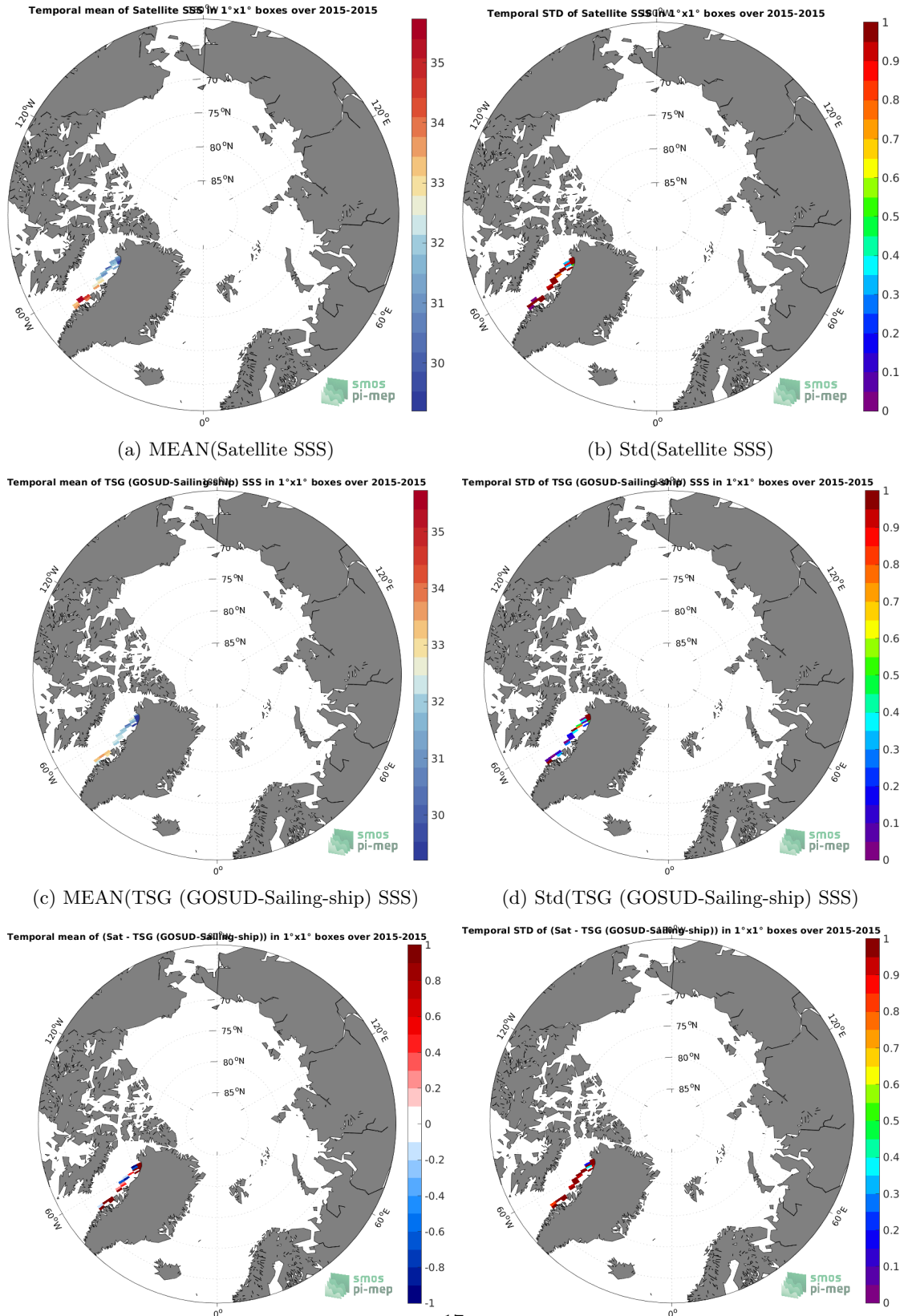
Figure 6: Temporal mean (left) and Std (right) of SSS from SMAP SSS L2 v5 - 40 km (RSS) (top), TSG (GOSUD-Sailing-ship) (middle), and of \Delta SSS (Satellite - TSG (GOSUD-Sailing-ship)). Only match-up pairs are used to generate these maps.
