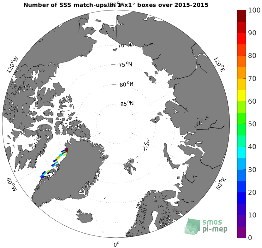
Figure 4: Number of SSS match-ups between TSG (GOSUD-Sailing-ship) SSS and the SMAP SSS L2 v5 - 40 km (RSS) SSS product for the Arctic Ocean Pi-MEP region over 1^\circ \times 1^\circ boxes and for the full satellite product period.
