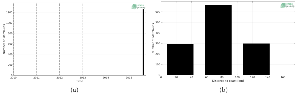
Figure 1: Number of match-ups between TSG (GOSUD-Sailing-ship) and SMAP SSS L2 v5 - 40 km (RSS) SSS as a function of time (a) and as function of the distance to coast (b) over the Arctic Ocean Pi-MEP region and for the full satellite product period.
