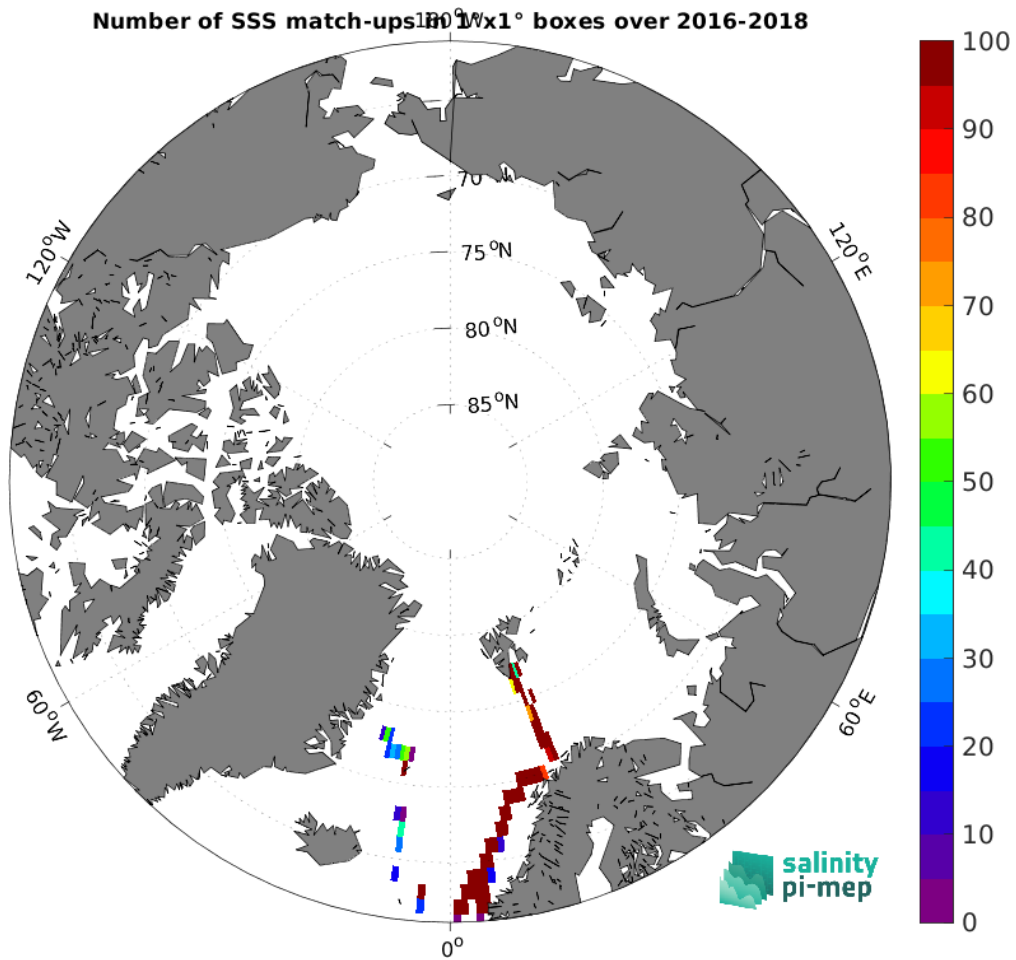
Figure 4: Number of SSS match-ups between TSG (GOSUD-Research-vessel) SSS and the SMAP SSS L2 v5 - 40 km (RSS) SSS product for the Arctic Ocean Pi-MEP region over 1^{\circ} \times 1^{\circ} boxes and for the full satellite product period.
