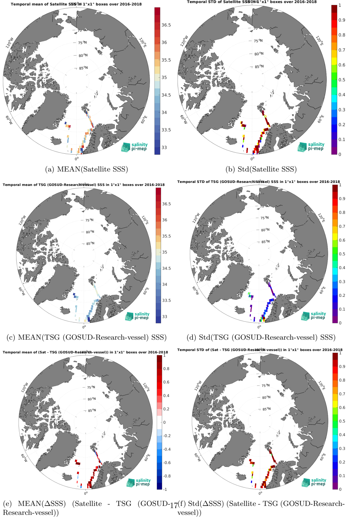
Figure 6: Temporal mean (left) and Std (right) of SSS from SMAP SSS L2 v5 - 40 km (RSS) (top), TSG (GOSUD-Research-vessel) (middle), and of \Delta SSS (Satellite - TSG (GOSUD-Research-vessel)). Only match-up pairs are used to generate these maps.
