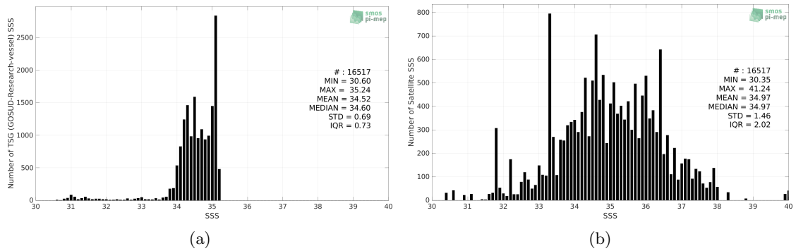
Figure 2: Histograms of SSS from TSG (GOSUD-Research-vessel) (a) and SMAP SSS L2 v5 - 40 km (RSS) (b) considering all match-up pairs per bins of 0.1 over the Arctic Ocean Pi-MEP region and for the full satellite product period.
