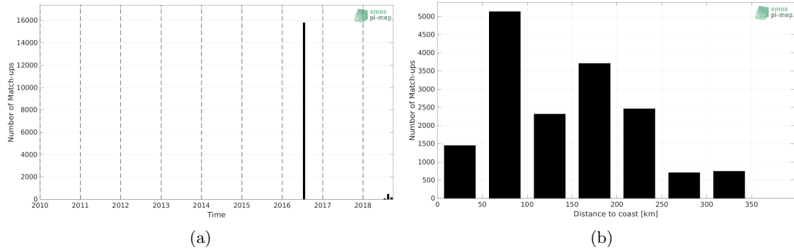
Figure 1: Number of match-ups between TSG (GOSUD-Research-vessel) and SMAP SSS L2 v5 - 40 km (RSS) SSS as a function of time (a) and as function of the distance to coast (b) over the Arctic Ocean Pi-MEP region and for the full satellite product period.
