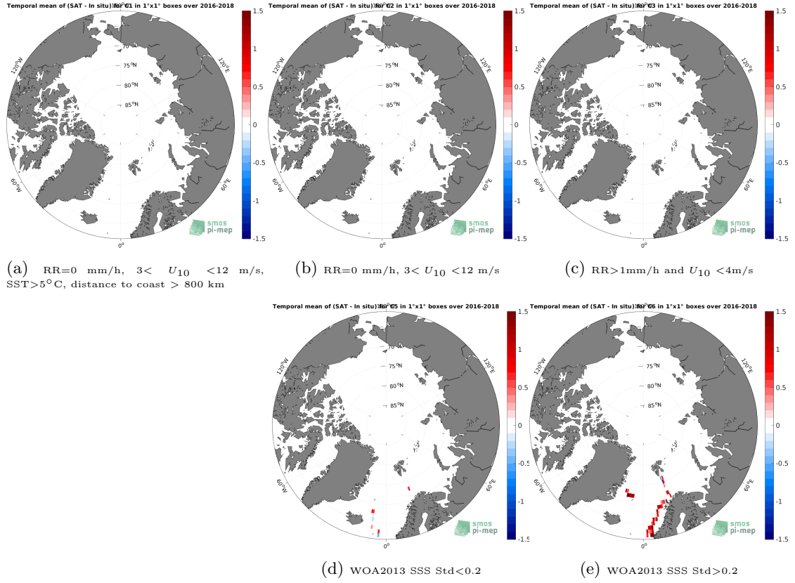
Figure 12: Temporal mean gridded over spatial boxes of size 1^\circ \times 1^\circ of \Delta\text{SSS} (SMAP SSS L2 v5 - 40 km (RSS) - TSG (GOSUD-Research-vessel)) for 5 different subdatasets corresponding to: RR=0 mm/h, 3 < U_{10} < 12 m/s, SST > 5^\circ\text{C} , distance to coast > 800 km (a), RR=0 mm/h, 3 < U_{10} < 12 m/s (b), RR > 1 mm/h and U_{10} < 4 m/s (c), WOA2013 SSS Std < 0.2 (d), WOA2013 SSS Std > 0.2 (e).
