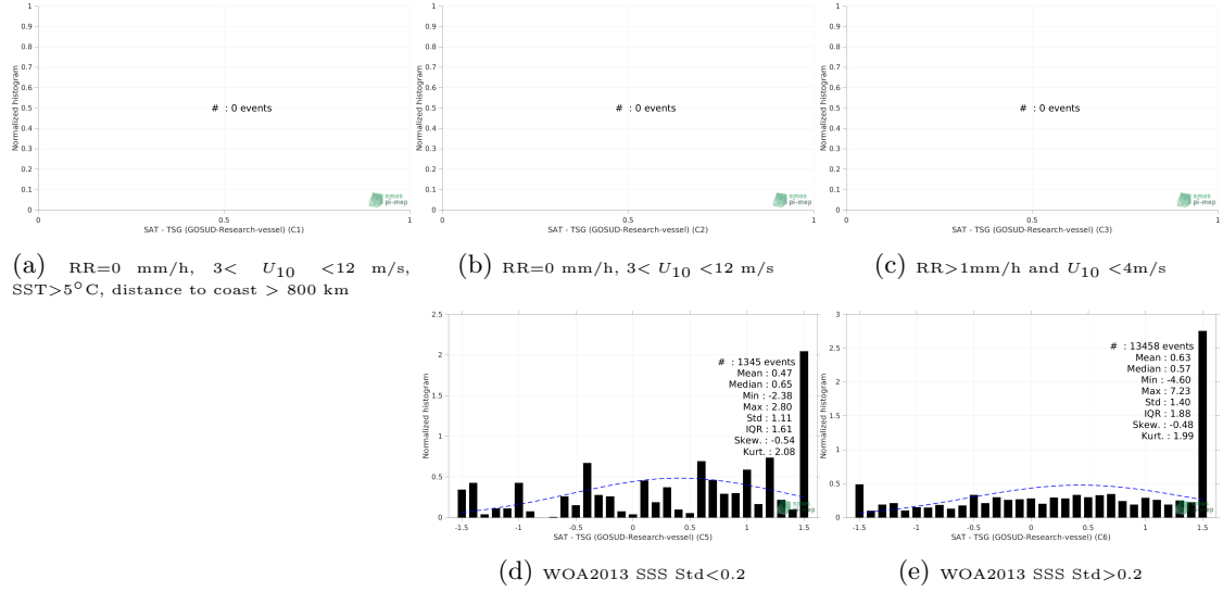
Figure 13: Normalized histogram of \Delta\text{SSS} (SMAP SSS L2 v5 - 40 km (RSS) - TSG (GOSUD-Research-vessel)) for 5 different subdatasets corresponding to: RR=0 mm/h, 3 < U_{10} < 12 m/s, SST > 5^\circ\text{C} , distance to coast > 800 km (a), RR=0 mm/h, 3 < U_{10} < 12 m/s (b), RR > 1 mm/h and U_{10} < 4 m/s (c), WOA2013 SSS Std < 0.2 (d), WOA2013 SSS Std > 0.2 (e).
