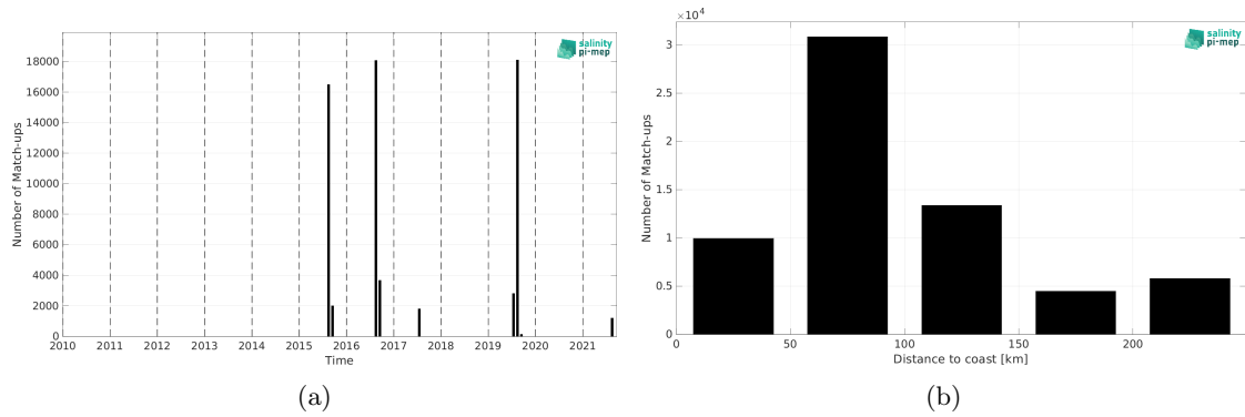
Figure 1: Number of match-ups between TSG (Amundsen) and SMAP SSS L2 v5 - 40 km (RSS) SSS as a function of time (a) and as function of the distance to coast (b) over the Arctic Ocean Pi-MEP region and for the full satellite product period.
