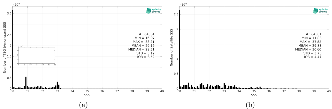
Figure 2: Histograms of SSS from TSG (Amundsen) (a) and SMAP SSS L2 v5 - 40 km (RSS) (b) considering all match-up pairs per bins of 0.1 over the Arctic Ocean Pi-MEP region and for the full satellite product period.
