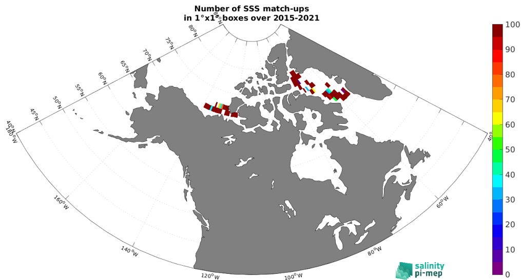
Figure 4: Number of SSS match-ups between TSG (Amundsen) SSS and the SMAP SSS L2 v5 - 40 km (RSS) SSS product for the Arctic Ocean Pi-MEP region over 1^\circ \times 1^\circ boxes and for the full satellite product period.
