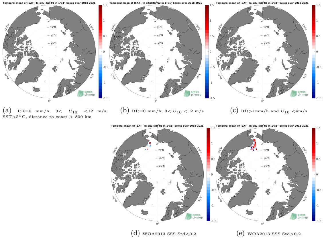
Figure 12: Temporal mean gridded over spatial boxes of size 1^{\circ}\times 1^{\circ} of \Delta\text{SSS} (SMAP SSS L2 v5 - 40 km (RSS) - SAILDRONE) for 5 different subdatasets corresponding to:RR=0 mm/h, 3 < U_{10} < 12 m/s, SST >5^{\circ}\text{C} , distance to coast > 800 km (a), RR=0 mm/h, 3 < U_{10} < 12 m/s (b), RR >1 mm/h and U_{10} < 4 m/s (c), WOA2013 SSS Std <0.2 (d), WOA2013 SSS Std >0.2 (e).
