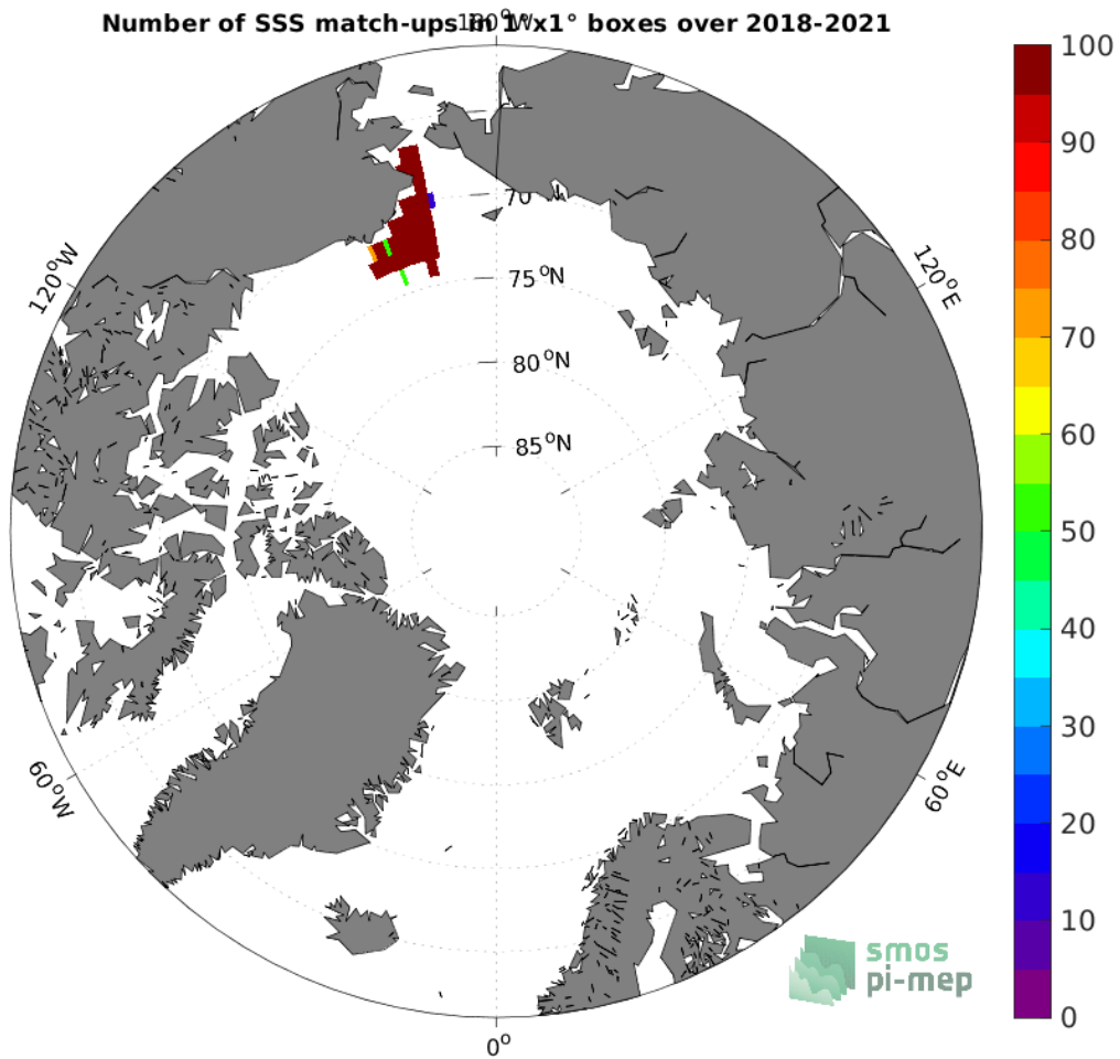
Figure 4: Number of SSS match-ups between Sairdrone SSS and the SMAP SSS L2 v5 - 40 km (RSS) SSS product for the Arctic Ocean Pi-MEP region over 1^{\circ} \times 1^{\circ} boxes and for the full satellite product period.
