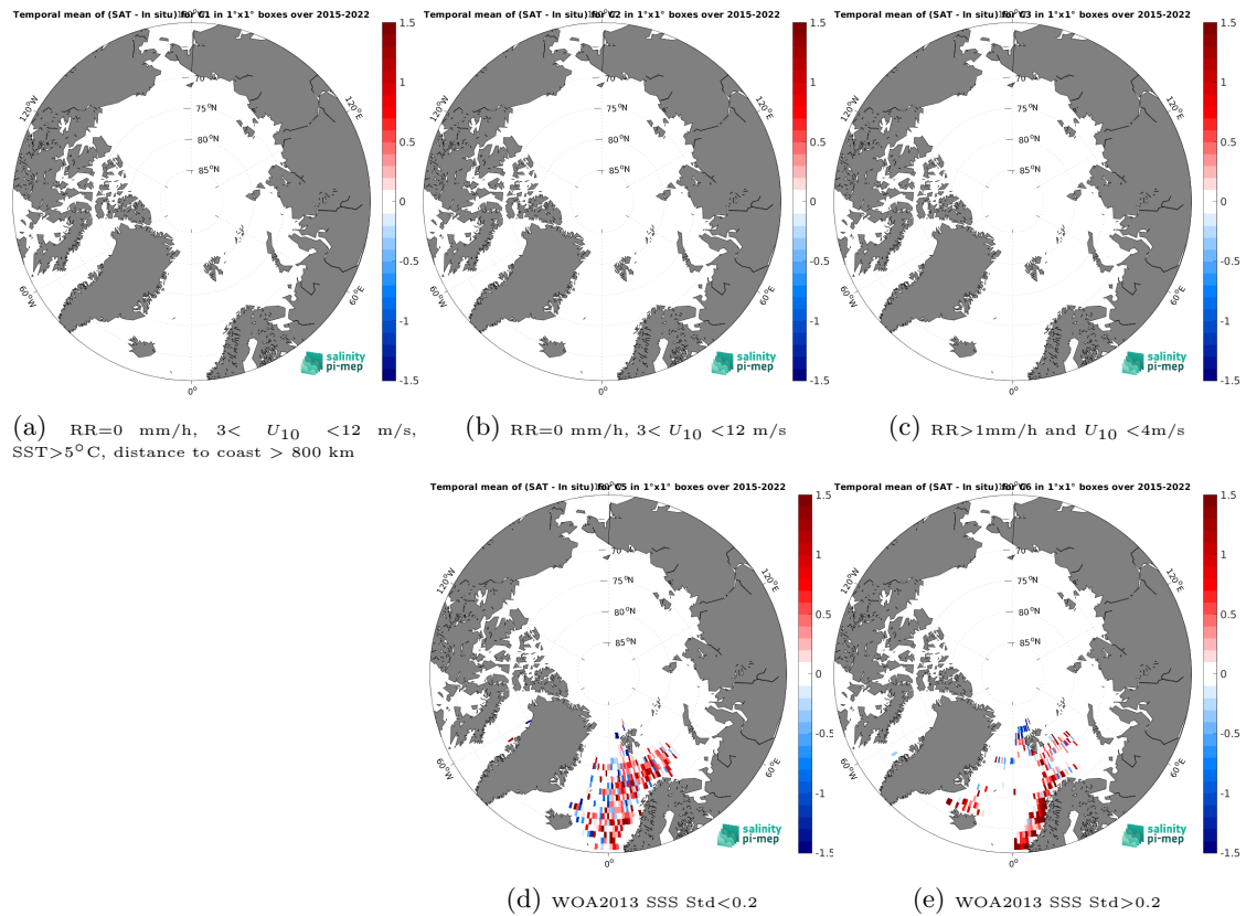
Figure 12: Temporal mean gridded over spatial boxes of size 1^{\circ}\times 1^{\circ} of \Delta\text{SSS} (SMAP SSS L2 v5 - 40 km (RSS) - ICES) for 5 different subdatasets corresponding to:RR=0 mm/h, 3 < U_{10} < 12 m/s, SST > 5^{\circ}\text{C} , distance to coast > 800 km (a), RR=0 mm/h, 3 < U_{10} < 12 m/s (b), RR > 1 mm/h and U_{10} < 4 m/s (c), WOA2013 SSS Std < 0.2 (d), WOA2013 SSS Std > 0.2 (e).
