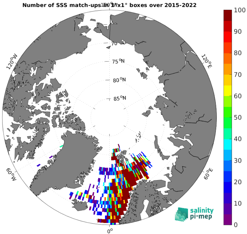
Figure 4: Number of SSS match-ups between ICES SSS and the SMAP SSS L2 v5 - 40 km (RSS) SSS product for the Arctic Ocean Pi-MEP region over 1^{\circ} \times 1^{\circ} boxes and for the full satellite product period.
