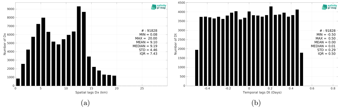
Figure 5: Histograms of the spatial (a) and temporal (b) lags between the location/time of the ICES measurement and the date of the corresponding SMAP SSS L2 v5 - 40 km (RSS) SSS pixel.
