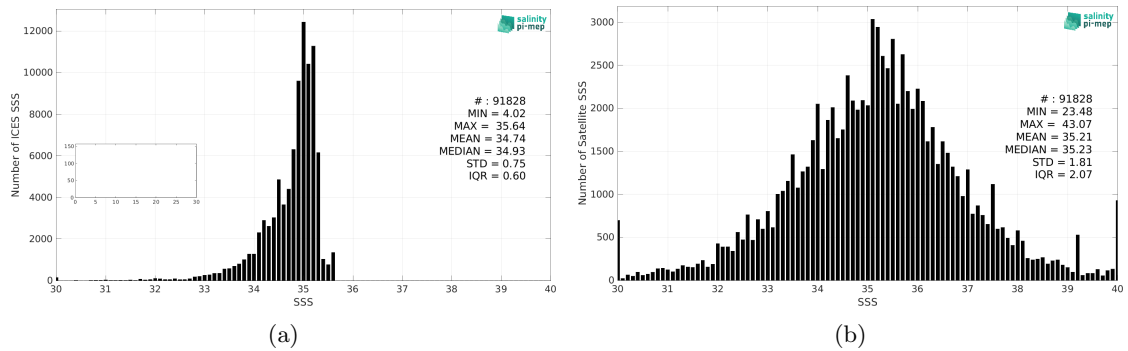
Figure 2: Histograms of SSS from ICES (a) and SMAP SSS L2 v5 - 40 km (RSS) (b) considering all match-up pairs per bins of 0.1 over the Arctic Ocean Pi-MEP region and for the full satellite product period.
