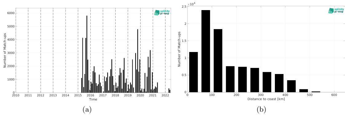
Figure 1: Number of match-ups between ICES and SMAP SSS L2 v5 - 40 km (RSS) SSS as a function of time (a) and as function of the distance to coast (b) over the Arctic Ocean Pi-MEP region and for the full satellite product period.
