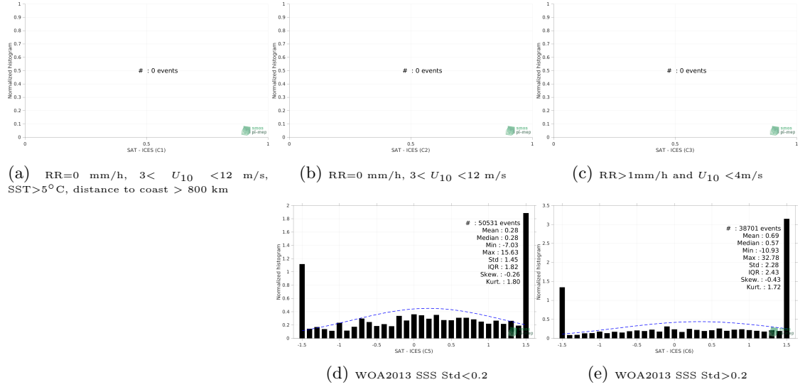
Figure 13: Normalized histogram of \Delta SSS (SMAP SSS L2 v5 - 40 km (RSS) - ICES) for 5 different subdatasets corresponding to: RR=0 mm/h, 3 < U_{10} < 12 m/s, SST>5°C, distance to coast > 800 km (a), RR=0 mm/h, 3 < U_{10} < 12 m/s (b), RR>1mm/h and U_{10} < 4 m/s (c), WOA2013 SSS Std<0.2 (d), WOA2013 SSS Std>0.2 (e).
