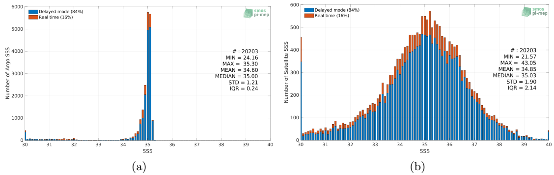
Figure 2: Histograms of SSS from Argo (a) and SMAP SSS L2 v5 - 40 km (RSS) (b) considering all match-up pairs per bins of 0.1 over the Arctic Ocean Pi-MEP region and for the full satellite product period.
