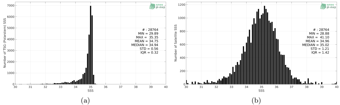
Figure 2: Histograms of SSS from TSG (Polarstern) (a) and SMAP SSS L2 v4 (RSS) (b) considering all match-up pairs per bins of 0.1 over the Arctic Ocean Pi-MEP region and for the full satellite product period.
