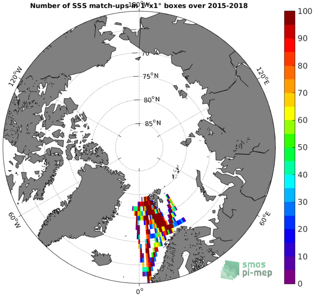
Figure 4: Number of SSS match-ups between TSG (Polarstern) SSS and the SMAP SSS L2 v4 (RSS) SSS product for the Arctic Ocean Pi-MEP region over 1°x1° boxes and for the full satellite product period.
