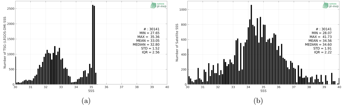
Figure 2: Histograms of SSS from TSG (LEGOS-DM) (a) and SMAP SSS L2 v4 (RSS) (b) considering all match-up pairs per bins of 0.1 over the Arctic Ocean Pi-MEP region and for the full satellite product period.
