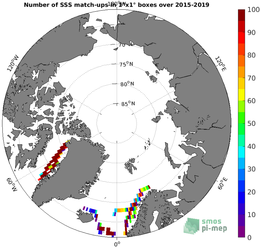
Figure 4: Number of SSS match-ups between TSG (LEGOS-DM) SSS and the SMAP SSS L2 v4 (RSS) SSS product for the Arctic Ocean Pi-MEP region over 1^\circ \times 1^\circ boxes and for the full satellite product period.
