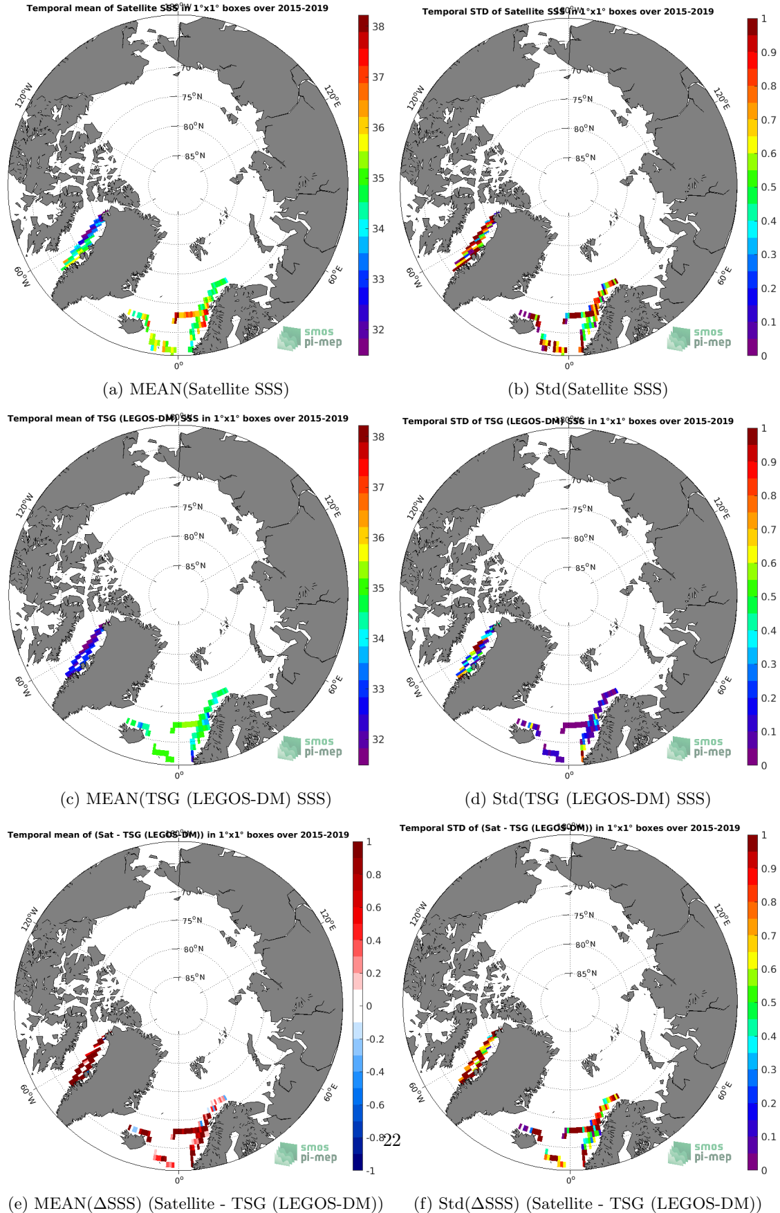
Figure 6: Temporal mean (left) and Std (right) of SSS from SMAP SSS L2 v4 (RSS) (top), TSG (LEGOS-DM) (middle), and of \Delta SSS (Satellite - TSG (LEGOS-DM)). Only match-up pairs are used to generate these maps.
