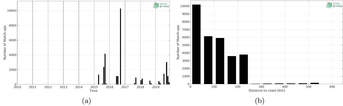
Figure 1: Number of match-ups between TSG (LEGOS-DM) and SMAP SSS L2 v4 (RSS) SSS as a function of time (a) and as function of the distance to coast (b) over the Arctic Ocean Pi-MEP region and for the full satellite product period.
