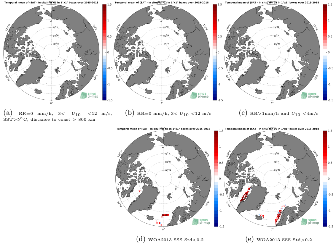
Figure 12: Temporal mean gridded over spatial boxes of size 1^{\circ}\times 1^{\circ} of \Delta\text{SSS} (SMAP-L2-RSS-V4 - TSG-LEGOS-DM) for 5 different subdatasets corresponding to: RR=0 mm/h, 3 < U_{10} < 12 m/s, SST > 5^{\circ}\text{C} , distance to coast > 800 km (a), RR=0 mm/h, 3 < U_{10} < 12 m/s (b), RR > 1 mm/h and U_{10} < 4 m/s (c), WOA2013 SSS Std < 0.2 (d), WOA2013 SSS Std > 0.2 (e).
