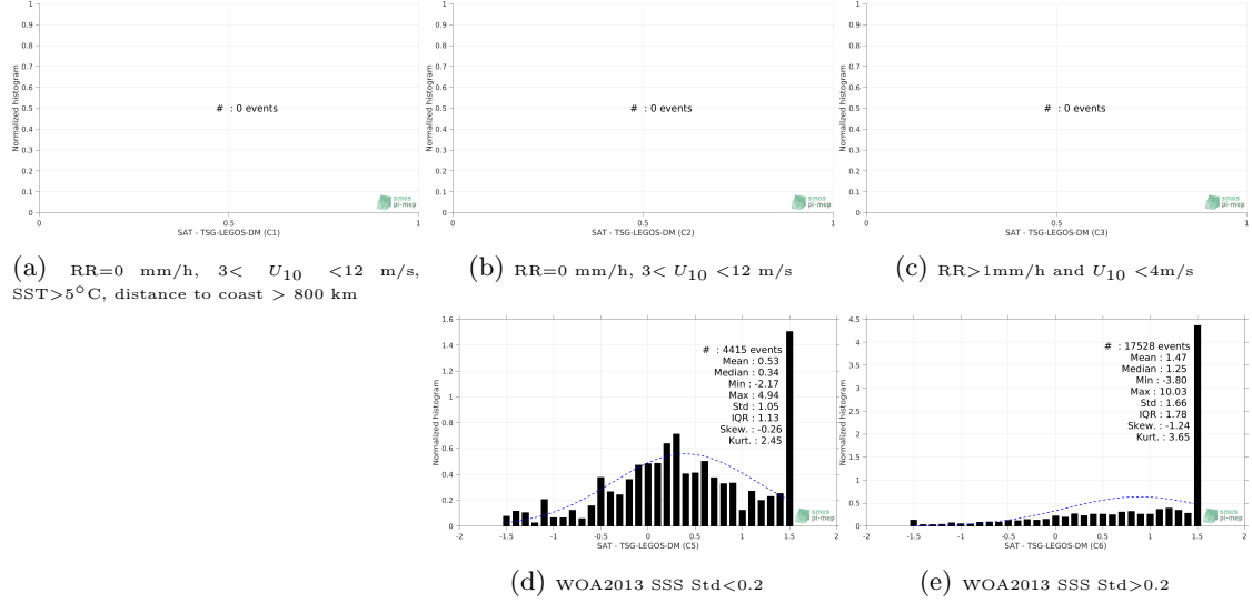
Figure 13: Normalized histogram of \Delta\text{SSS} (SMAP-L2-RSS-V4 - TSG-LEGOS-DM) for 5 different subdatasets corresponding to: RR=0 mm/h, 3 < U_{10} < 12 m/s, SST > 5^{\circ}\text{C} , distance to coast > 800 km (a), RR=0 mm/h, 3 < U_{10} < 12 m/s (b), RR > 1\text{mm/h} and U_{10} < 4\text{m/s} (c), WOA2013 SSS Std < 0.2 (d), WOA2013 SSS Std > 0.2 (e).
