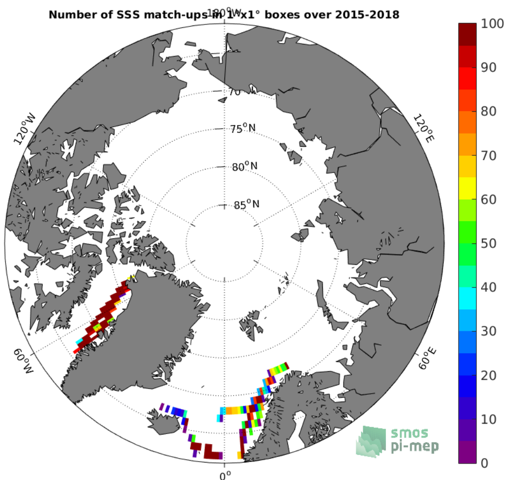
Figure 4: Number of SSS match-ups between TSG-LEGOS-DM SSS and the SMAP-L2-RSS-V4 SSS product for the Arctic Ocean Pi-MEP region over 1^\circ \times 1^\circ boxes and for the full satellite product period.
