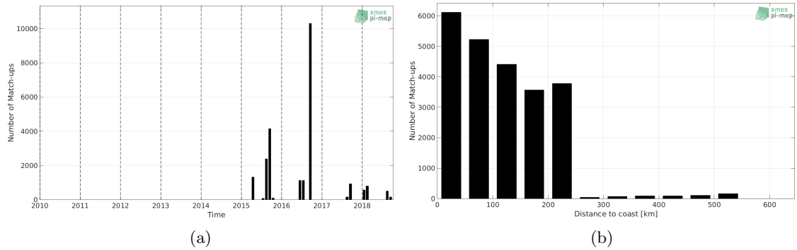
Figure 1: Number of match-ups between TSG-LEGOS-DM and SMAP-L2-RSS-V4 SSS as a function of time (a) and as function of the distance to coast (b) over the Arctic Ocean Pi-MEP region and for the full satellite product period.
