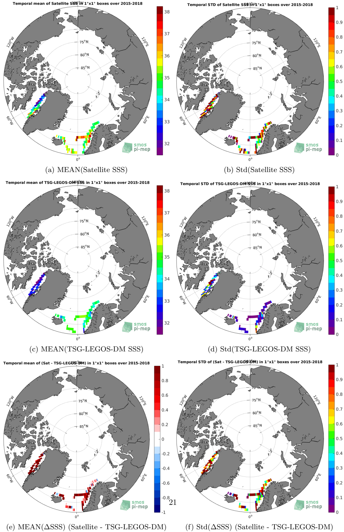
Figure 6: Temporal mean (left) and Std (right) of SSS from SMAP-L2-RSS-V4 (top), TSG-LEGOS-DM (middle), and of \Delta SSS (Satellite - TSG-LEGOS-DM). Only match-up pairs are used to generate these maps.
