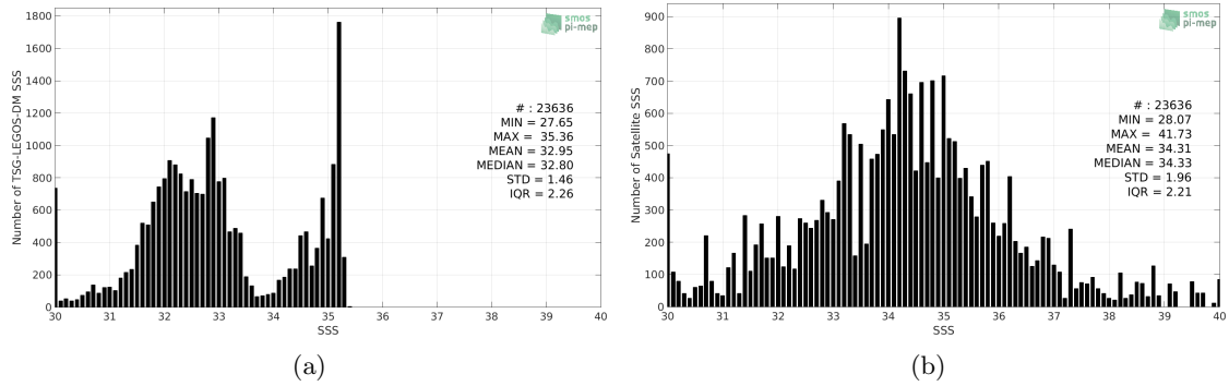
Figure 2: Histograms of SSS from TSG-LEGOS-DM (a) and SMAP-L2-RSS-V4 (b) considering all match-up pairs per bins of 0.1 over the Arctic Ocean Pi-MEP region and for the full satellite product period.
