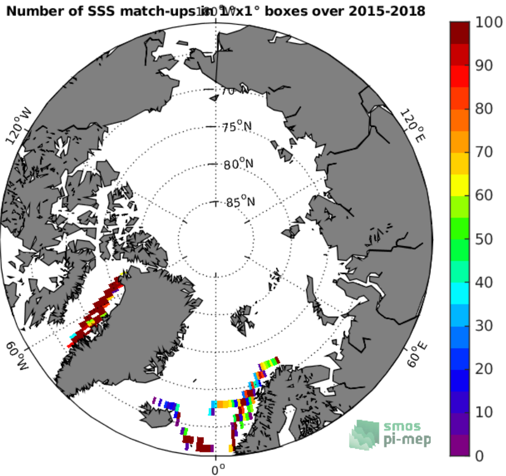
Figure 4: Number of SSS match-ups between TSG-LEGOS-DM SSS and the SMAP-L2-RSS-V4 SSS product for the Arctic Ocean Pi-MEP region over 1°x1° boxes and for the full satellite product period.
