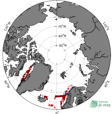
(e) MEAN( \Delta SSS) (Satellite - TSG-LEGOS-DM)
