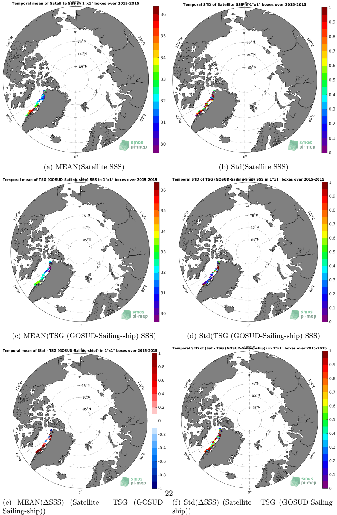
Figure 6: Temporal mean (left) and Std (right) of SSS from SMAP SSS L2 v4 (RSS) (top), TSG (GOSUD-Sailing-ship) (middle), and of \Delta SSS (Satellite - TSG (GOSUD-Sailing-ship)). Only match-up pairs are used to generate these maps.
