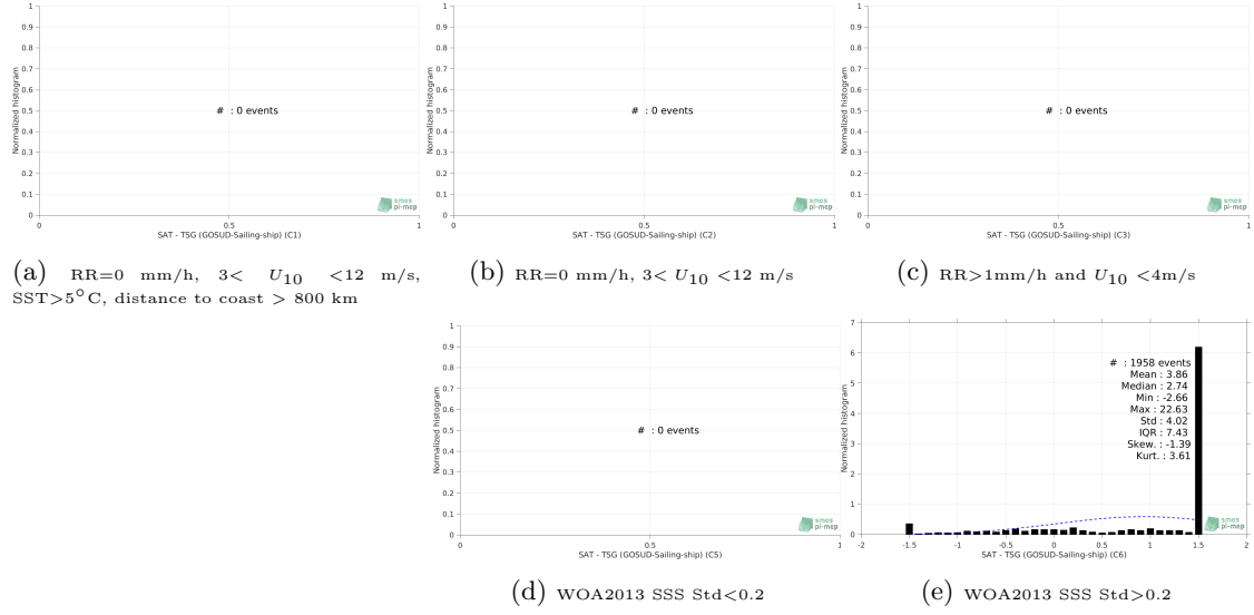
Figure 13: Normalized histogram of \Delta SSS (SMAP SSS L2 v4 (RSS) - TSG (GOSUD-Sailing-ship)) for 5 different subdatasets corresponding to: RR=0 mm/h, 3 < U_{10} < 12 m/s, SST >5^{\circ} C, distance to coast > 800 km (a), RR=0 mm/h, 3 < U_{10} < 12 m/s (b), RR >1 mm/h and U_{10} < 4 m/s (c), WOA2013 SSS Std <0.2 (d), WOA2013 SSS Std >0.2 (e).
