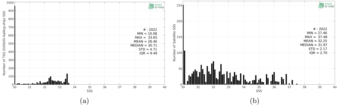
Figure 2: Histograms of SSS from TSG (GOSUD-Sailing-ship) (a) and SMAP SSS L2 v4 (RSS) (b) considering all match-up pairs per bins of 0.1 over the Arctic Ocean Pi-MEP region and for the full satellite product period.
