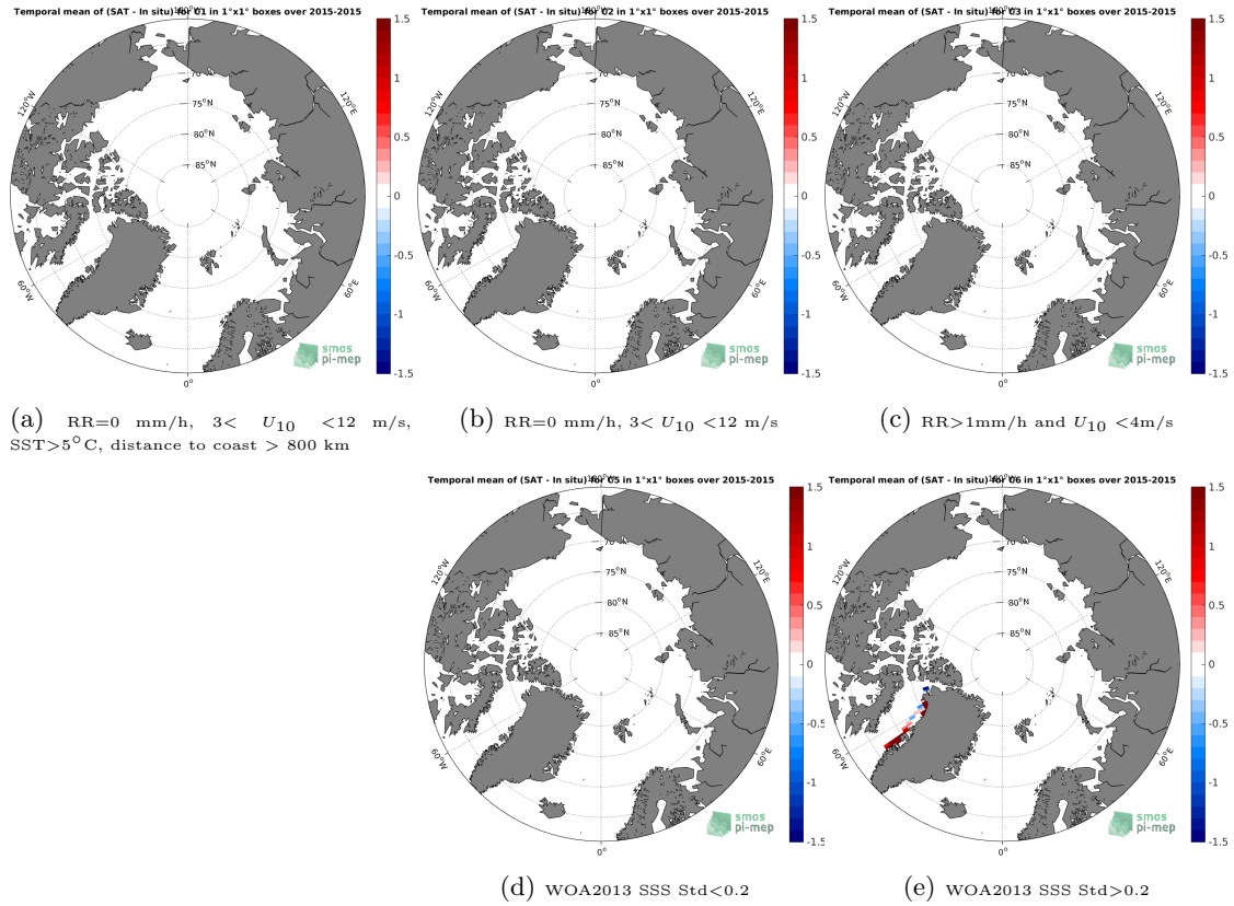
Figure 12: Temporal mean gridded over spatial boxes of size 1°x1° of \Delta SSS (SMAP SSS L2 v4 (RSS) - TSG (GOSUD-Sailing-ship)) for 5 different subdatasets corresponding to: RR=0 mm/h, 3 < U_{10} < 12 m/s, SST > 5°C, distance to coast > 800 km (a), RR=0 mm/h, 3 < U_{10} < 12 m/s (b), RR > 1mm/h and U_{10} < 4 m/s (c), WOA2013 SSS Std < 0.2 (d), WOA2013 SSS Std > 0.2 (e).
