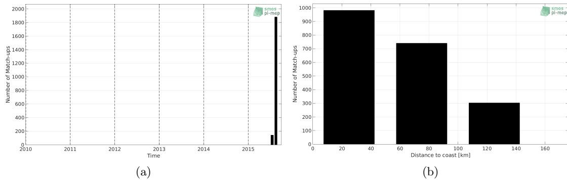
Figure 1: Number of match-ups between TSG (GOSUD-Sailing-ship) and SMAP SSS L2 v4 (RSS) SSS as a function of time (a) and as function of the distance to coast (b) over the Arctic Ocean Pi-MEP region and for the full satellite product period.
