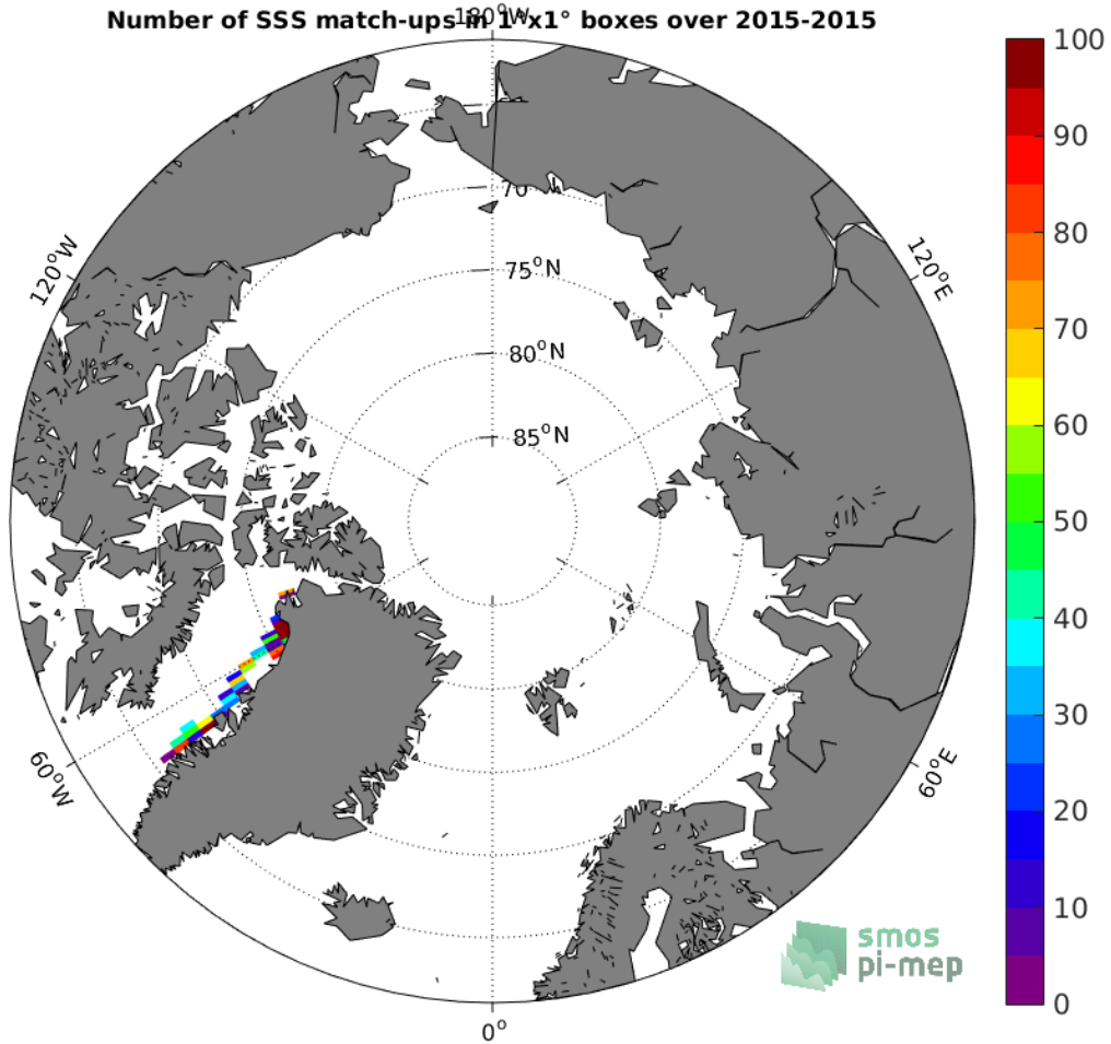
Figure 4: Number of SSS match-ups between TSG (GOSUD-Sailing-ship) SSS and the SMAP SSS L2 v4 (RSS) SSS product for the Arctic Ocean Pi-MEP region over 1°x1° boxes and for the full satellite product period.
