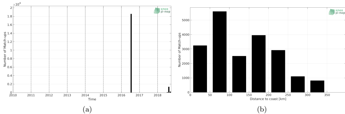
Figure 1: Number of match-ups between TSG (GOSUD-Research-vessel) and SMAP SSS L2 v4 (RSS) SSS as a function of time (a) and as function of the distance to coast (b) over the Arctic Ocean Pi-MEP region and for the full satellite product period.
