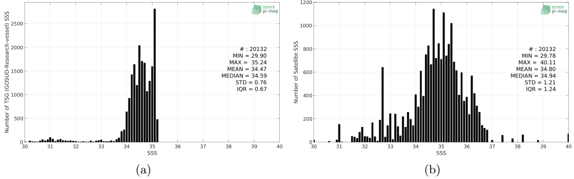
Figure 2: Histograms of SSS from TSG (GOSUD-Research-vessel) (a) and SMAP SSS L2 v4 (RSS) (b) considering all match-up pairs per bins of 0.1 over the Arctic Ocean Pi-MEP region and for the full satellite product period.
