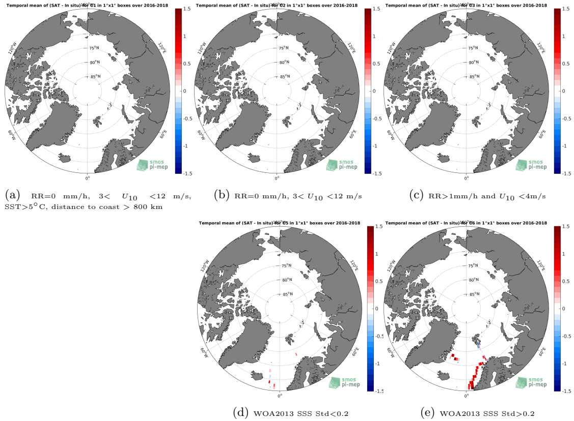
Figure 12: Temporal mean gridded over spatial boxes of size 1^\circ \times 1^\circ of \Delta SSS (SMAP SSS L2 v4 (RSS) - TSG (GOSUD-Research-vessel)) for 5 different subdatasets corresponding to: RR=0 mm/h, 3 < U_{10} < 12 m/s, SST > 5°C, distance to coast > 800 km (a), RR=0 mm/h, 3 < U_{10} < 12 m/s (b), RR > 1mm/h and U_{10} < 4 m/s (c), WOA2013 SSS Std < 0.2 (d), WOA2013 SSS Std > 0.2 (e).
