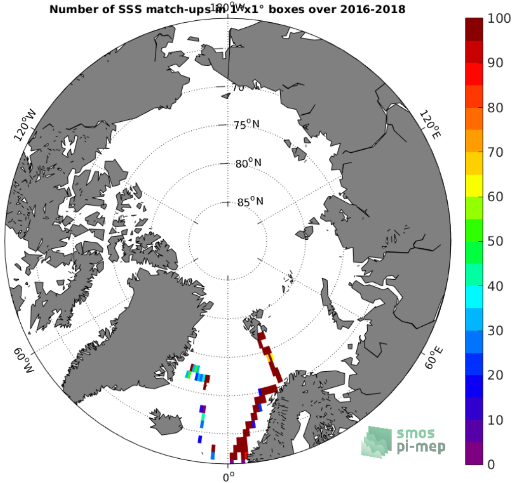
Figure 4: Number of SSS match-ups between TSG (GOSUD-Research-vessel) SSS and the SMAP SSS L2 v4 (RSS) SSS product for the Arctic Ocean Pi-MEP region over 1^\circ \times 1^\circ boxes and for the full satellite product period.
