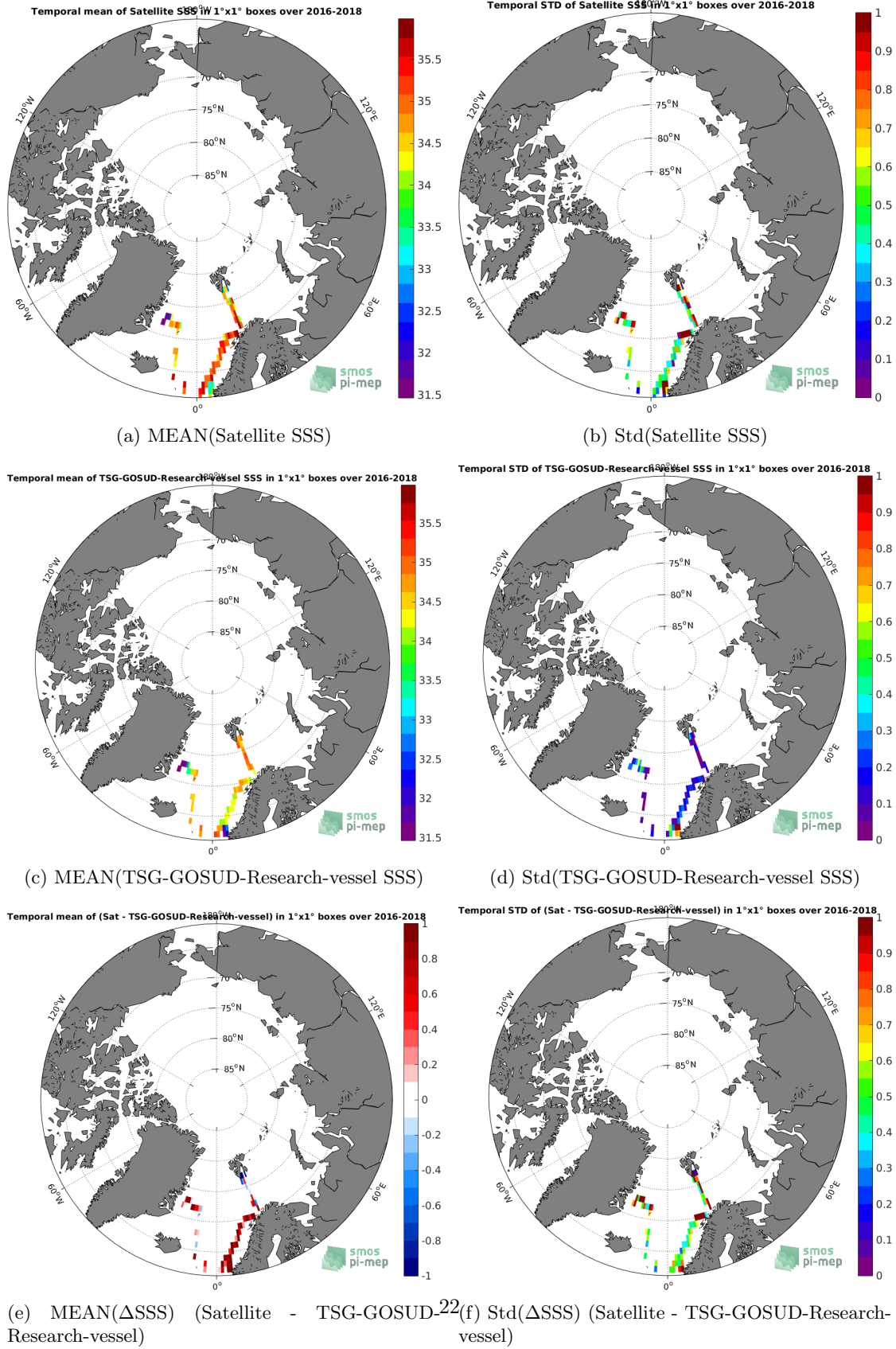
Figure 6: Temporal mean (left) and Std (right) of SSS from SMAP-L2-RSS-V4 (top), TSG-GOSUD-Research-vessel (middle), and of \Delta SSS (Satellite - TSG-GOSUD-Research-vessel). Only match-up pairs are used to generate these maps.
