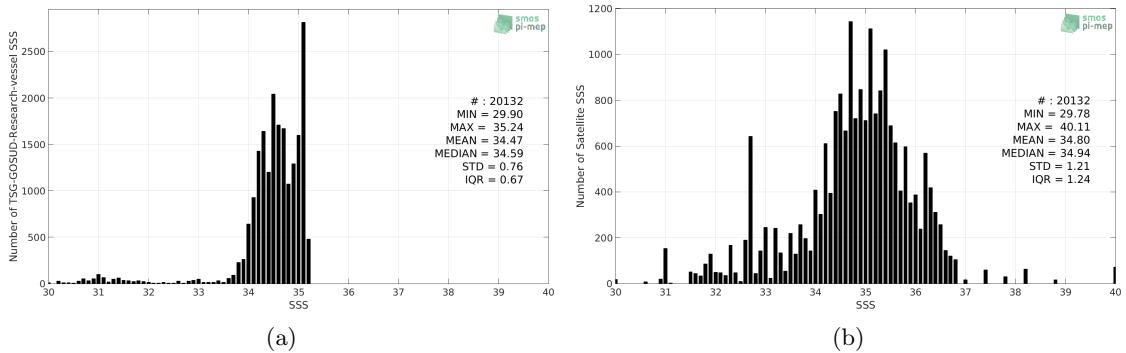
Figure 2: Histograms of SSS from TSG-GOSUD-Research-vessel (a) and SMAP-L2-RSS-V4 (b) considering all match-up pairs per bins of 0.1 over the Arctic Ocean Pi-MEP region and for the full satellite product period.
