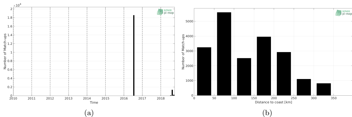
Figure 1: Number of match-ups between TSG-GOSUD-Research-vessel and SMAP-L2-RSS-V4 SSS as a function of time (a) and as function of the distance to coast (b) over the Arctic Ocean Pi-MEP region and for the full satellite product period.
