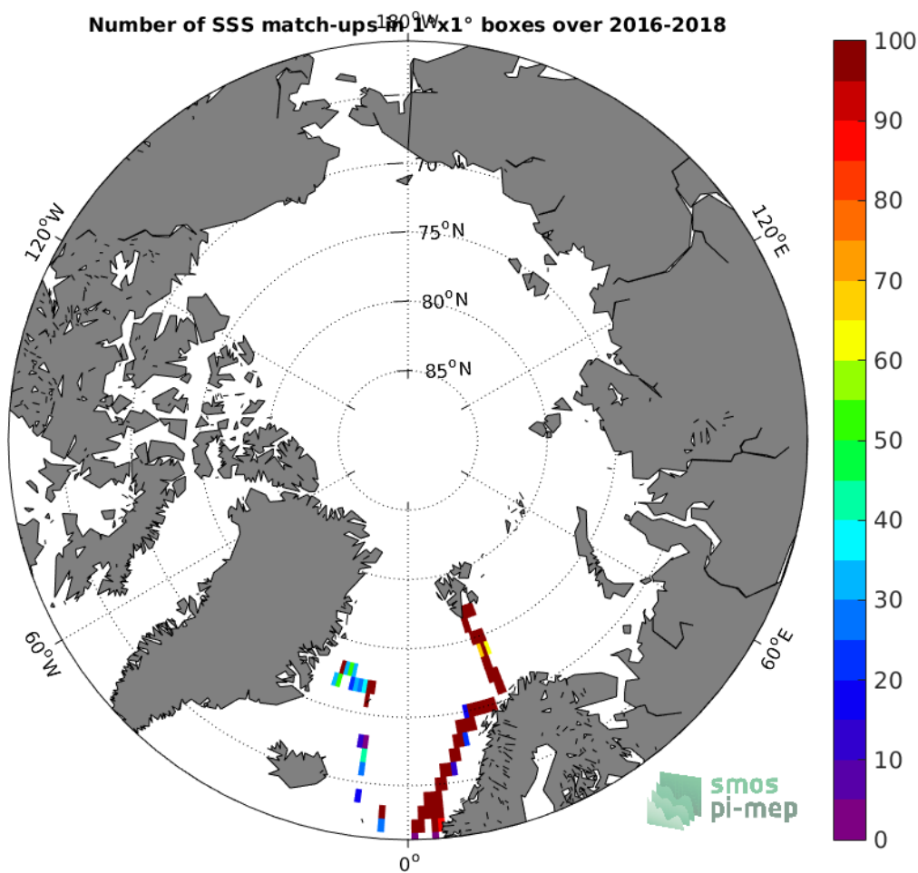
Figure 4: Number of SSS match-ups between TSG-GOSUD-Research-vessel SSS and the SMAP-L2-RSS-V4 SSS product for the Arctic Ocean Pi-MEP region over 1°x1° boxes and for the full satellite product period.
