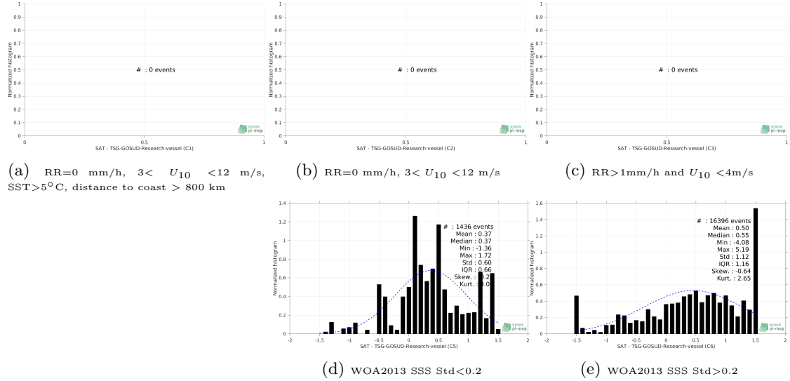
Figure 13: Normalized histogram of \Delta SSS (SMAP-L2-RSS-V4 - TSG-GOSUD-Research-vessel) for 5 different subdatasets corresponding to: RR=0 mm/h, 3 < U_{10} < 12 m/s, SST>5°C, distance to coast > 800 km (a), RR=0 mm/h, 3 < U_{10} < 12 m/s (b), RR>1mm/h and U_{10} < 4 m/s (c), WOA2013 SSS Std<0.2 (d), WOA2013 SSS Std>0.2 (e).
