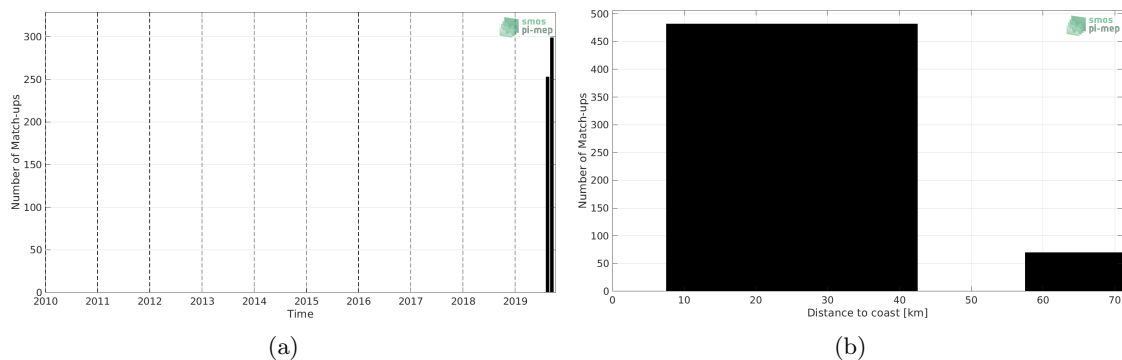
Figure 1: Number of match-ups between Surface drifters and SMAP SSS L2 v4 (RSS) SSS as a function of time (a) and as function of the distance to coast (b) over the Arctic Ocean Pi-MEP region and for the full satellite product period.
