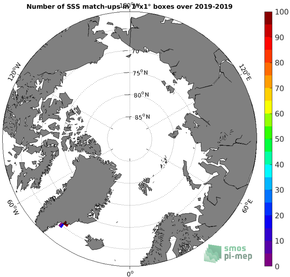
Figure 3: Number of SSS match-ups between Surface drifters SSS and the SMAP SSS L2 v4 (RSS) SSS product for the Arctic Ocean Pi-MEP region over 1°x1° boxes and for the full satellite product period.
