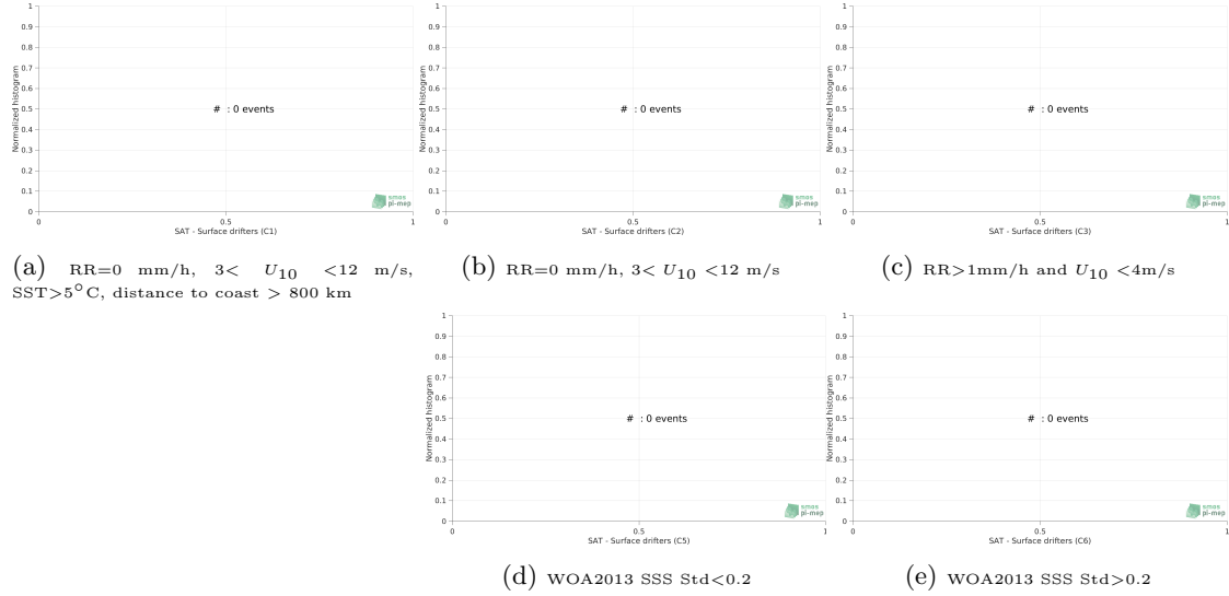
Figure 12: Normalized histogram of \Delta\text{SSS} (SMAP SSS L2 v4 (RSS) - Surface drifters) for 5 different subdatasets corresponding to: RR=0 mm/h, 3 < U_{10} < 12 m/s, SST > 5^\circ\text{C} , distance to coast > 800 km (a), RR=0 mm/h, 3 < U_{10} < 12 m/s (b), RR > 1 mm/h and U_{10} < 4 m/s (c), WOA2013 SSS Std < 0.2 (d), WOA2013 SSS Std > 0.2 (e).
