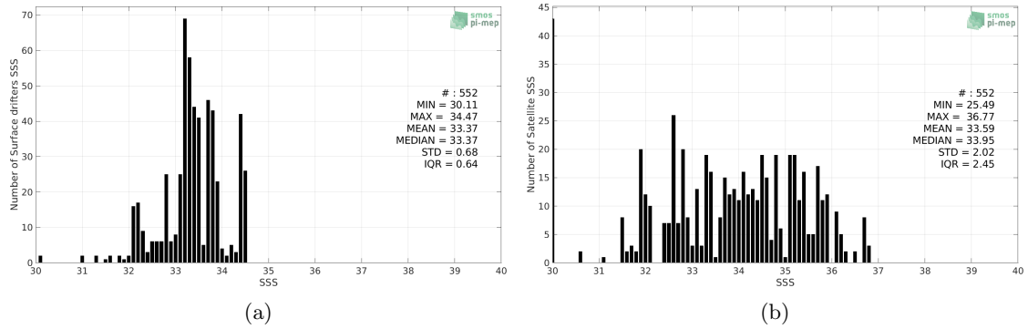
Figure 2: Histograms of SSS from Surface drifters (a) and SMAP SSS L2 v4 (RSS) (b) considering all match-up pairs per bins of 0.1 over the Arctic Ocean Pi-MEP region and for the full satellite product period.
