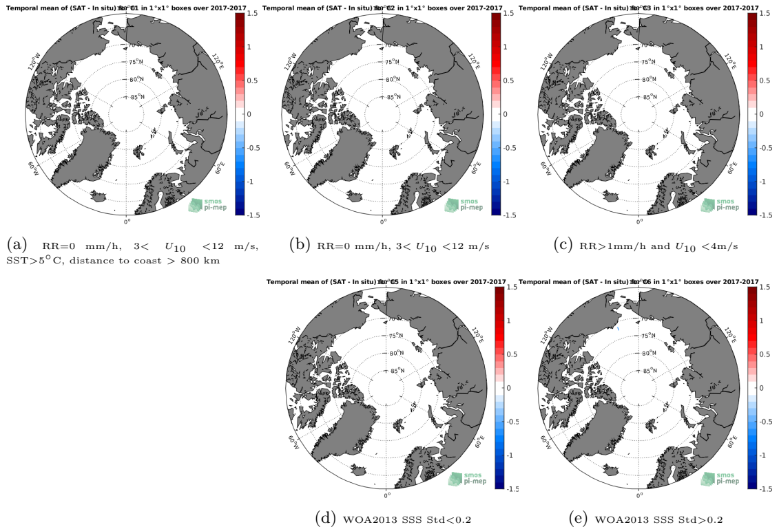
Figure 11: Temporal mean gridded over spatial boxes of size 1°x1° of \Delta SSS (SMAP-L2-RSS-V4 - Surface drifters) for 5 different subdatasets corresponding to: RR=0 mm/h, 3 < U_{10} < 12 m/s, SST > 5°C, distance to coast > 800 km (a), RR=0 mm/h, 3 < U_{10} < 12 m/s (b), RR > 1mm/h and U_{10} < 4m/s (c), WOA2013 SSS Std < 0.2 (d), WOA2013 SSS Std > 0.2 (e).
