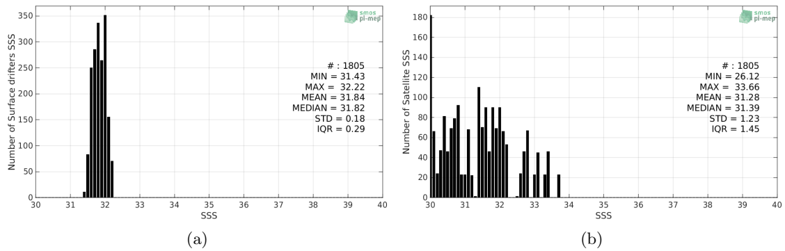
Figure 2: Histograms of SSS from Surface drifters (a) and SMAP-L2-RSS-V4 (b) considering all match-up pairs per bins of 0.1 over the Arctic Ocean Pi-MEP region and for the full satellite product period.
