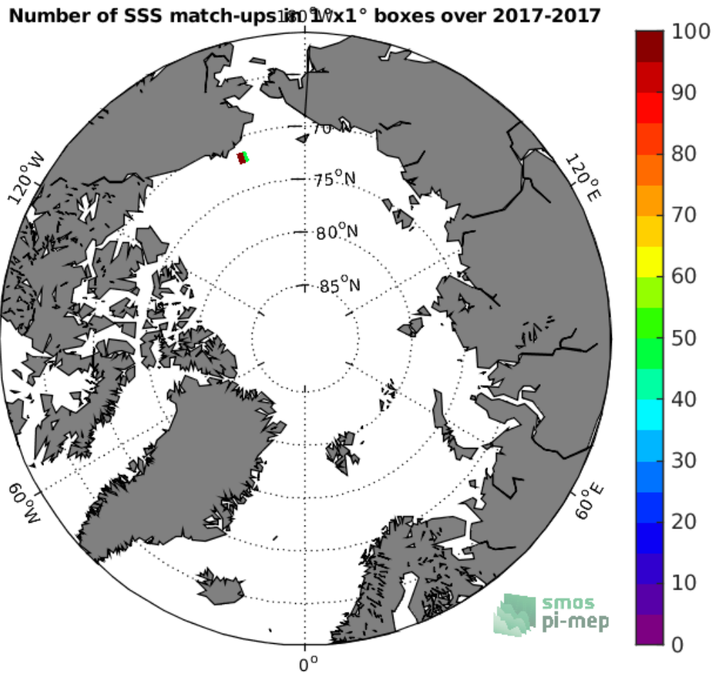
Figure 3: Number of SSS match-ups between Surface drifters SSS and the SMAP-L2-RSS-V4 SSS product for the Arctic Ocean Pi-MEP region over 1°x1° boxes and for the full satellite product period.
