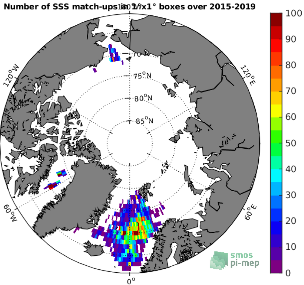
Figure 4: Number of SSS match-ups between Argo SSS and the SMAP-L2-RSS-V4 SSS product for the Arctic Ocean Pi-MEP region over 1^\circ \times 1^\circ boxes and for the full satellite product period.
