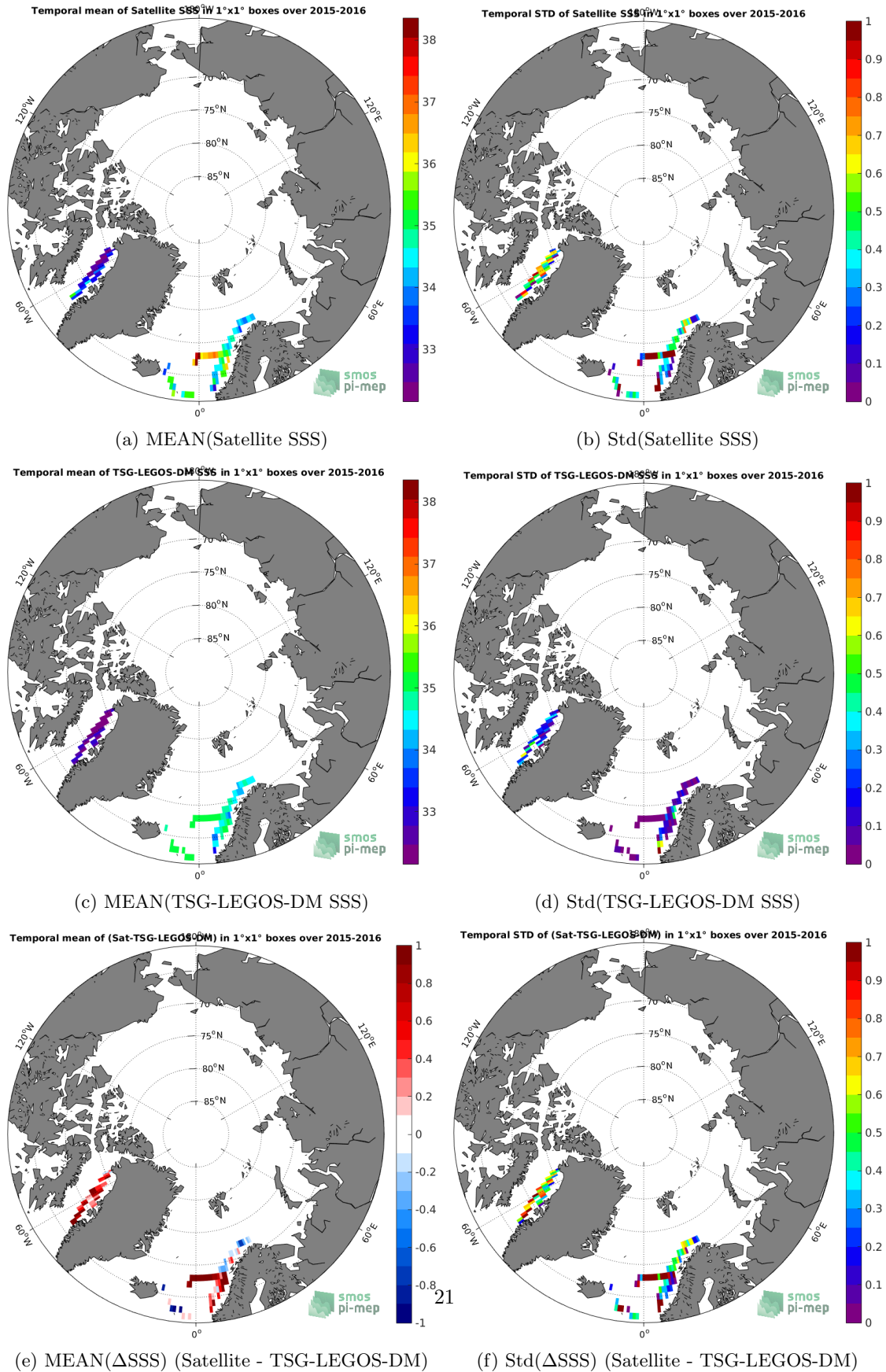
Figure 6: Temporal mean (left) and Std (right) of SSS from SMAP-L2-RSS-V3-70KM (top), TSG-LEGOS-DM (middle), and of \Delta SSS (Satellite - TSG-LEGOS-DM). Only match-up pairs are used to generate these maps.
