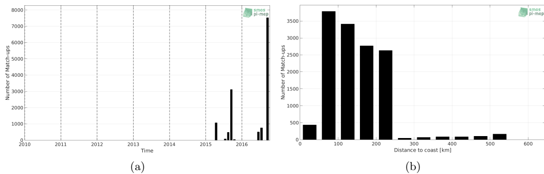
Figure 1: Number of match-ups between TSG-LEGOS-DM and SMAP-L2-RSS-V3-70KM SSS as a function of time (a) and as function of the distance to coast (b) over the Arctic Ocean Pi-MEP region and for the full satellite product period.
