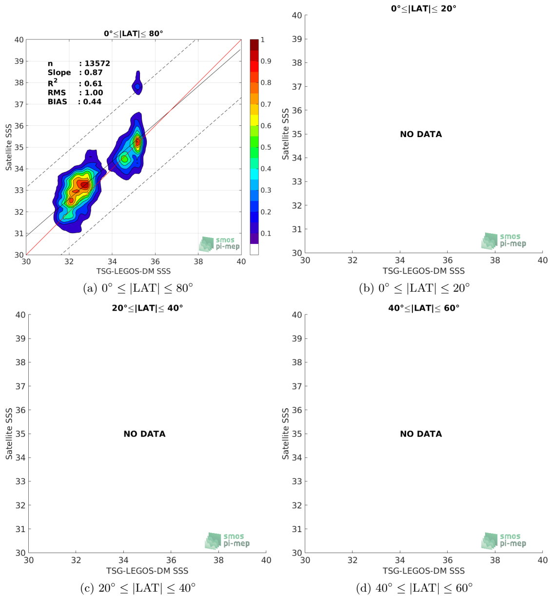
Figure 9: Contour maps of the concentration of SMAP-L2-RSS-V3-70KM SSS (y-axis) versus TSG-LEGOS-DM SSS (x-axis) at match-up pairs for different latitude bands. For each plot, the red line shows x=y . The black thin and dashed lines indicate a linear fit through the data cloud and the \pm 95\% confidence levels, respectively. The number match-up pairs n , the slope and R^2 coefficient of the linear fit, the root mean square (RMS) and the mean bias between satellite and in situ data are indicated for each latitude band in each plots.
