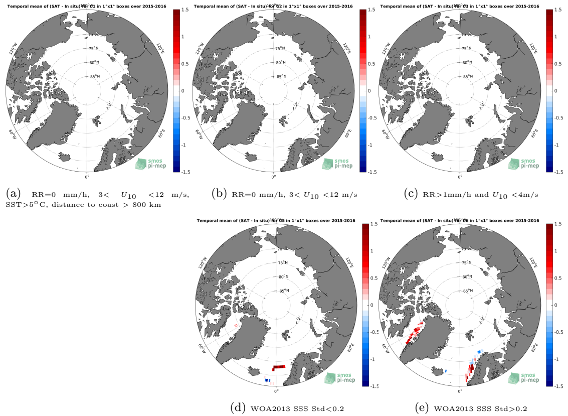
Figure 12: Temporal mean gridded over spatial boxes of size 1^\circ \times 1^\circ of \Delta SSS (SMAP-L2-RSS-V3-70KM - TSG-LEGOS-DM) for 5 different subdatasets corresponding to:RR=0 mm/h, 3 < U_{10} < 12 m/s, SST >5^\circ C, distance to coast > 800 km (a), RR=0 mm/h, 3 < U_{10} < 12 m/s (b), RR >1 mm/h and U_{10} < 4 m/s (c), WOA2013 SSS Std <0.2 (d), WOA2013 SSS Std >0.2 (e).
