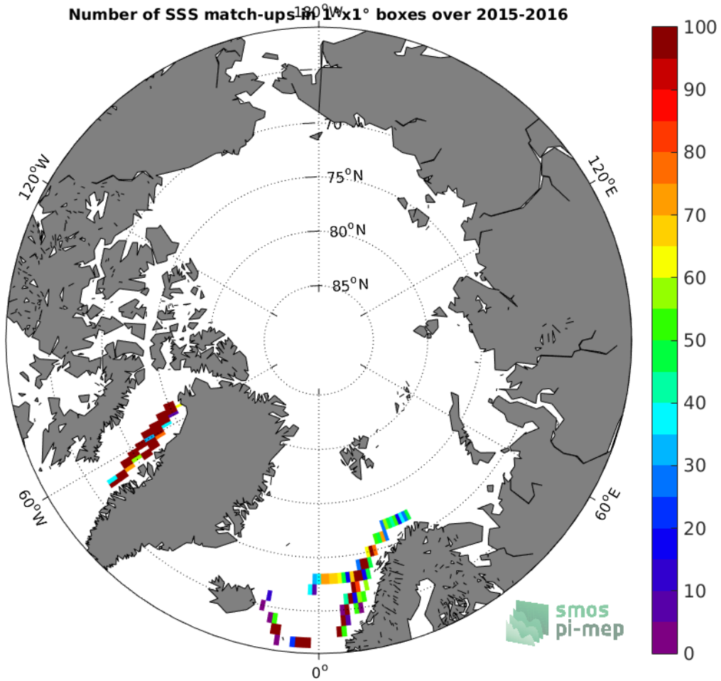
Figure 4: Number of SSS match-ups between TSG-LEGOS-DM SSS and the SMAP-L2-RSS-V3-70KM SSS product for the Arctic Ocean Pi-MEP region over 1^\circ \times 1^\circ boxes and for the full satellite product period.
