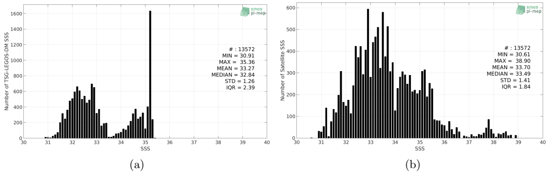
Figure 2: Histograms of SSS from TSG-LEGOS-DM (a) and SMAP-L2-RSS-V3-70KM (b) considering all match-up pairs per bins of 0.1 over the Arctic Ocean Pi-MEP region and for the full satellite product period.
