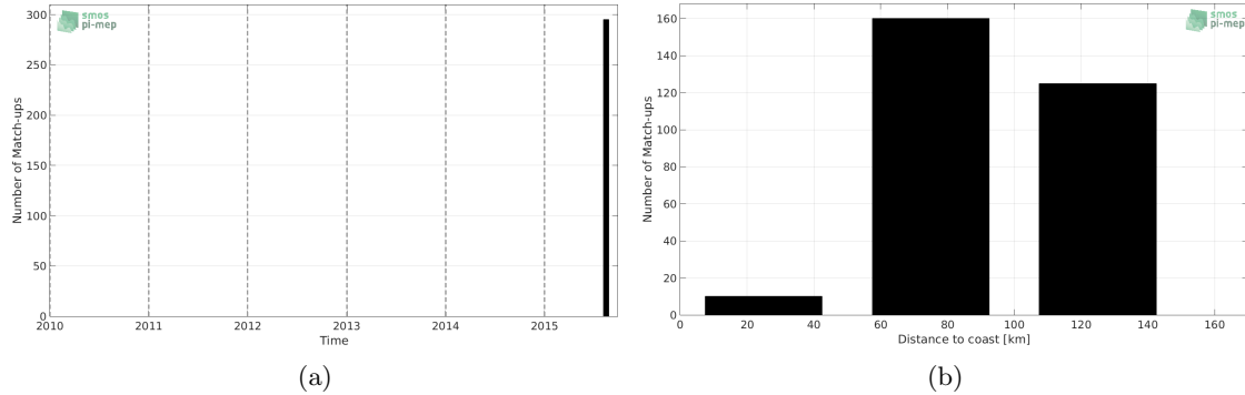
Figure 1: Number of match-ups between TSG-GOSUD-Sailing-ship and SMAP-L2-RSS-V3-70KM SSS as a function of time (a) and as function of the distance to coast (b) over the Arctic Ocean Pi-MEP region and for the full satellite product period.
