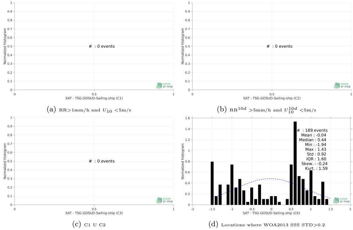
Figure 13: Normalized histogram of \Delta SSS (SMAP-L2-RSS-V3-70KM - TSG-GOSUD-Sailing-ship) for 6 different subdatasets corresponding to: RR > 1\text{mm/h} and U_{10} < 5\text{m/s} (a), RR^{10d} > 5\text{mm/h} and U_{10}^{10d} < 5\text{m/s} (b), C1 \cup C2 (c), Locations where WOA2013 SSS STD > 0.2 (d).
