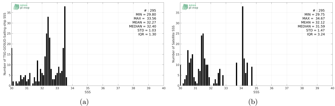
Figure 2: Histograms of SSS from TSG-GOSUD-Sailing-ship (a) and SMAP-L2-RSS-V3-70KM (b) considering all match-up pairs per bins of 0.1 over the Arctic Ocean Pi-MEP region and for the full satellite product period.
