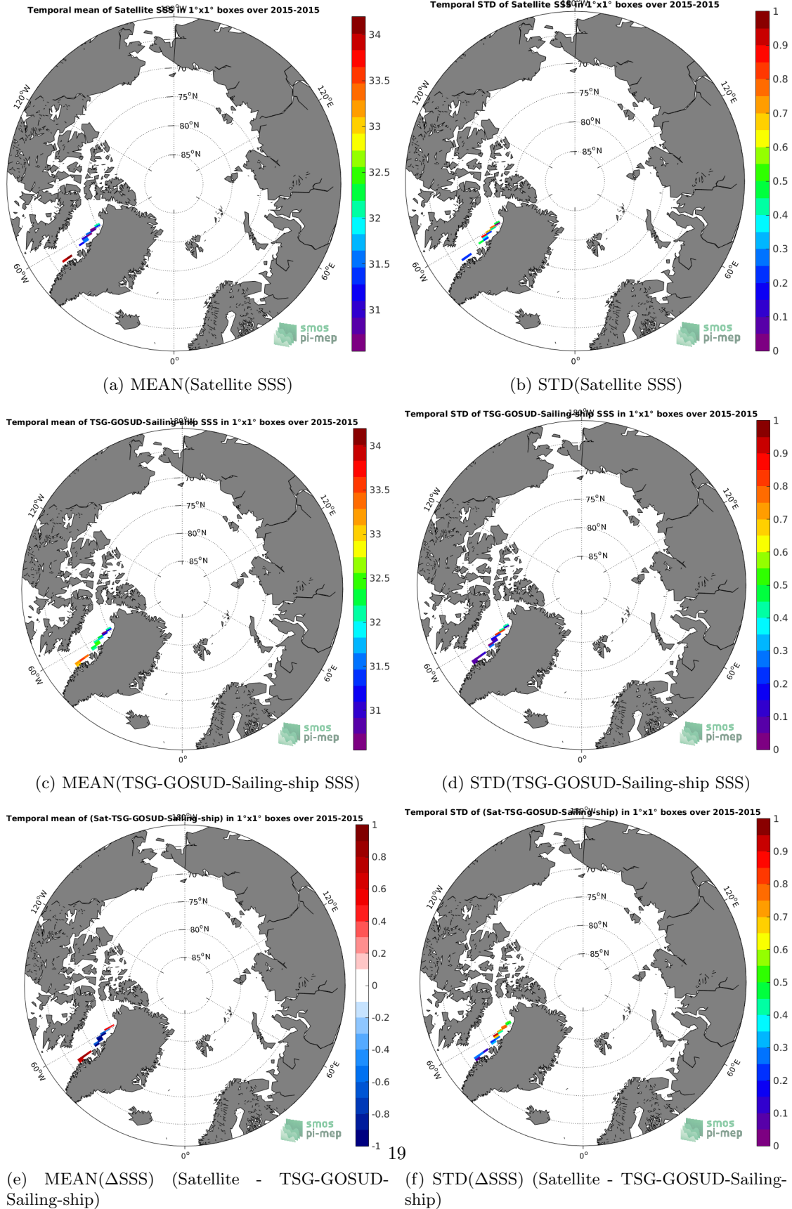
Figure 6: Temporal mean (left) and STD (right) of SSS from SMAP-L2-RSS-V3-70KM (top), TSG-GOSUD-Sailing-ship (middle), and of \Delta SSS (Satellite - TSG-GOSUD-Sailing-ship). Only match-up pairs are used to generate these maps.
