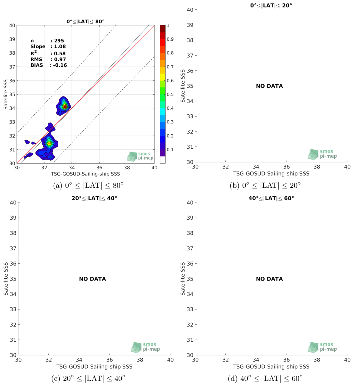
Figure 9: Contour maps of the concentration of SMAP-L2-RSS-V3-70KM SSS (y-axis) versus TSG-GOSUD-Sailing-ship SSS (x-axis) at match-up pairs for different latitude bands. For each plot, the red line shows x=y . The black thin and dashed lines indicate a linear fit through the data cloud and the \pm 95\% confidence levels, respectively. The number match-up pairs n , the slope and R^2 coefficient of the linear fit, the root mean square (RMS) and the mean bias between satellite and in situ data are indicated for each latitude band in each plots.
