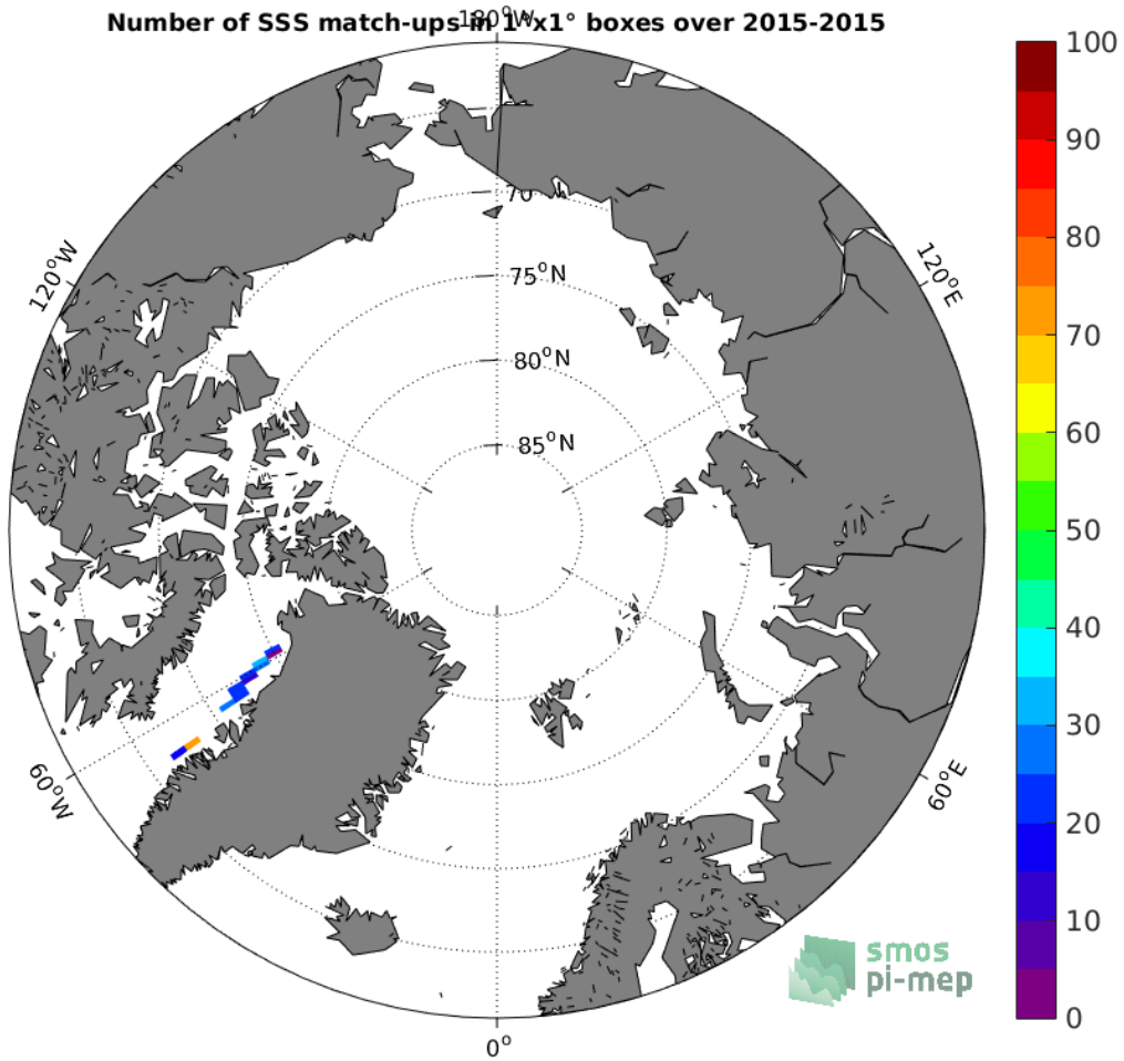
Figure 4: Number of SSS match-ups between TSG-GOSUD-Sailing-ship SSS and the SMAP-L2-RSS-V3-70KM SSS product for the Arctic Ocean Pi-MEP region over 1°x1° boxes and for the full satellite product period.
