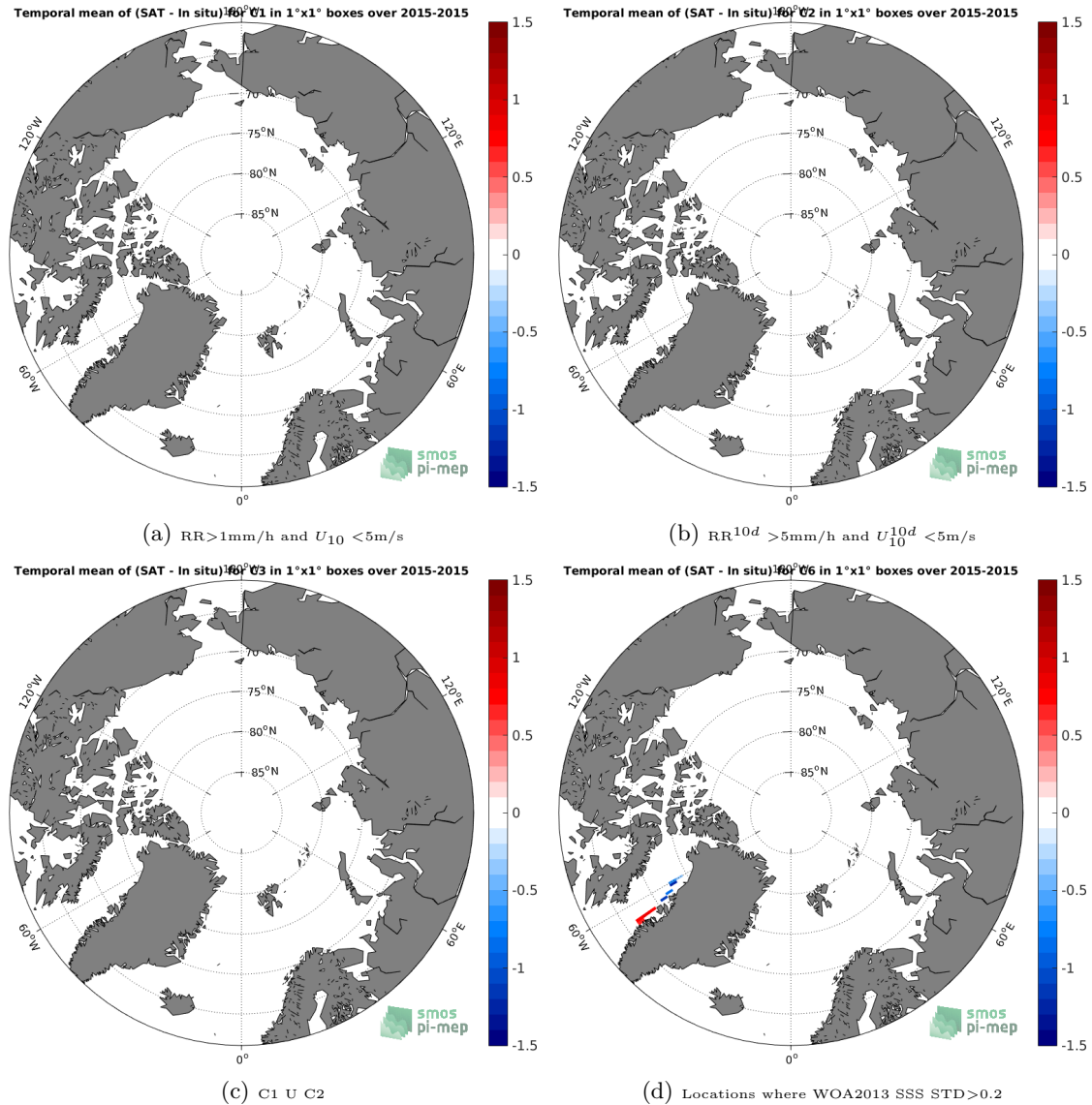
Figure 12: Temporal mean gridded over spatial boxes of size 1^\circ \times 1^\circ of \Delta SSS (SMAP-L2-RSS-V3-70KM - TSG-GOSUD-Sailing-ship) for 4 different subdatasets corresponding to:RR > 1mm/h and U_{10} < 5\text{m/s} (a), RR 10d > 5mm/h and U_{10}^{10d} < 5\text{m/s} (b), C1 U C2 (c),Locations where WOA2013 SSS STD > 0.2 (d).
