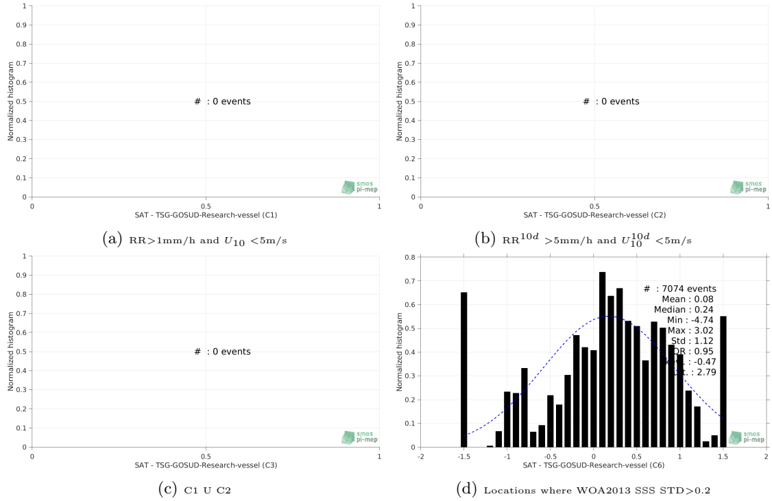
Figure 13: Normalized histogram of \Delta SSS (SMAP-L2-RSS-V3-70KM - TSG-GOSUD-Research-vessel) for 6 different subdatasets corresponding to: RR > 1\text{mm/h} and U_{10} < 5\text{m/s} (a), RR^{10d} > 5\text{mm/h} and U_{10}^{10d} < 5\text{m/s} (b), C1 \cup C2 (c), Locations where WOA2013 SSS STD > 0.2 (d).
