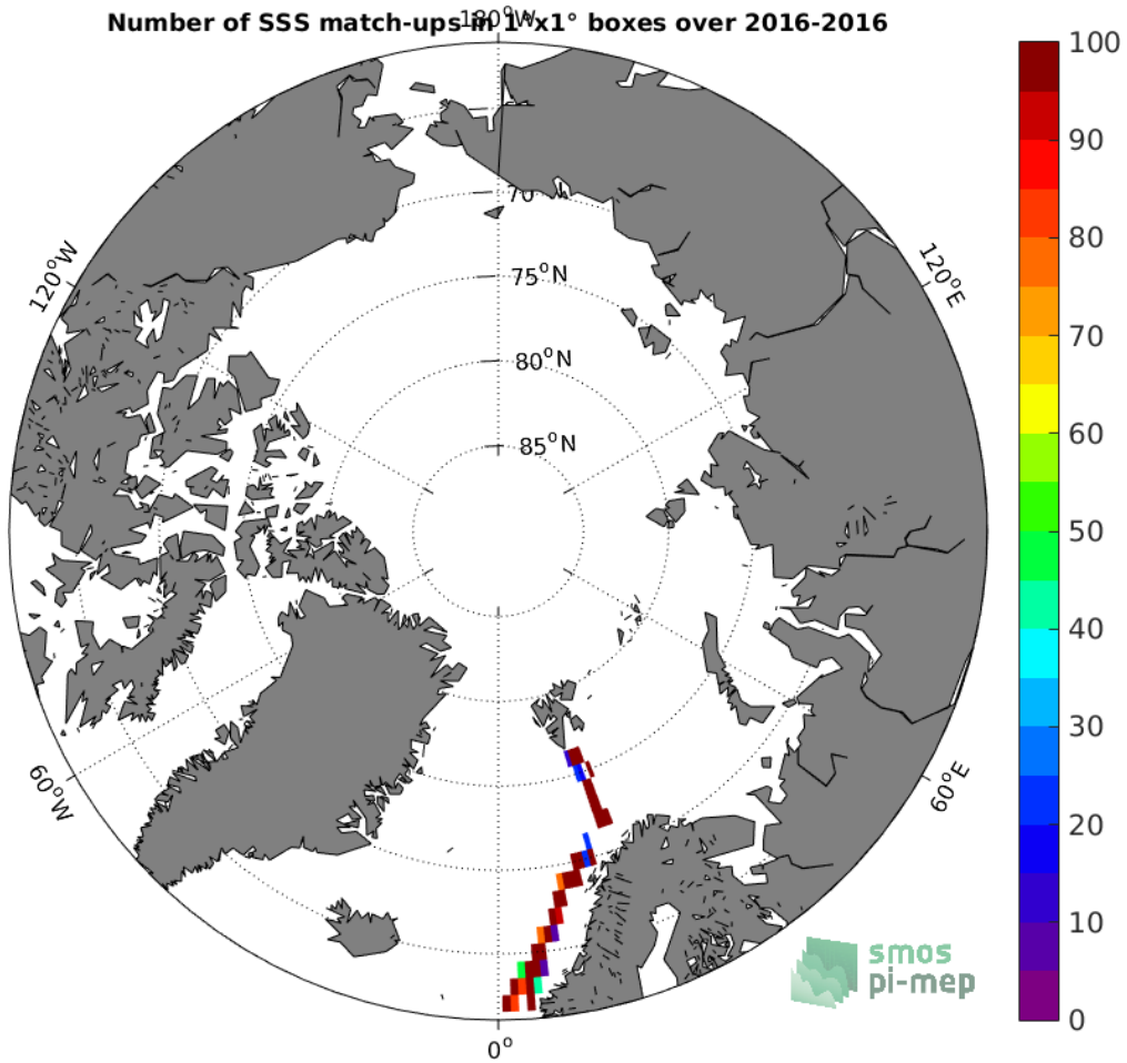
Figure 4: Number of SSS match-ups between TSG-GOSUD-Research-vessel SSS and the SMAP-L2-RSS-V3-70KM SSS product for the Arctic Ocean Pi-MEP region over 1°x1° boxes and for the full satellite product period.
