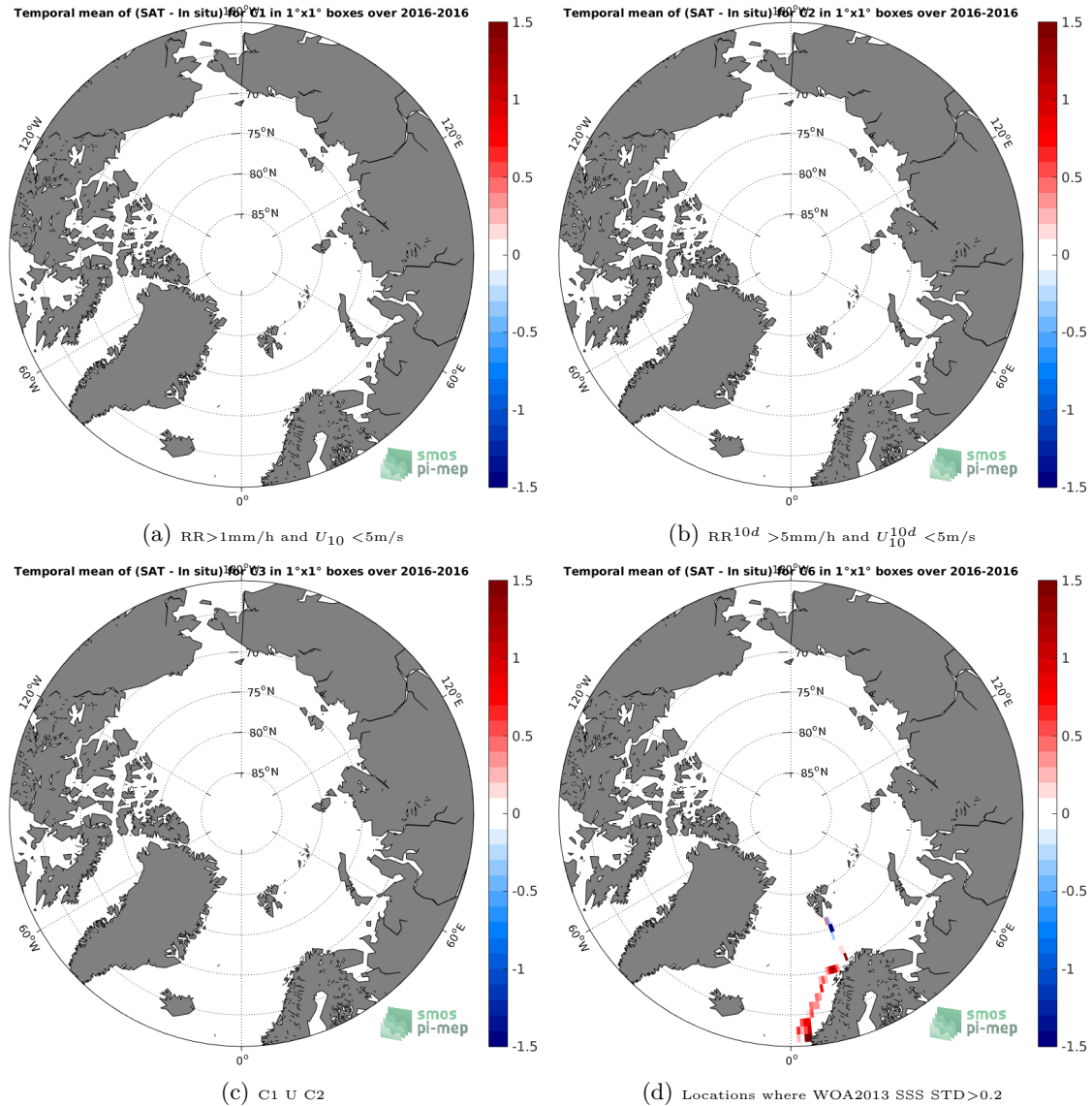
Figure 12: Temporal mean gridded over spatial boxes of size 1^\circ \times 1^\circ of \Delta SSS (SMAP-L2-RSS-V3-70KM - TSG-GOSUD-Research-vessel) for 4 different subdatasets corresponding to: RR > 1\text{mm/h} and U_{10} < 5\text{m/s} (a), RR^{10d} > 5\text{mm/h} and U_{10}^{10d} < 5\text{m/s} (b), C1 U C2 (c), Locations where WOA2013 SSS STD > 0.2 (d).
