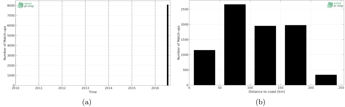
Figure 1: Number of match-ups between TSG-GOSUD-Research-vessel and SMAP-L2-RSS-V3-70KM SSS as a function of time (a) and as function of the distance to coast (b) over the Arctic Ocean Pi-MEP region and for the full satellite product period.
