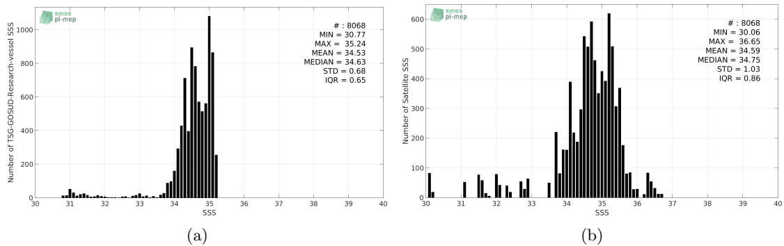
Figure 2: Histograms of SSS from TSG-GOSUD-Research-vessel (a) and SMAP-L2-RSS-V3-70KM (b) considering all match-up pairs per bins of 0.1 over the Arctic Ocean Pi-MEP region and for the full satellite product period.
