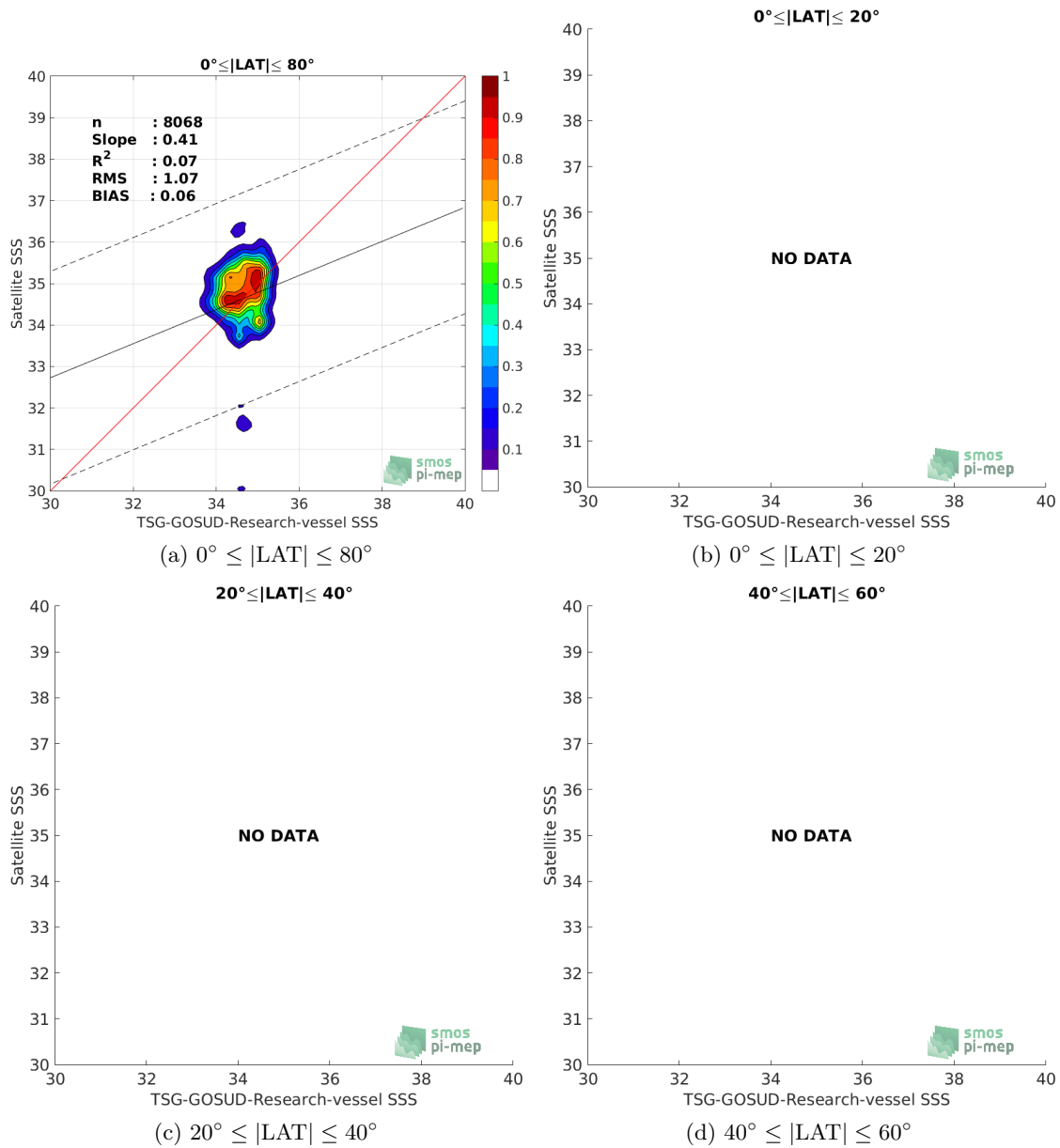
Figure 9: Contour maps of the concentration of SMAP-L2-RSS-V3-70KM SSS (y-axis) versus TSG-GOSUD-Research-vessel SSS (x-axis) at match-up pairs for different latitude bands. For each plot, the red line shows x=y . The black thin and dashed lines indicate a linear fit through the data cloud and the \pm 95\% confidence levels, respectively. The number match-up pairs n , the slope and R^2 coefficient of the linear fit, the root mean square (RMS) and the mean bias between satellite and in situ data are indicated for each latitude band in each plots.
