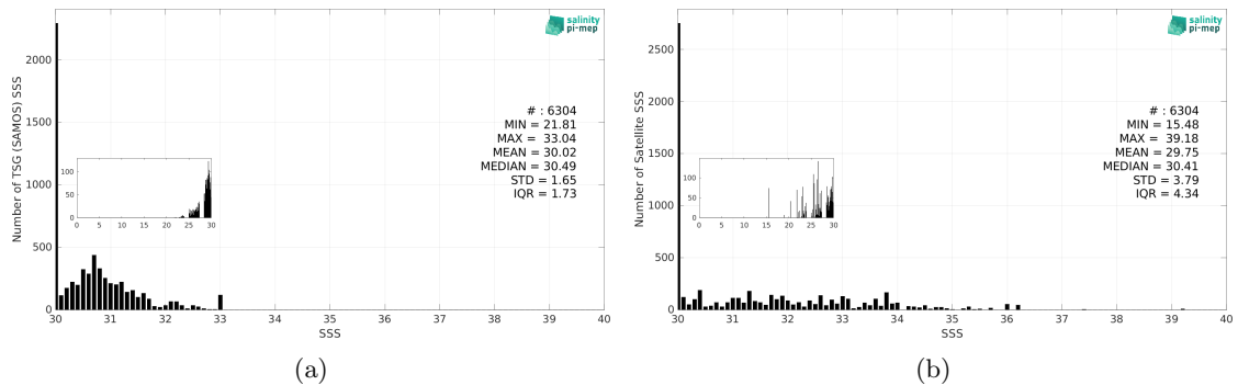
Figure 3: Histograms of SSS from TSG (SAMOS) (a) and SMAP SSS L2 v5.0 (JPL) (b) considering all match-up pairs per bins of 0.1 over the Arctic Ocean Pi-MEP region and for the full satellite product period.
