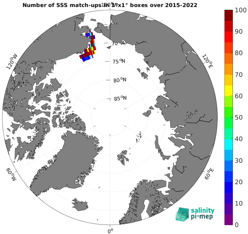
Figure 5: Number of SSS match-ups between TSG (SAMOS) SSS and the SMAP SSS L2 v5.0 (JPL) SSS product for the Arctic Ocean Pi-MEP region over 1^\circ \times 1^\circ boxes and for the full satellite product period.
