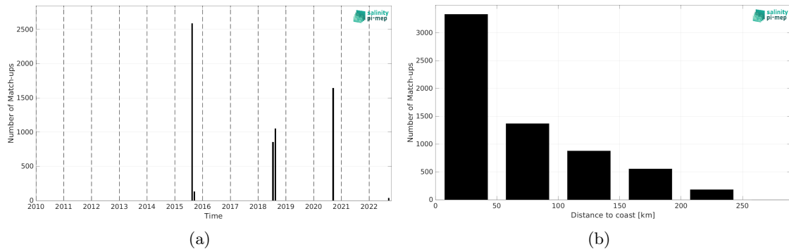
Figure 2: Number of match-ups between TSG (SAMOS) and SMAP SSS L2 v5.0 (JPL) SSS as a function of time (a) and as function of the distance to coast (b) over the Arctic Ocean Pi-MEP region and for the full satellite product period.
