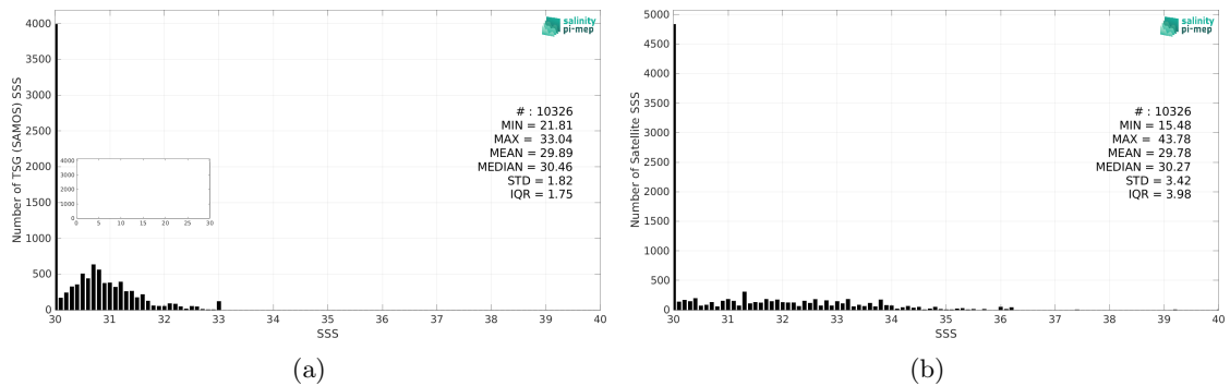
Figure 2: Histograms of SSS from TSG (SAMOS) (a) and SMAP SSS L2 v5.0 (JPL) (b) considering all match-up pairs per bins of 0.1 over the Arctic Ocean Pi-MEP region and for the full satellite product period.
