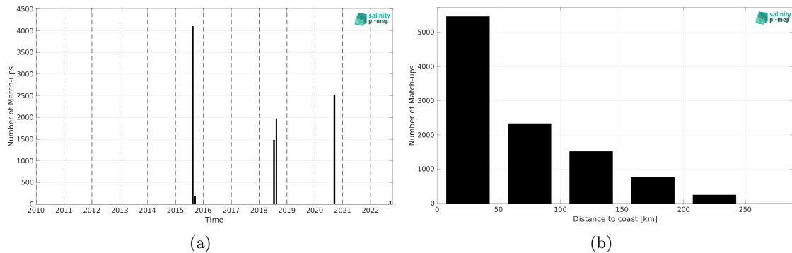
Figure 1: Number of match-ups between TSG (SAMOS) and SMAP SSS L2 v5.0 (JPL) SSS as a function of time (a) and as function of the distance to coast (b) over the Arctic Ocean Pi-MEP region and for the full satellite product period.
