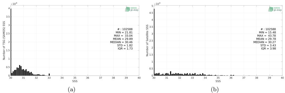
Figure 2: Histograms of SSS from TSG (SAMOS) (a) and SMAP SSS L2 v5.0 (JPL) (b) considering all match-up pairs per bins of 0.1 over the Arctic Ocean Pi-MEP region and for the full satellite product period.
