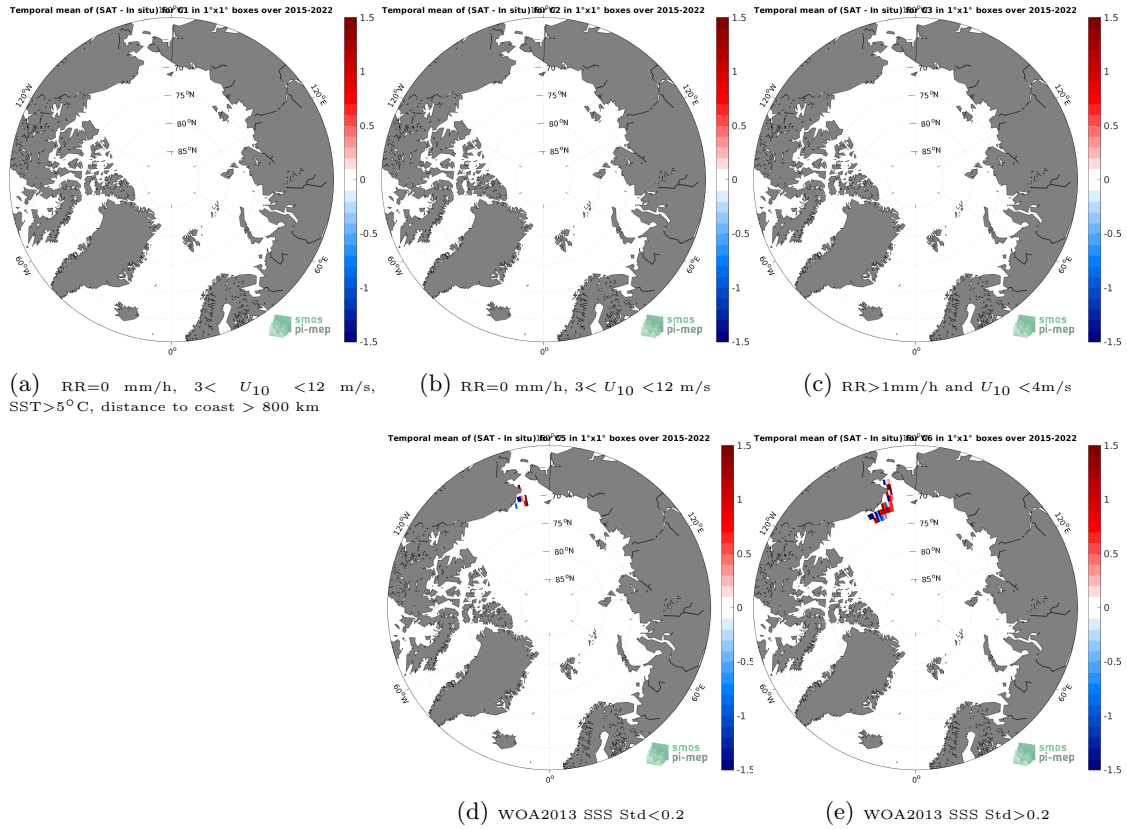
Figure 12: Temporal mean gridded over spatial boxes of size 1^{\circ}\times 1^{\circ} of \Delta\text{SSS} (SMAP SSS L2 v5.0 (JPL) - TSG (SAMOS)) for 5 different subdatasets corresponding to:RR=0 mm/h, 3 < U_{10} < 12 m/s, SST >5^{\circ}\text{C} , distance to coast > 800 km (a), RR=0 mm/h, 3 < U_{10} < 12 m/s (b), RR >1 mm/h and U_{10} < 4 m/s (c), WOA2013 SSS Std <0.2 (d), WOA2013 SSS Std >0.2 (e).
