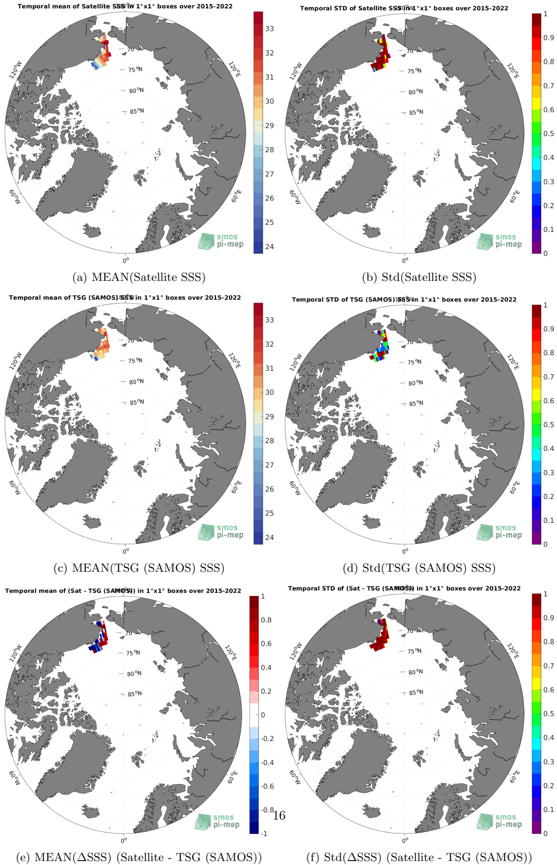
Figure 6: Temporal mean (left) and Std (right) of SSS from SMAP SSS L2 v5.0 (JPL) (top), TSG (SAMOS) (middle), and of \Delta SSS (Satellite - TSG (SAMOS)). Only match-up pairs are used to generate these maps.
