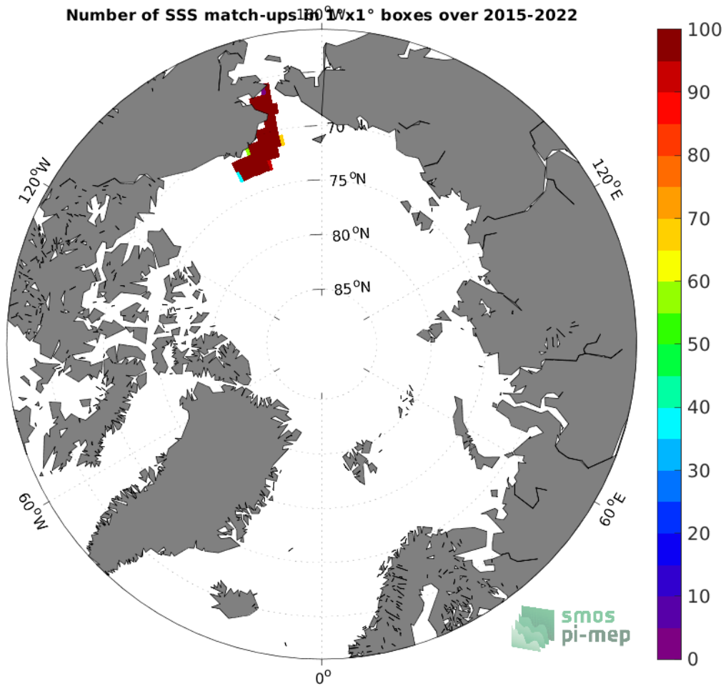
Figure 4: Number of SSS match-ups between TSG (SAMOS) SSS and the SMAP SSS L2 v5.0 (JPL) SSS product for the Arctic Ocean Pi-MEP region over 1^{\circ} \times 1^{\circ} boxes and for the full satellite product period.
