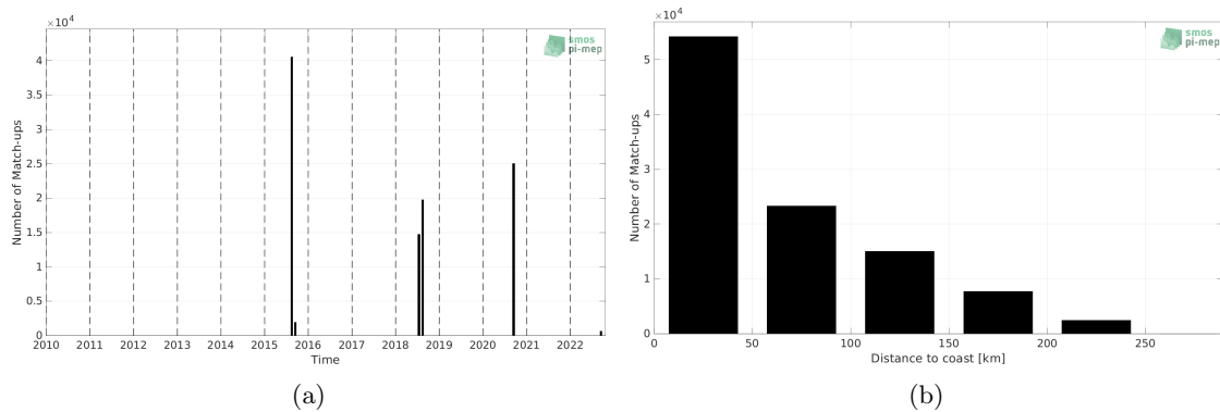
Figure 1: Number of match-ups between TSG (SAMOS) and SMAP SSS L2 v5.0 (JPL) SSS as a function of time (a) and as function of the distance to coast (b) over the Arctic Ocean Pi-MEP region and for the full satellite product period.
