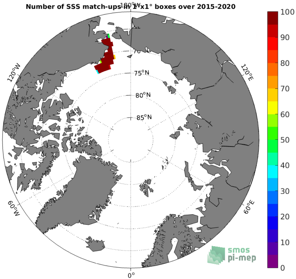
Figure 4: Number of SSS match-ups between TSG (SAMOS) SSS and the SMAP SSS L2 v5.0 (JPL) SSS product for the Arctic Ocean Pi-MEP region over 1^\circ \times 1^\circ boxes and for the full satellite product period.
