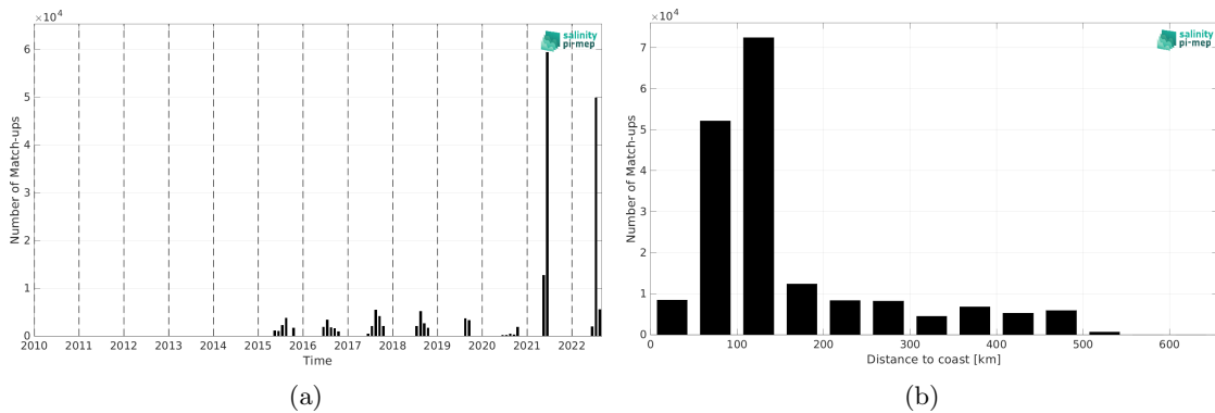
Figure 2: Number of match-ups between TSG (Polarstern) and SMAP SSS L2 v5.0 (JPL) SSS as a function of time (a) and as function of the distance to coast (b) over the Arctic Ocean Pi-MEP region and for the full satellite product period.
