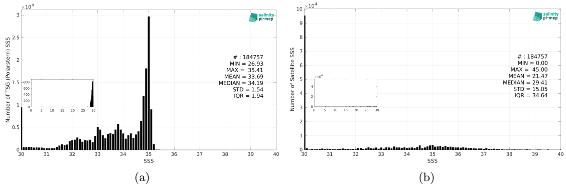
Figure 3: Histograms of SSS from TSG (Polarstern) (a) and SMAP SSS L2 v5.0 (JPL) (b) considering all match-up pairs per bins of 0.1 over the Arctic Ocean Pi-MEP region and for the full satellite product period.
