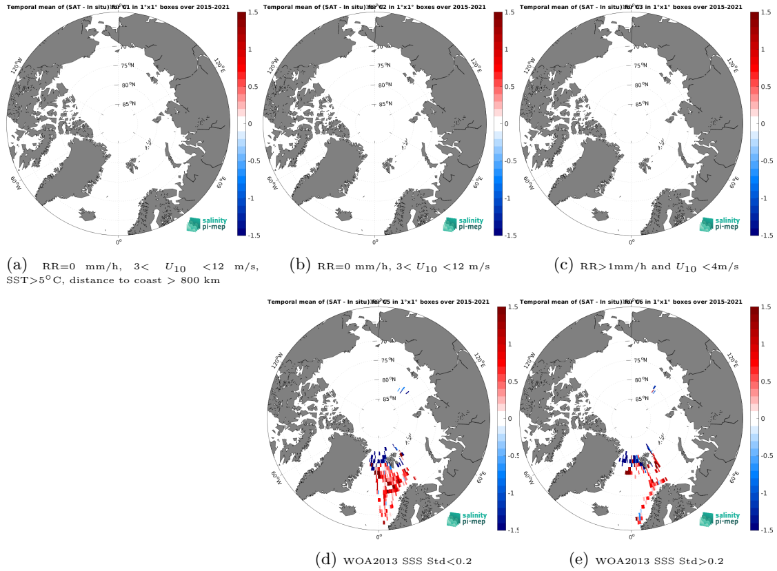
Figure 12: Temporal mean gridded over spatial boxes of size 1^{\circ}\times 1^{\circ} of \Delta\text{SSS} (SMAP SSS L2 v5.0 (JPL) - TSG (Polarstern)) for 5 different subdatasets corresponding to:RR=0 mm/h, 3 < U_{10} < 12 m/s, SST >5^{\circ}\text{C} , distance to coast > 800 km (a), RR=0 mm/h, 3 < U_{10} < 12 m/s (b), RR >1 mm/h and U_{10} < 4 m/s (c), WOA2013 SSS Std <0.2 (d), WOA2013 SSS Std >0.2 (e).
