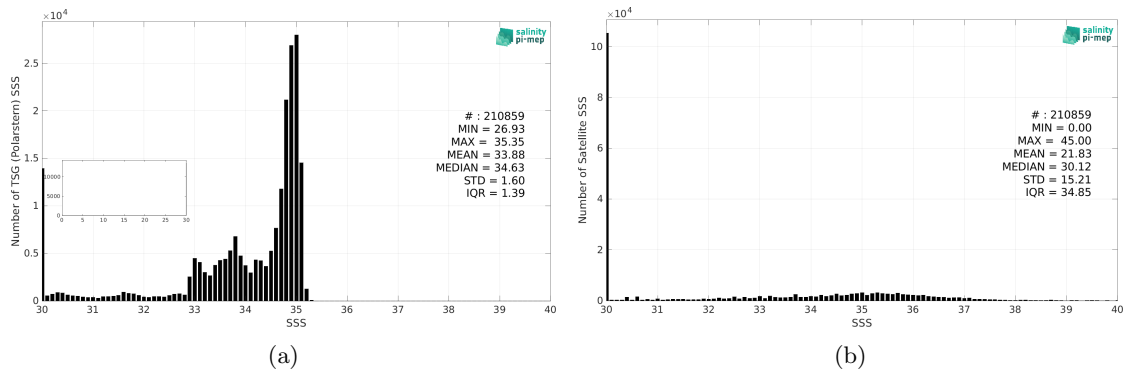
Figure 2: Histograms of SSS from TSG (Polarstern) (a) and SMAP SSS L2 v5.0 (JPL) (b) considering all match-up pairs per bins of 0.1 over the Arctic Ocean Pi-MEP region and for the full satellite product period.
