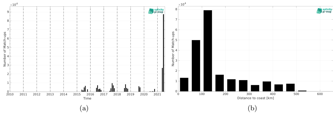
Figure 1: Number of match-ups between TSG (Polarstern) and SMAP SSS L2 v5.0 (JPL) SSS as a function of time (a) and as function of the distance to coast (b) over the Arctic Ocean Pi-MEP region and for the full satellite product period.
