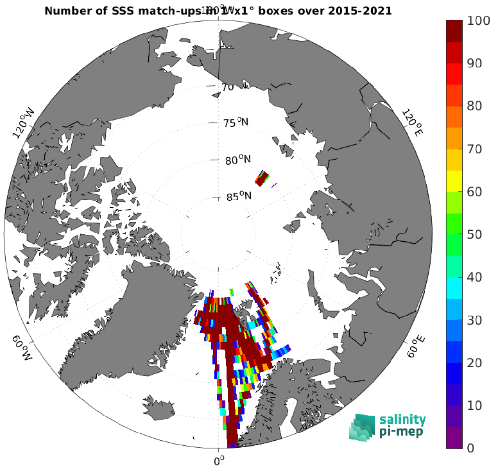
Figure 4: Number of SSS match-ups between TSG (Polarstern) SSS and the SMAP SSS L2 v5.0 (JPL) SSS product for the Arctic Ocean Pi-MEP region over 1^\circ \times 1^\circ boxes and for the full satellite product period.
