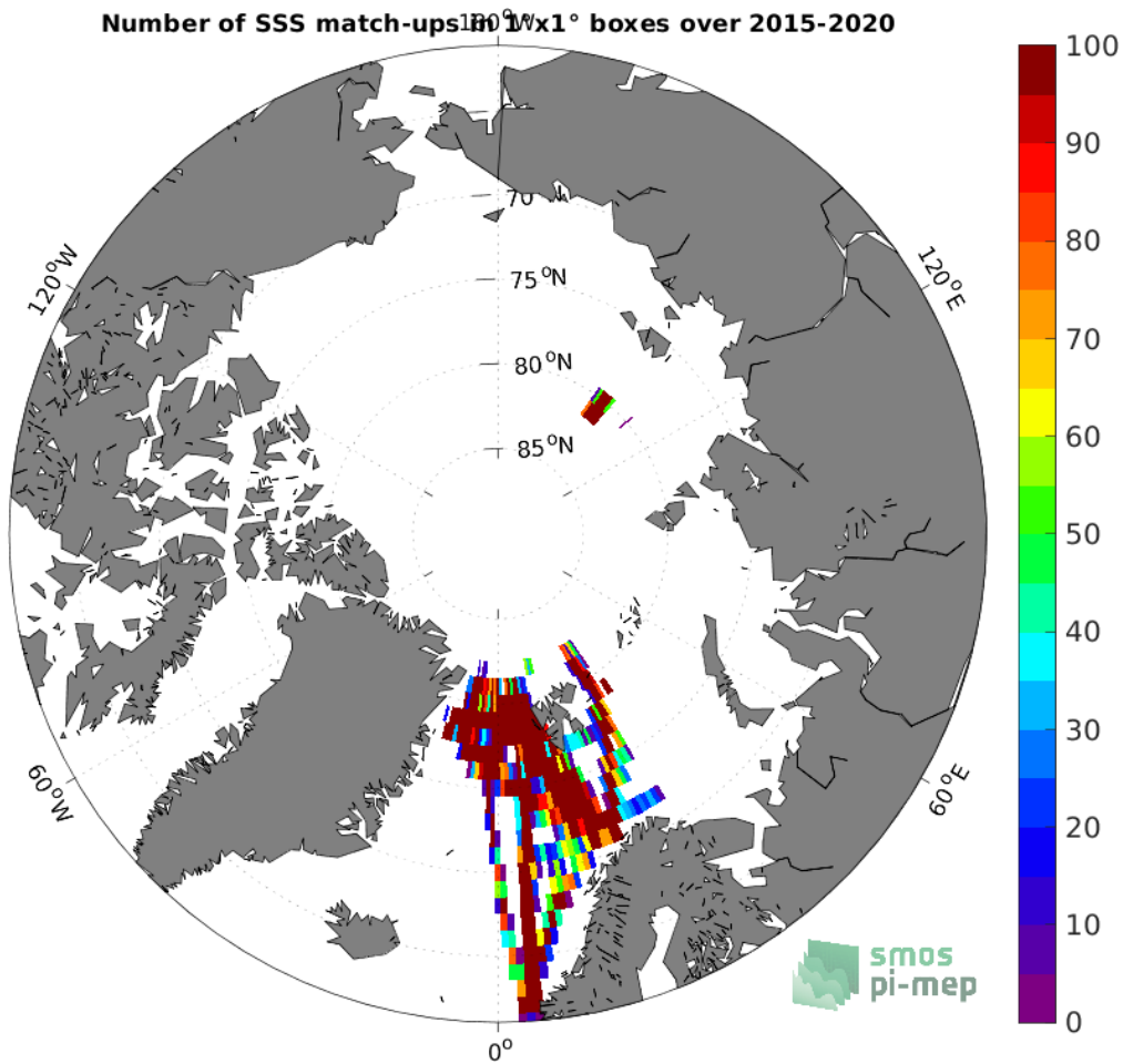
Figure 4: Number of SSS match-ups between TSG (Polarstern) SSS and the SMAP SSS L2 v5.0 (JPL) SSS product for the Arctic Ocean Pi-MEP region over 1^{\circ} \times 1^{\circ} boxes and for the full satellite product period.
