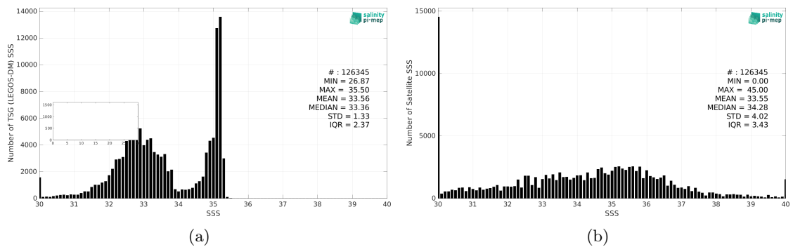
Figure 2: Histograms of SSS from TSG (LEGOS-DM) (a) and SMAP SSS L2 v5.0 (JPL) (b) considering all match-up pairs per bins of 0.1 over the Arctic Ocean Pi-MEP region and for the full satellite product period.
