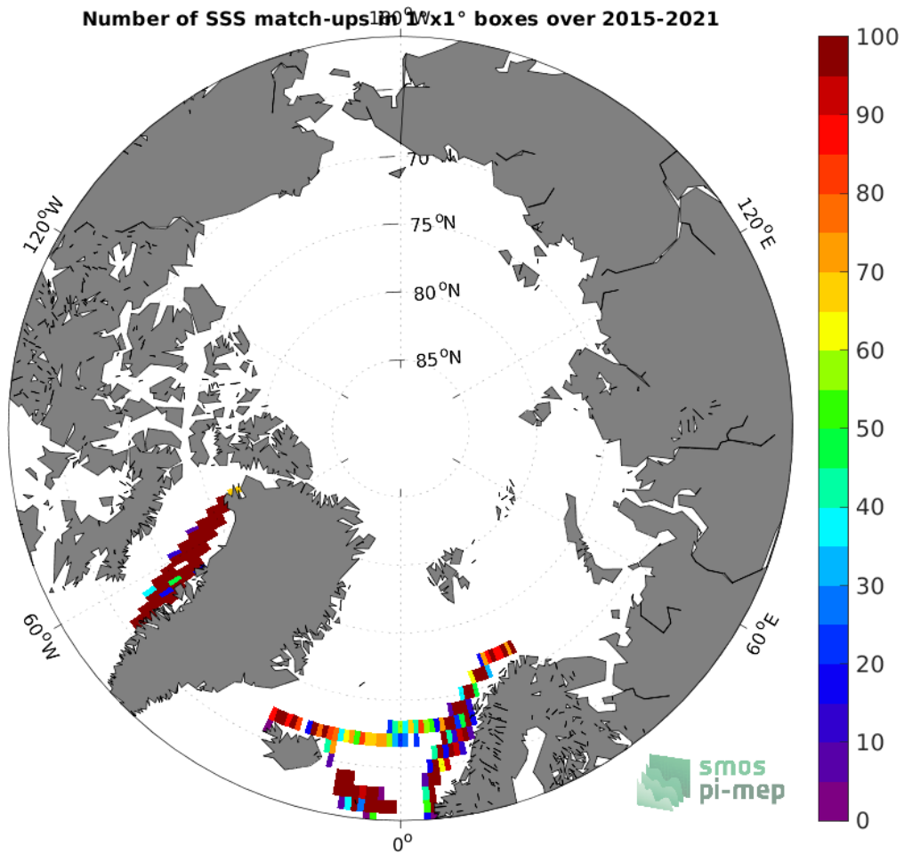
Figure 4: Number of SSS match-ups between TSG (LEGOS-DM) SSS and the SMAP SSS L2 v5.0 (JPL) SSS product for the Arctic Ocean Pi-MEP region over 1^{\circ} \times 1^{\circ} boxes and for the full satellite product period.
