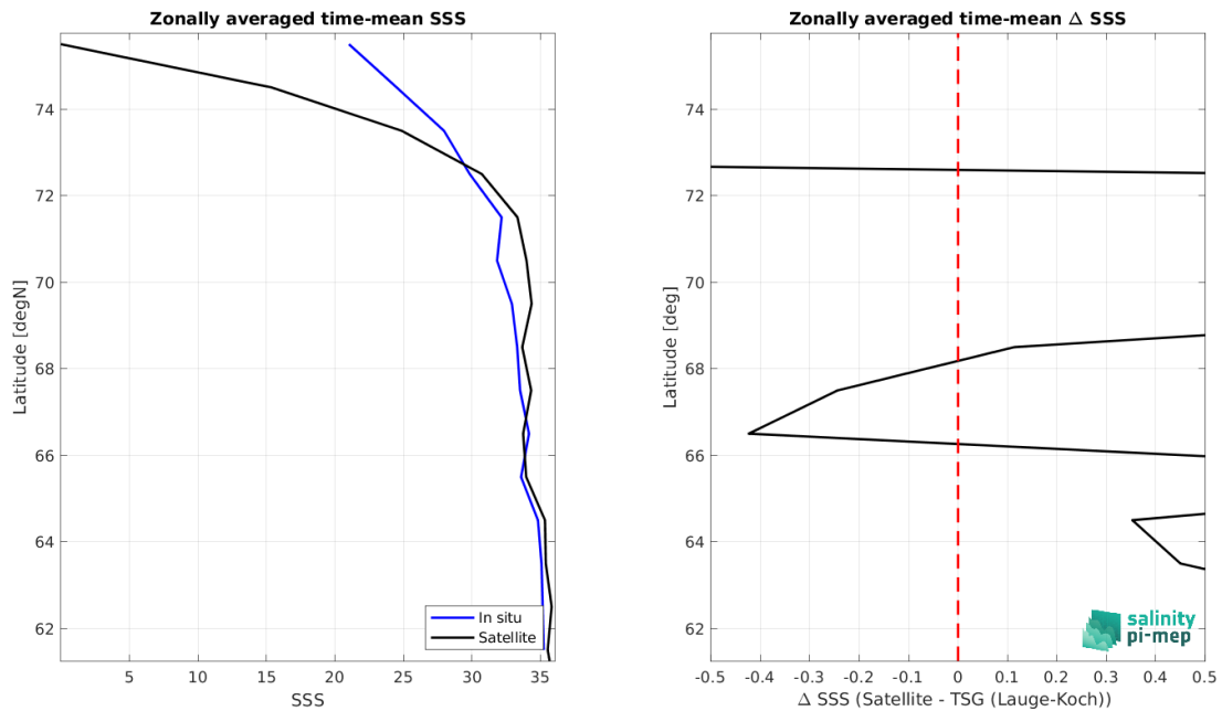
Figure 9: Left panel: Zonal mean SSS from SMAP SSS L2 v5.0 (JPL) satellite product (black) and from TSG (Lauge-Koch) (blue). Right panel: Zonal mean of \Delta SSS (Satellite - TSG (Lauge-Koch)) for all the collected Pi-MEP match-up pairs estimated over the full satellite product period.
