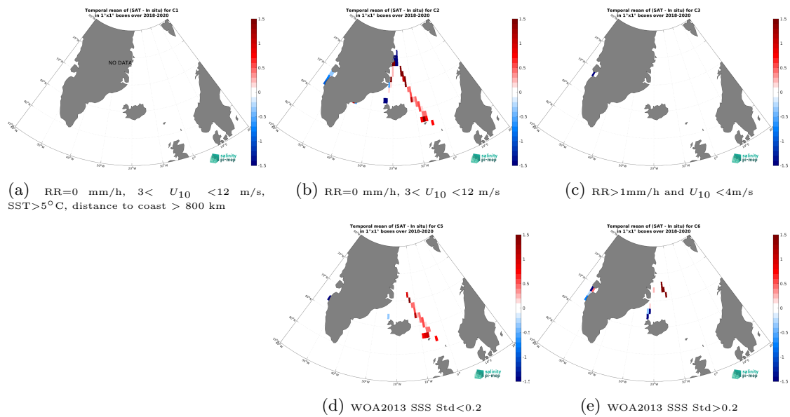
Figure 14: Temporal mean gridded over spatial boxes of size 1^\circ \times 1^\circ of \Delta SSS (SMAP SSS L2 v5.0 (JPL) - TSG (Lauge-Koch)) for 5 different subdatasets corresponding to:RR=0 mm/h, 3 < U_{10} < 12 m/s, SST > 5^\circ\text{C} , distance to coast > 800 km (a), RR=0 mm/h, 3 < U_{10} < 12 m/s (b), RR > 1 mm/h and U_{10} < 4 m/s (c), WOA2013 SSS Std < 0.2 (d), WOA2013 SSS Std > 0.2 (e).
