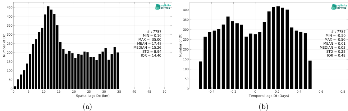
Figure 6: Histograms of the spatial (a) and temporal (b) lags between the location/time of the TSG (Lauge-Koch) measurement and the date of the corresponding SMAP SSS L2 v5.0 (JPL) SSS pixel.
