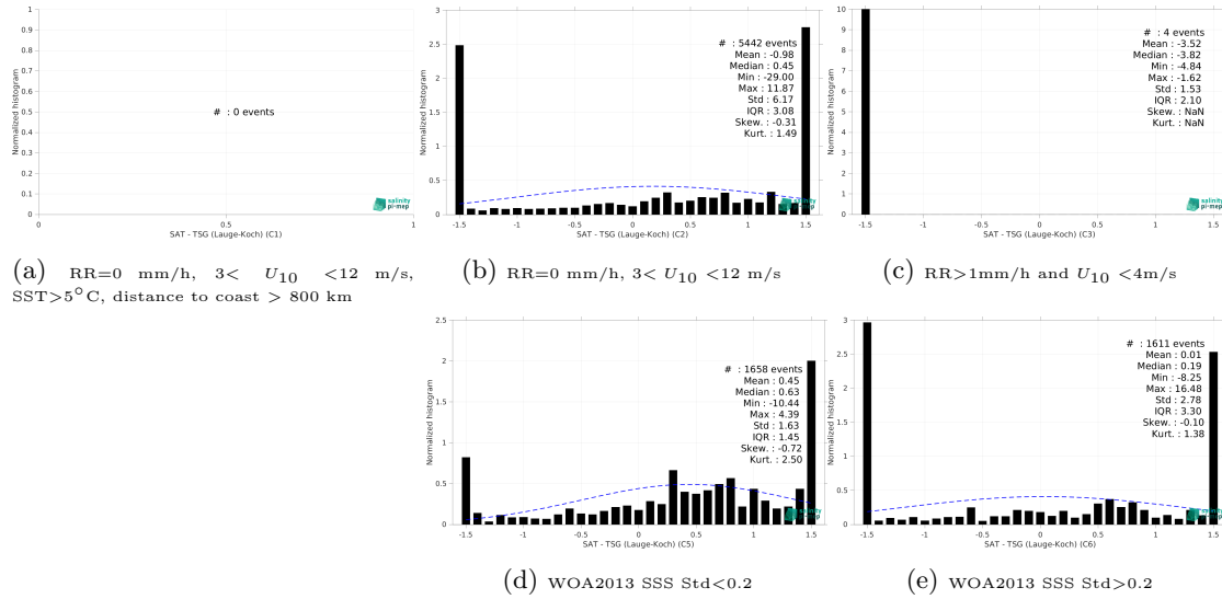
Figure 15: Normalized histogram of \Delta SSS (SMAP SSS L2 v5.0 (JPL) - TSG (Lauge-Koch)) for 5 different subdatasets corresponding to: RR=0 mm/h, 3 < U_{10} < 12 m/s, SST > 5°C, distance to coast > 800 km (a), RR=0 mm/h, 3 < U_{10} < 12 m/s (b), RR > 1mm/h and U_{10} < 4 m/s (c), WOA2013 SSS Std < 0.2 (d), WOA2013 SSS Std > 0.2 (e).
