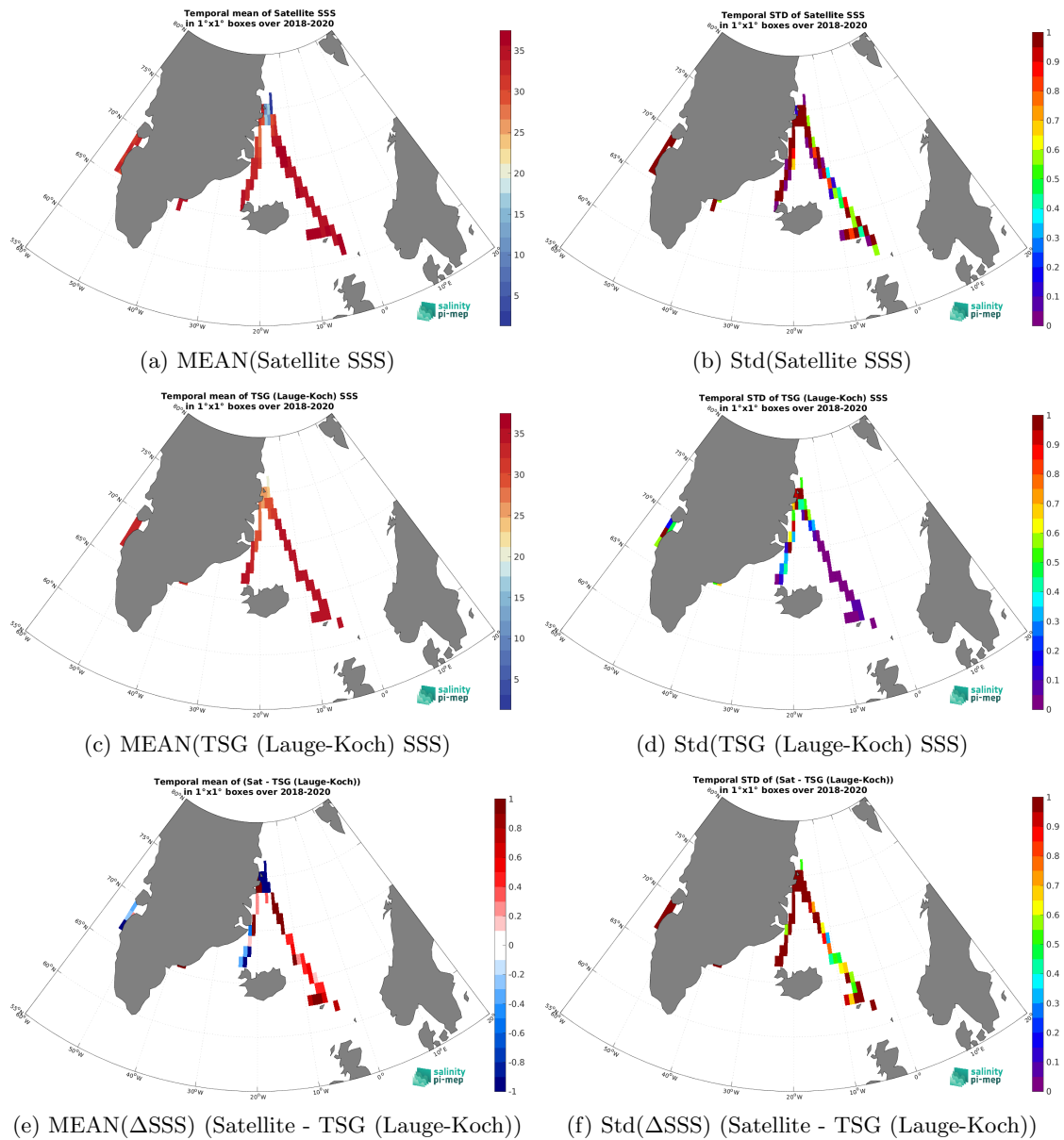
Figure 7: Temporal mean (left) and Std (right) of SSS from SMAP SSS L2 v5.0 (JPL) (top), TSG (Lauge-Koch) (middle), and of \Delta SSS (Satellite - TSG (Lauge-Koch)). Only match-up pairs are used to generate these maps.
