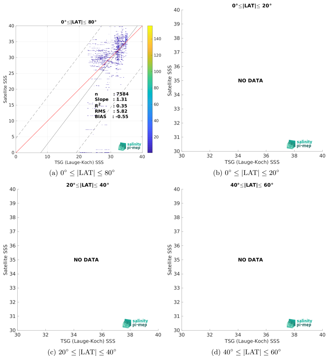
Figure 10: Contour maps of the concentration of SMAP SSS L2 v5.0 (JPL) SSS (y-axis) versus TSG (Lauge-Koch) SSS (x-axis) at match-up pairs for different latitude bands. For each plot, the red line shows x=y . The black thin and dashed lines indicate a linear fit through the data cloud and the \pm 95\% confidence levels, respectively. The number match-up pairs n , the slope and R^2 coefficient of the linear fit, the root mean square (RMS) and the mean bias between satellite and in situ data are indicated for each latitude band in each plots.
