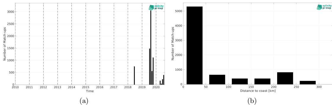
Figure 2: Number of match-ups between TSG (Lauge-Koch) and SMAP SSS L2 v5.0 (JPL) SSS as a function of time (a) and as function of the distance to coast (b) over the Arctic Ocean Pi-MEP region and for the full satellite product period.
