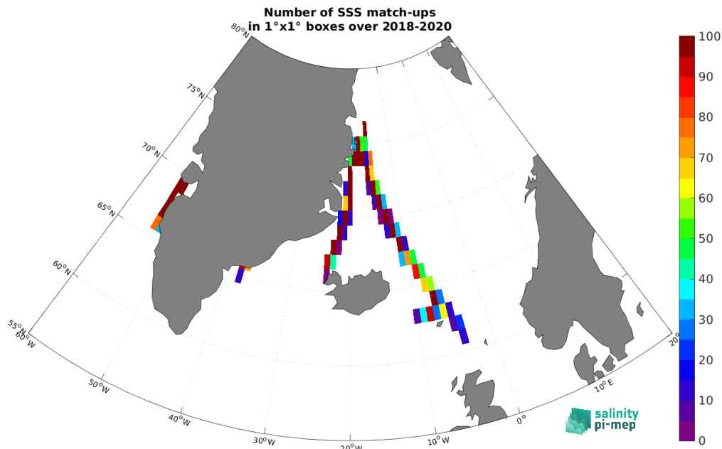
Figure 5: Number of SSS match-ups between TSG (Lauge-Koch) SSS and the SMAP SSS L2 v5.0 (JPL) SSS product for the Arctic Ocean Pi-MEP region over 1^\circ \times 1^\circ boxes and for the full satellite product period.
