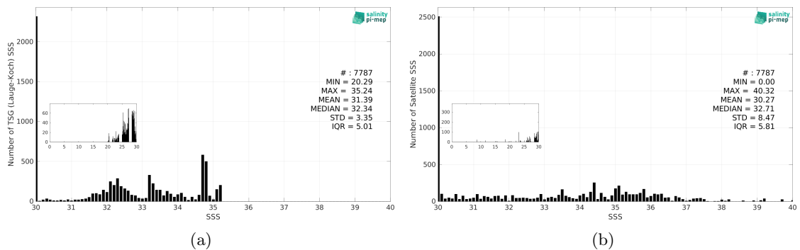
Figure 3: Histograms of SSS from TSG (Lauge-Koch) (a) and SMAP SSS L2 v5.0 (JPL) (b) considering all match-up pairs per bins of 0.1 over the Arctic Ocean Pi-MEP region and for the full satellite product period.
